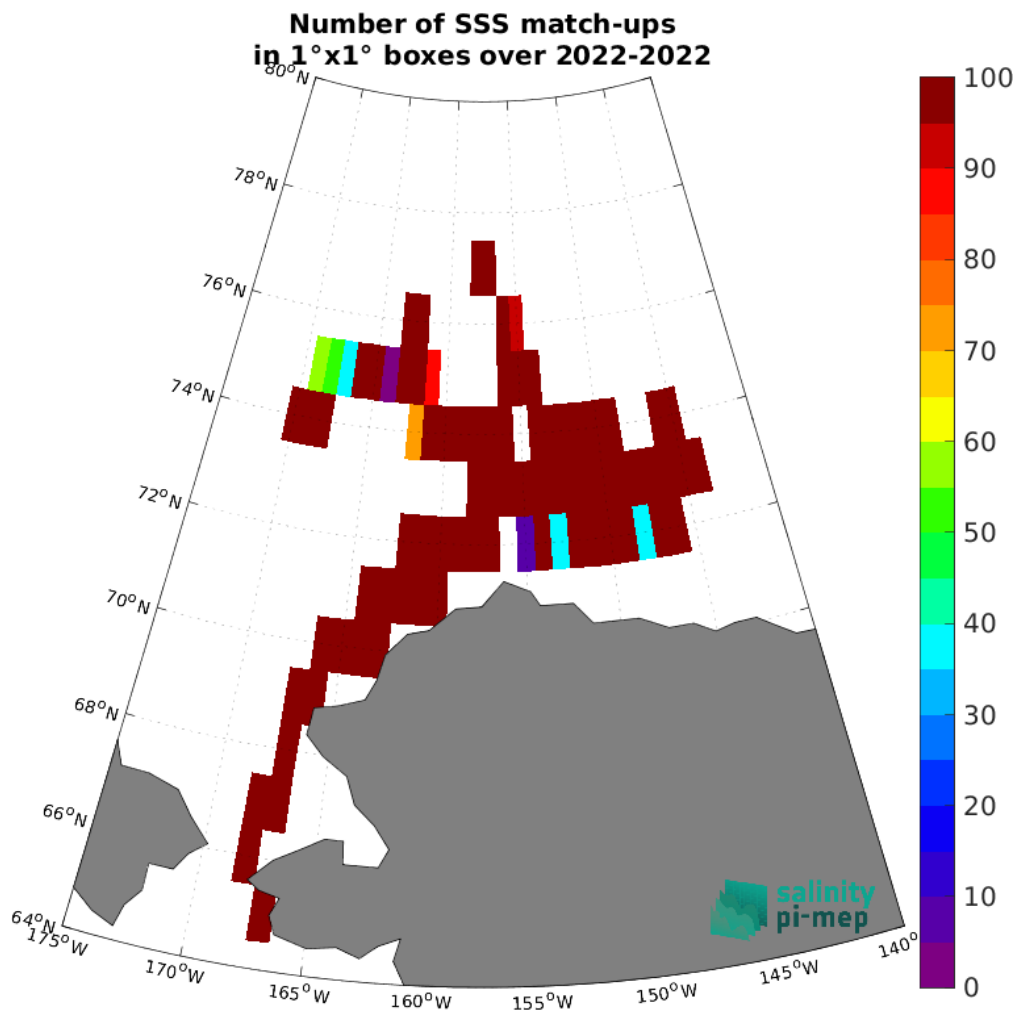
Figure 5: Number of SSS match-ups between SASSIE SSS and the SMAP SSS L4 OI v3 - Monthly (ESR) SSS product for the Global Ocean Pi-MEP region over 1^\circ \times 1^\circ boxes and for the full satellite product period.
