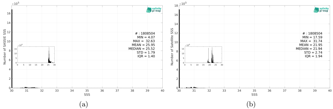
Figure 3: Histograms of SSS from SASSIE (a) and SMAP SSS L4 OI v3 - Monthly (ESR) (b) considering all match-up pairs per bins of 0.1 over the Global Ocean Pi-MEP region and for the full satellite product period.
