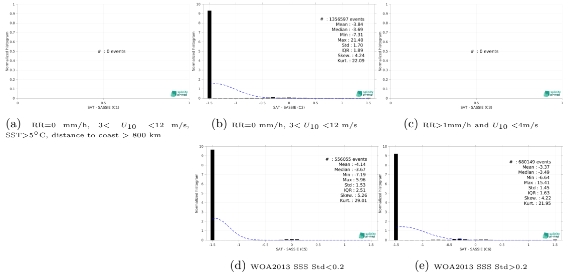
Figure 15: Normalized histogram of \Delta SSS (SMAP SSS L4 OI v3 - Monthly (ESR) - SASSIE) for 5 different subdatasets corresponding to: RR=0 mm/h, 3 < U_{10} < 12 m/s, SST > 5°C, distance to coast > 800 km (a), RR=0 mm/h, 3 < U_{10} < 12 m/s (b), RR > 1mm/h and U_{10} < 4 m/s (c), WOA2013 SSS Std < 0.2 (d), WOA2013 SSS Std > 0.2 (e).
