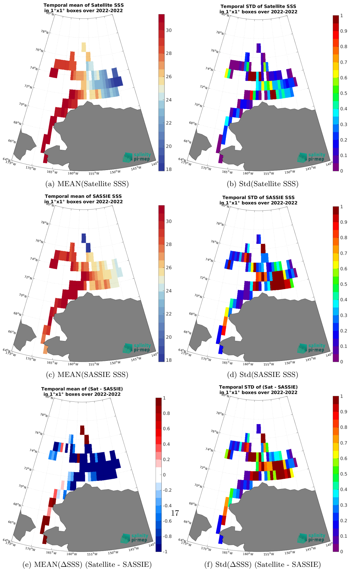
Figure 7: Temporal mean (left) and Std (right) of SSS from SMAP SSS L4 OI v3 - Monthly (ESR) (top), SASSIE (middle), and of \Delta SSS (Satellite - SASSIE). Only match-up pairs are used to generate these maps.
