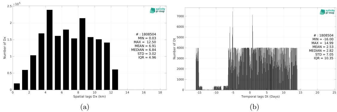
Figure 6: Histograms of the spatial (a) and temporal (b) lags between the location/time of the SASSIE measurement and the date of the corresponding SMAP SSS L4 OI v3 - Monthly (ESR) SSS pixel.
