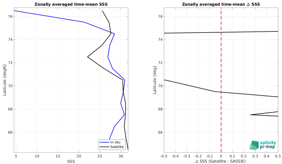
Figure 9: Left panel: Zonal mean SSS from SMAP SSS L4 OI v3 - Monthly (ESR) satellite product (black) and from SASSIE (blue). Right panel: Zonal mean of \Delta SSS (Satellite - SASSIE) for all the collected Pi-MEP match-up pairs estimated over the full satellite product period.
