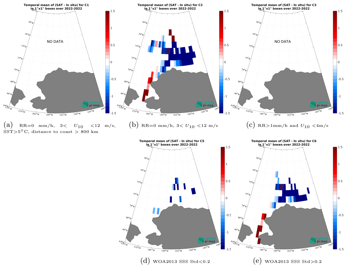
Figure 14: Temporal mean gridded over spatial boxes of size 1^\circ \times 1^\circ of \Delta SSS (SMAP SSS L4 OI v3 - Monthly (ESR) - SASSIE) for 5 different subdatasets corresponding to:RR=0 mm/h, 3 < U_{10} < 12 m/s, SST >5^\circ C, distance to coast > 800 km (a), RR=0 mm/h, 3 < U_{10} < 12 m/s (b), RR >1 mm/h and U_{10} < 4 m/s (c), WOA2013 SSS Std <0.2 (d), WOA2013 SSS Std >0.2 (e).
