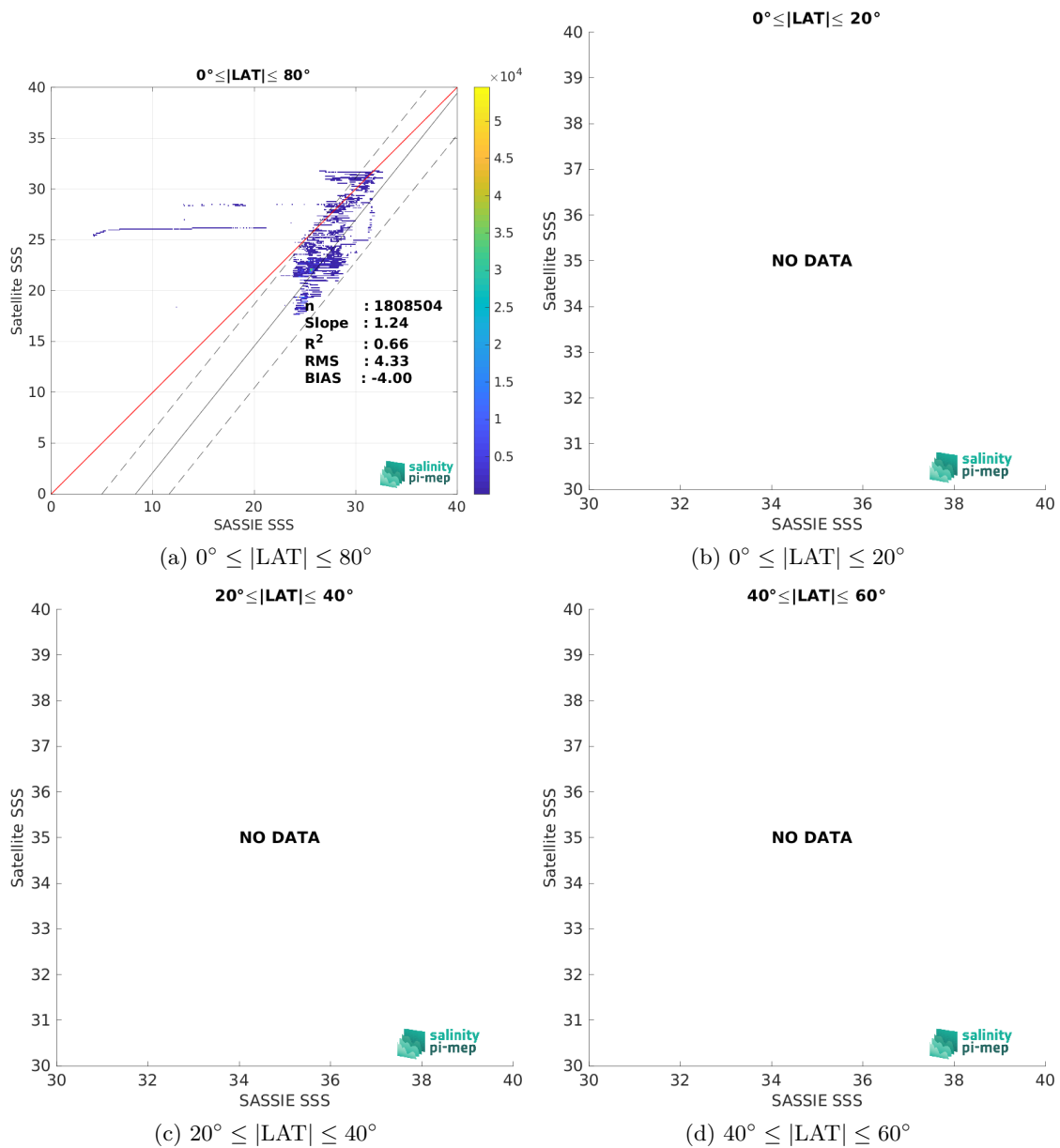
Figure 10: Contour maps of the concentration of SMAP SSS L4 OI v3 - Monthly (ESR) SSS (y-axis) versus SASSIE SSS (x-axis) at match-up pairs for different latitude bands. For each plot, the red line shows x=y . The black thin and dashed lines indicate a linear fit through the data cloud and the \pm 95\% confidence levels, respectively. The number match-up pairs n , the slope and R^2 coefficient of the linear fit, the root mean square (RMS) and the mean bias between satellite and in situ data are indicated for each latitude band in each plots.
