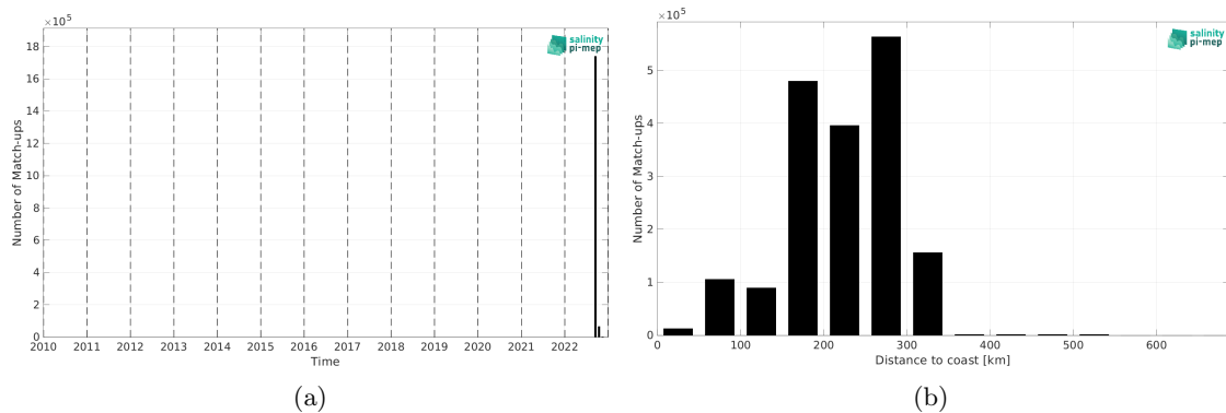
Figure 2: Number of match-ups between SASSIE and SMAP SSS L4 OI v3 - Monthly (ESR) SSS as a function of time (a) and as function of the distance to coast (b) over the Global Ocean Pi-MEP region and for the full satellite product period.
