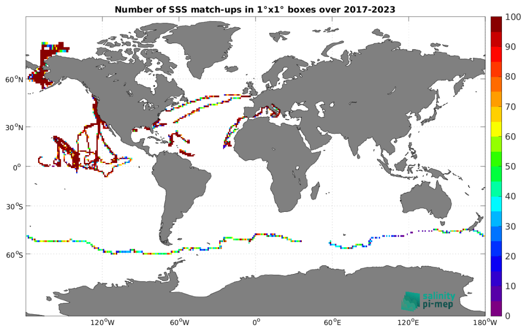
Figure 5: Number of SSS match-ups between Saildrone SSS and the SMAP SSS L4 OI v3 - Monthly (ESR) SSS product for the Global Ocean Pi-MEP region over 1^\circ \times 1^\circ boxes and for the full satellite product period.
