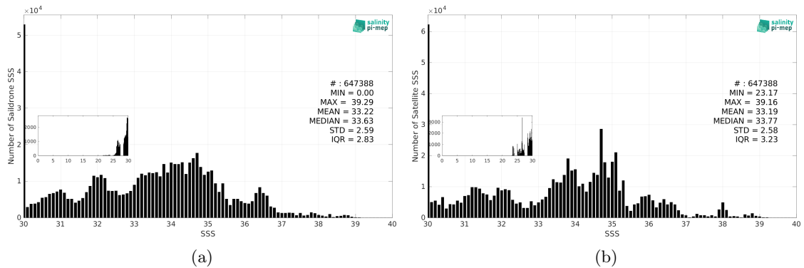
Figure 3: Histograms of SSS from Saïdrone (a) and SMAP SSS L4 OI v3 - Monthly (ESR) (b) considering all match-up pairs per bins of 0.1 over the Global Ocean Pi-MEP region and for the full satellite product period.
