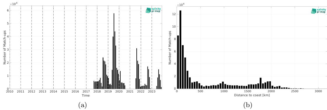
Figure 2: Number of match-ups between Saïdrone and SMAP SSS L4 OI v3 - Monthly (ESR) SSS as a function of time (a) and as function of the distance to coast (b) over the Global Ocean Pi-MEP region and for the full satellite product period.
