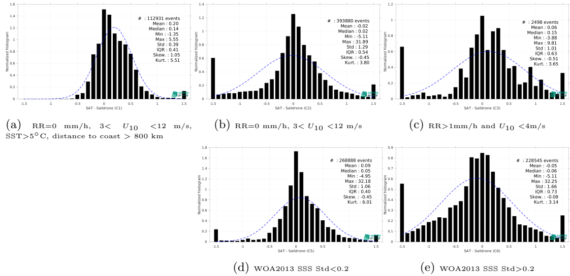
Figure 15: Normalized histogram of \Delta SSS (SMAP SSS L4 OI v3 - Monthly (ESR) - Sairdronne) for 5 different subdatasets corresponding to: RR=0 mm/h, 3 < U_{10} < 12 m/s, SST > 5°C, distance to coast > 800 km (a), RR=0 mm/h, 3 < U_{10} < 12 m/s (b), RR > 1mm/h and U_{10} < 4 m/s (c), WOA2013 SSS Std < 0.2 (d), WOA2013 SSS Std > 0.2 (e).
