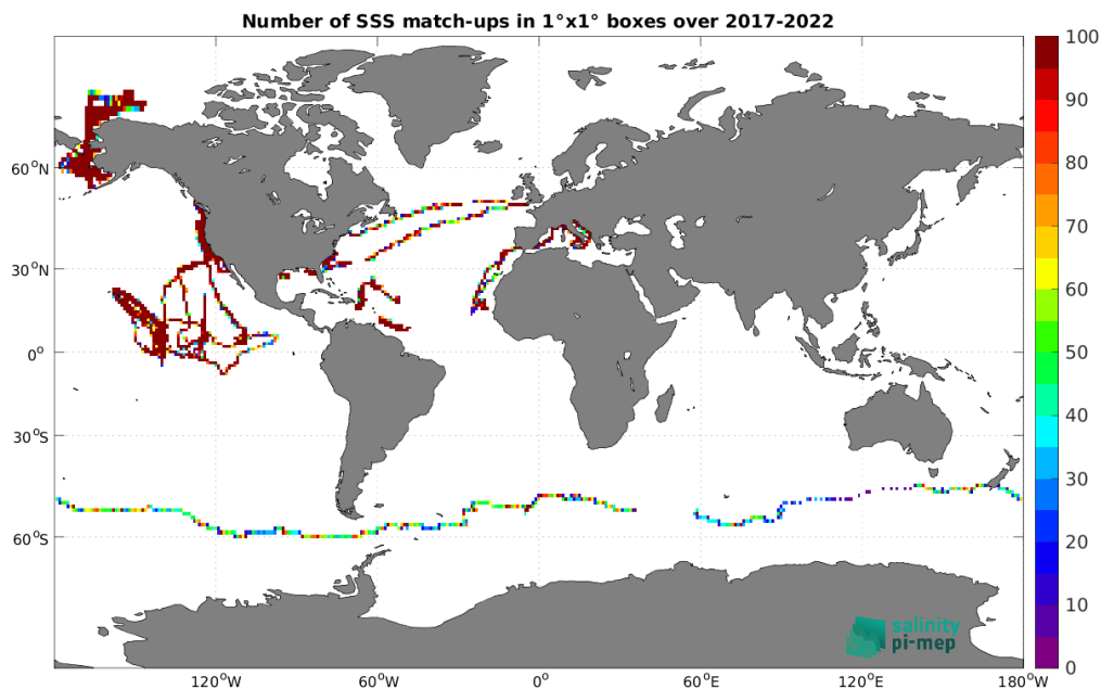
Figure 5: Number of SSS match-ups between Salldrone SSS and the SMAP SSS L4 OI v3 - Monthly (ESR) SSS product for the Global Ocean Pi-MEP region over 1^\circ \times 1^\circ boxes and for the full satellite product period.
