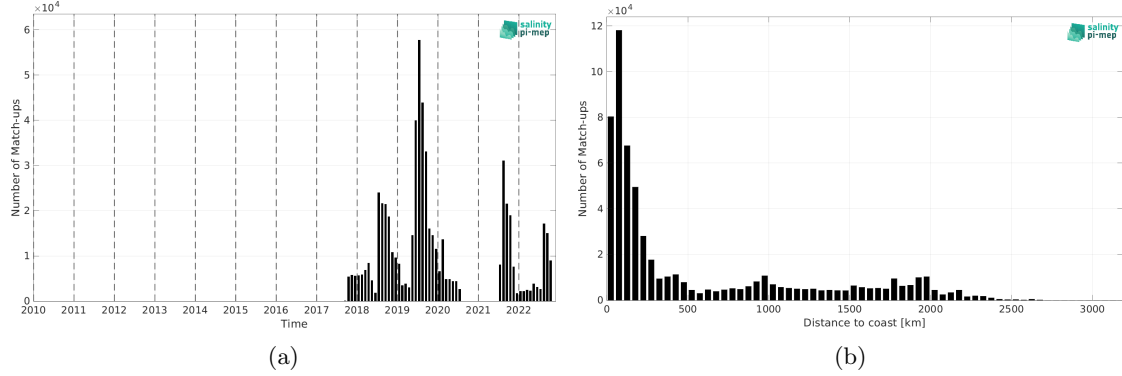
Figure 2: Number of match-ups between Sailldrone and SMAP SSS L4 OI v3 - Monthly (ESR) SSS as a function of time (a) and as function of the distance to coast (b) over the Global Ocean Pi-MEP region and for the full satellite product period.
