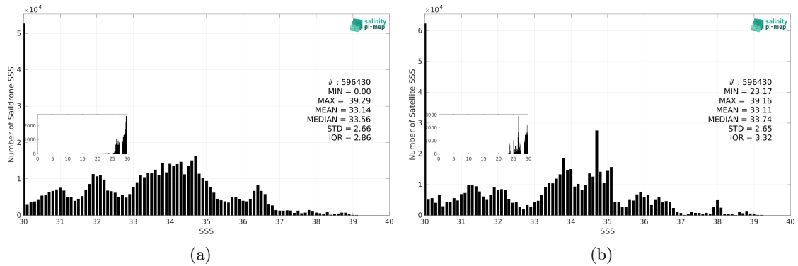
Figure 3: Histograms of SSS from Sailldrone (a) and SMAP SSS L4 OI v3 - Monthly (ESR) (b) considering all match-up pairs per bins of 0.1 over the Global Ocean Pi-MEP region and for the full satellite product period.
