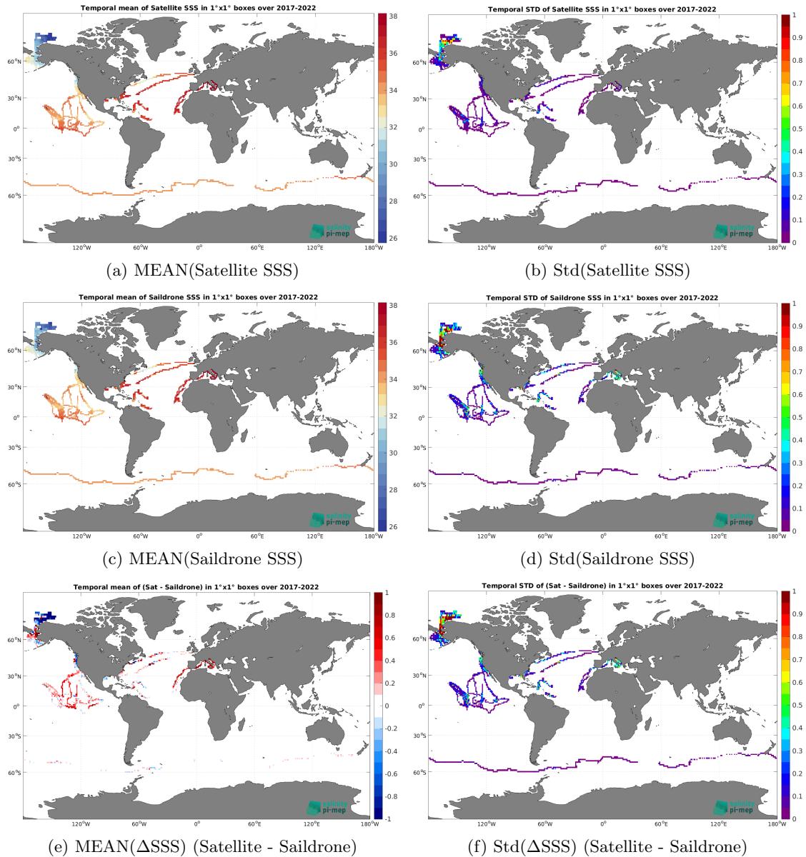
Figure 7: Temporal mean (left) and Std (right) of SSS from SMAP SSS L4 OI v3 - Monthly (ESR) (top), Saildrone (middle), and of \Delta SSS (Satellite - Saildrone). Only match-up pairs are used to generate these maps.
