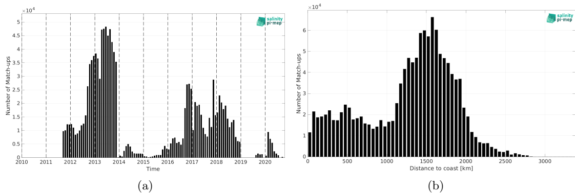
Figure 2: Number of match-ups between Surface drifters and SMAP SSS L4 OI v3 - Monthly (ESR) SSS as a function of time (a) and as function of the distance to coast (b) over the Global Ocean Pi-MEP region and for the full satellite product period.
