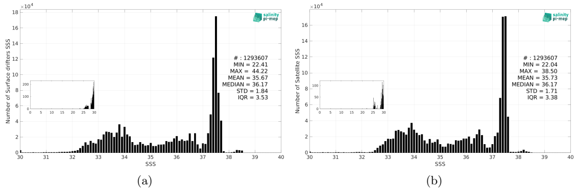
Figure 3: Histograms of SSS from Surface drifters (a) and SMAP SSS L4 OI v3 - Monthly (ESR) (b) considering all match-up pairs per bins of 0.1 over the Global Ocean Pi-MEP region and for the full satellite product period.
