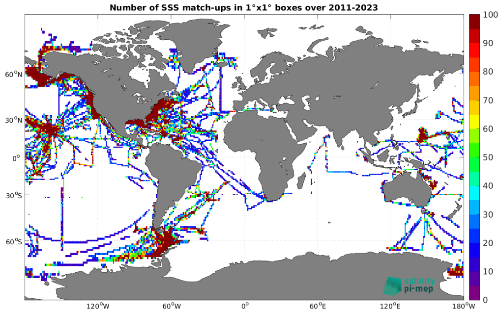
Figure 5: Number of SSS match-ups between TSG (SAMOS) SSS and the SMAP SSS L4 OI v3 - Daily (ESR) SSS product for the Global Ocean Pi-MEP region over 1^\circ \times 1^\circ boxes and for the full satellite product period.
