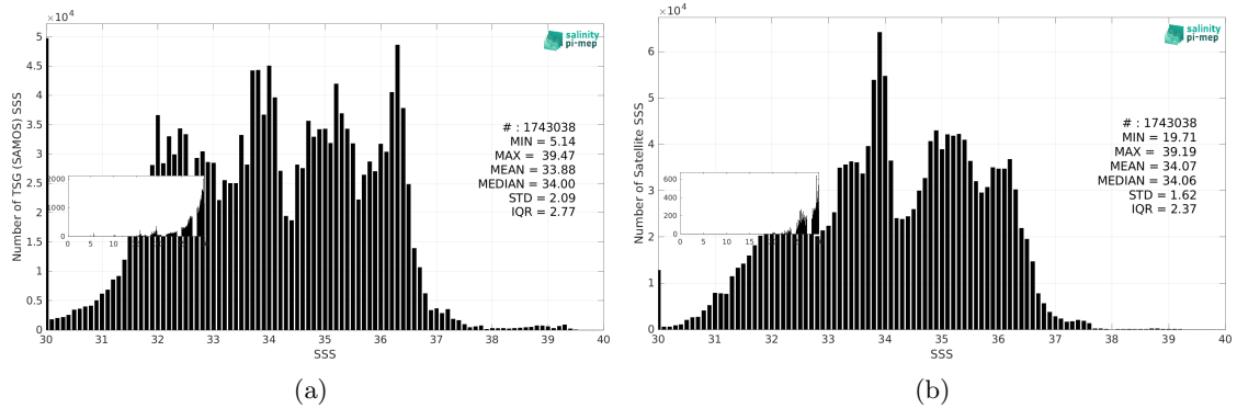
Figure 3: Histograms of SSS from TSG (SAMOS) (a) and SMAP SSS L4 OI v3 - Daily (ESR) (b) considering all match-up pairs per bins of 0.1 over the Global Ocean Pi-MEP region and for the full satellite product period.
