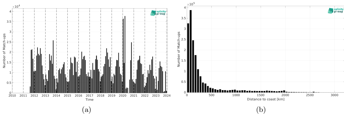
Figure 2: Number of match-ups between TSG (SAMOS) and SMAP SSS L4 OI v3 - Daily (ESR) SSS as a function of time (a) and as function of the distance to coast (b) over the Global Ocean Pi-MEP region and for the full satellite product period.
