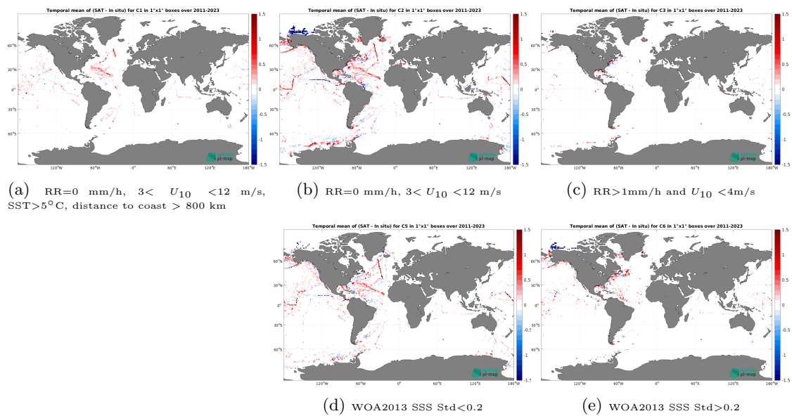
Figure 14: Temporal mean gridded over spatial boxes of size 1^\circ \times 1^\circ of \Delta\text{SSS} (SMAP SSS L4 OI v3 - Daily (ESR) - TSG (SAMOS)) for 5 different subdatasets corresponding to:RR=0 mm/h, 3 < U_{10} < 12 m/s, SST >5^\circ\text{C} , distance to coast > 800 km (a), RR=0 mm/h, 3 < U_{10} < 12 m/s (b), RR >1 mm/h and U_{10} < 4 m/s (c), WOA2013 SSS Std <0.2 (d), WOA2013 SSS Std >0.2 (e).
