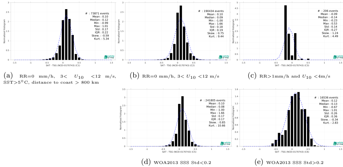
Figure 15: Normalized histogram of \Delta SSS (SMAP SSS L4 OI v3 - Daily (ESR) - TSG (NCEI-0170743)) for 5 different subdatasets corresponding to: RR=0 mm/h, 3 < U_{10} < 12 m/s, SST>5°C, distance to coast > 800 km (a), RR=0 mm/h, 3 < U_{10} < 12 m/s (b), RR>1mm/h and U_{10} < 4 m/s (c), WOA2013 SSS Std<0.2 (d), WOA2013 SSS Std>0.2 (e).
