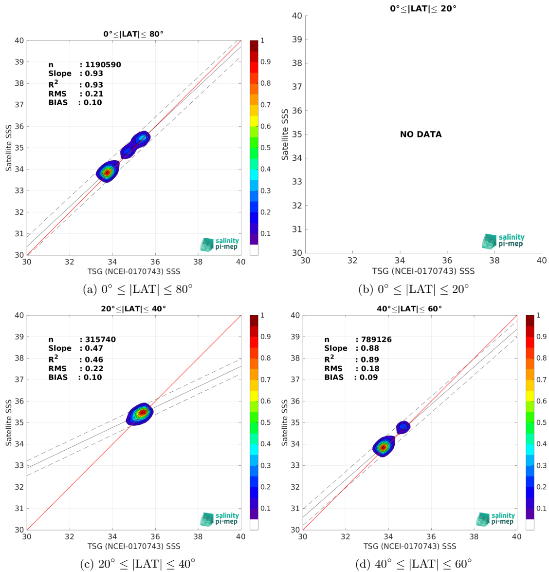
Figure 10: Contour maps of the concentration of SMAP SSS L4 OI v3 - Daily (ESR) SSS (y-axis) versus TSG (NCEI-0170743) SSS (x-axis) at match-up pairs for different latitude bands. For each plot, the red line shows x=y . The black thin and dashed lines indicate a linear fit through the data cloud and the \pm 95\% confidence levels, respectively. The number match-up pairs n , the slope and R^2 coefficient of the linear fit, the root mean square (RMS) and the mean bias between satellite and in situ data are indicated for each latitude band in each plots.
