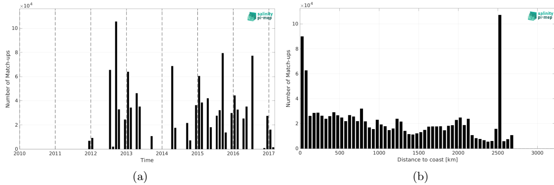
Figure 2: Number of match-ups between TSG (NCEI-0170743) and SMAP SSS L4 OI v3 - Daily (ESR) SSS as a function of time (a) and as function of the distance to coast (b) over the Global Ocean Pi-MEP region and for the full satellite product period.
