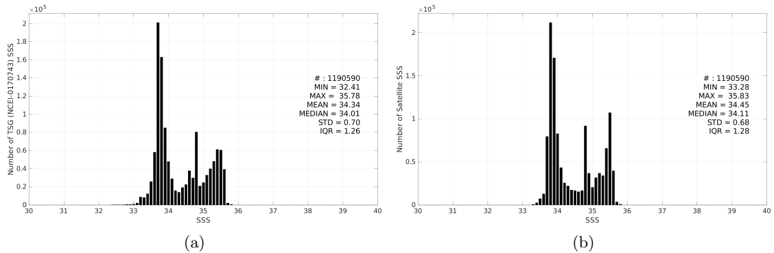
Figure 3: Histograms of SSS from TSG (NCEI-0170743) (a) and SMAP SSS L4 OI v3 - Daily (ESR) (b) considering all match-up pairs per bins of 0.1 over the Global Ocean Pi-MEP region and for the full satellite product period.
