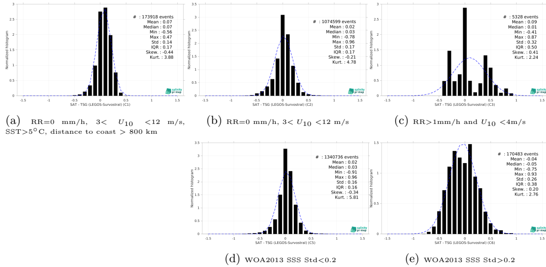
Figure 15: Normalized histogram of \Delta SSS (SMAP SSS L4 OI v3 - Daily (ESR) - TSG (LEGOS-Survostral)) for 5 different subdatasets corresponding to: RR=0 mm/h, 3 < U_{10} < 12 m/s, SST>5°C, distance to coast > 800 km (a), RR=0 mm/h, 3 < U_{10} < 12 m/s (b), RR>1mm/h and U_{10} < 4 m/s (c), WOA2013 SSS Std<0.2 (d), WOA2013 SSS Std>0.2 (e).
