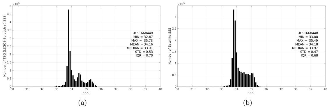
Figure 3: Histograms of SSS from TSG (LEGOS-Survostral) (a) and SMAP SSS L4 OI v3 - Daily (ESR) (b) considering all match-up pairs per bins of 0.1 over the Global Ocean Pi-MEP region and for the full satellite product period.
