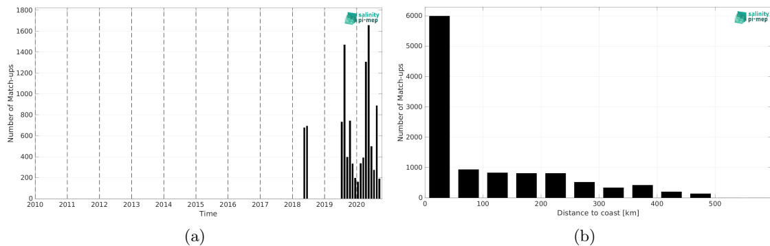
Figure 2: Number of match-ups between TSG (Lauge-Koch) and SMAP SSS L4 OI v3 - Daily (ESR) SSS as a function of time (a) and as function of the distance to coast (b) over the Global Ocean Pi-MEP region and for the full satellite product period.
