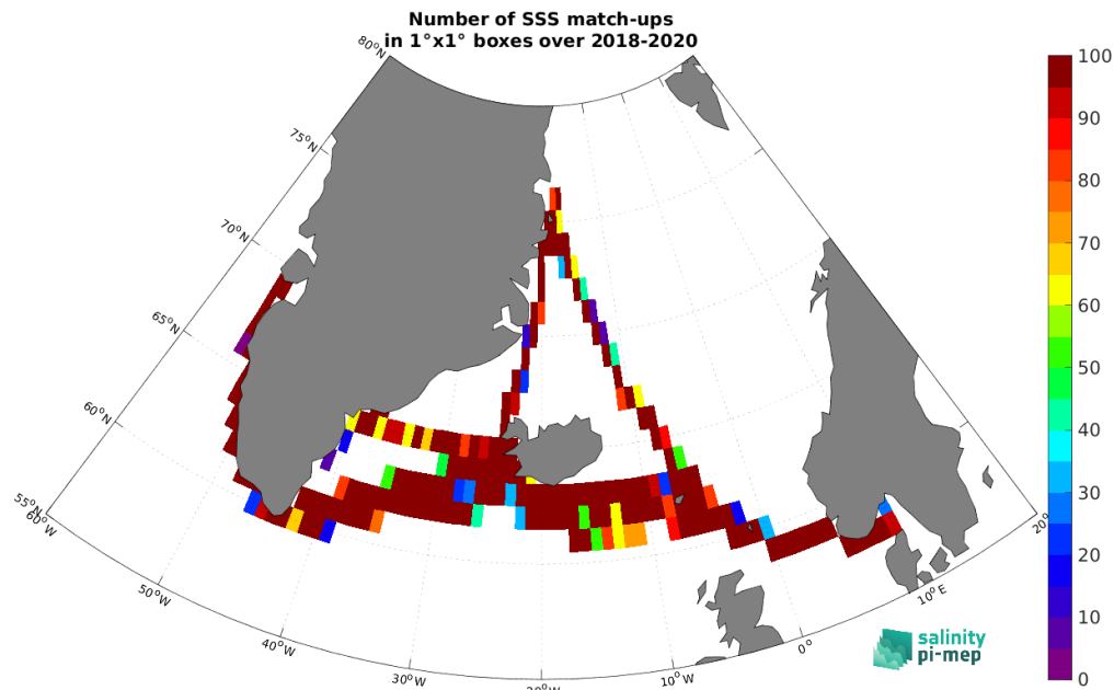
Figure 5: Number of SSS match-ups between TSG (Lauge-Koch) SSS and the SMAP SSS L4 OI v3 - Daily (ESR) SSS product for the Global Ocean Pi-MEP region over 1^\circ \times 1^\circ boxes and for the full satellite product period.
