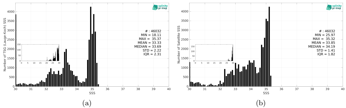
Figure 3: Histograms of SSS from TSG (Lauge-Koch) (a) and SMAP SSS L4 OI v3 - Daily (ESR) (b) considering all match-up pairs per bins of 0.1 over the Global Ocean Pi-MEP region and for the full satellite product period.
