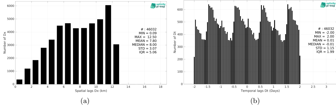
Figure 6: Histograms of the spatial (a) and temporal (b) lags between the location/time of the TSG (Lauge-Koch) measurement and the date of the corresponding SMAP SSS L4 OI v3 - Daily (ESR) SSS pixel.
