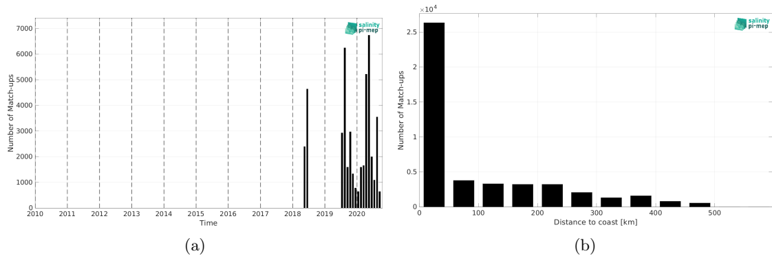
Figure 2: Number of match-ups between TSG (Lauge-Koch) and SMAP SSS L4 OI v3 - Daily (ESR) SSS as a function of time (a) and as function of the distance to coast (b) over the Global Ocean Pi-MEP region and for the full satellite product period.
