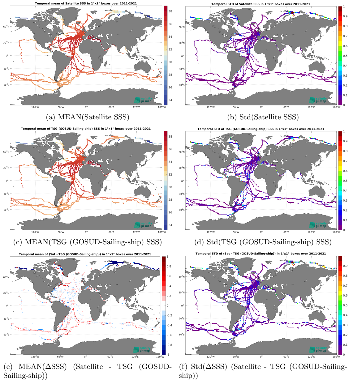
Figure 7: Temporal mean (left) and Std (right) of SSS from SMAP SSS L4 OI v3 - Daily (ESR) (top), TSG (GOSUD-Sailing-ship) (middle), and of \Delta SSS (Satellite - TSG (GOSUD-Sailing-ship)). Only match-up pairs are used to generate these maps.
