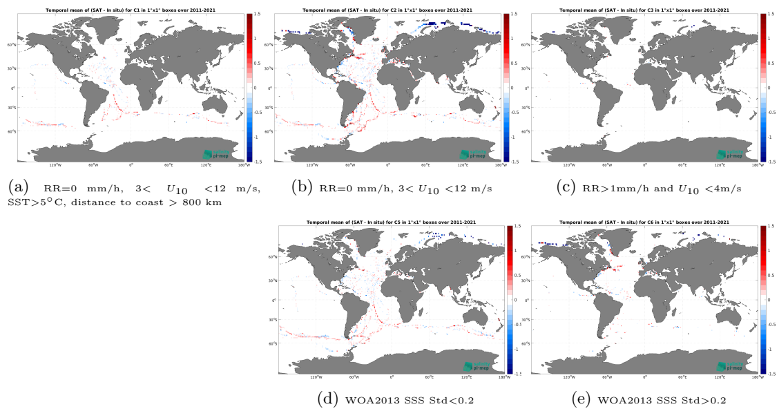
Figure 14: Temporal mean gridded over spatial boxes of size 1^\circ \times 1^\circ of \Delta SSS (SMAP SSS L4 OI v3 - Daily (ESR) - TSG (GOSUD-Sailing-ship)) for 5 different subdatasets corresponding to:RR=0 mm/h, 3 < U_{10} < 12 m/s, SST > 5^\circ\text{C} , distance to coast > 800 km (a), RR=0 mm/h, 3 < U_{10} < 12 m/s (b), RR > 1 mm/h and U_{10} < 4 m/s (c), WOA2013 SSS Std < 0.2 (d), WOA2013 SSS Std > 0.2 (e).
