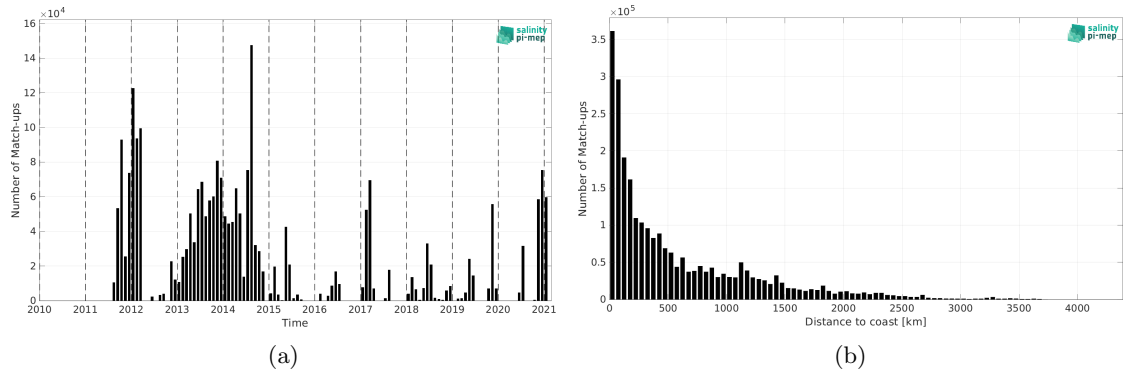
Figure 2: Number of match-ups between TSG (GOSUD-Sailing-ship) and SMAP SSS L4 OI v3 - Daily (ESR) SSS as a function of time (a) and as function of the distance to coast (b) over the Global Ocean Pi-MEP region and for the full satellite product period.
