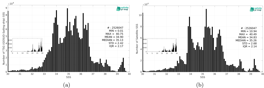
Figure 3: Histograms of SSS from TSG (GOSUD-Sailing-ship) (a) and SMAP SSS L4 OI v3 - Daily (ESR) (b) considering all match-up pairs per bins of 0.1 over the Global Ocean Pi-MEP region and for the full satellite product period.
