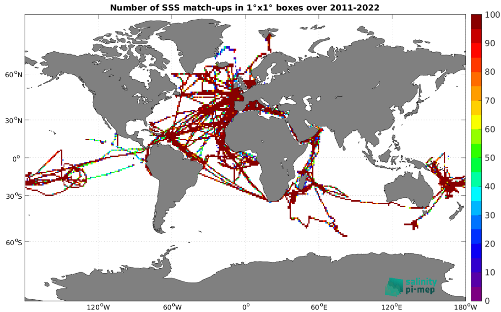
Figure 5: Number of SSS match-ups between TSG (GOSUD-Research-vessel) SSS and the SMAP SSS L4 OI v3 - Daily (ESR) SSS product for the Global Ocean Pi-MEP region over 1^\circ \times 1^\circ boxes and for the full satellite product period.
