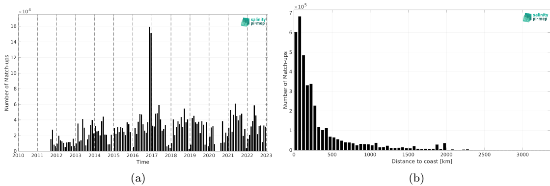
Figure 2: Number of match-ups between TSG (GOSUD-Research-vessel) and SMAP SSS L4 OI v3 - Daily (ESR) SSS as a function of time (a) and as function of the distance to coast (b) over the Global Ocean Pi-MEP region and for the full satellite product period.
