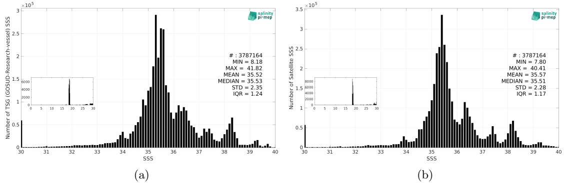
Figure 3: Histograms of SSS from TSG (GOSUD-Research-vessel) (a) and SMAP SSS L4 OI v3 - Daily (ESR) (b) considering all match-up pairs per bins of 0.1 over the Global Ocean Pi-MEP region and for the full satellite product period.
