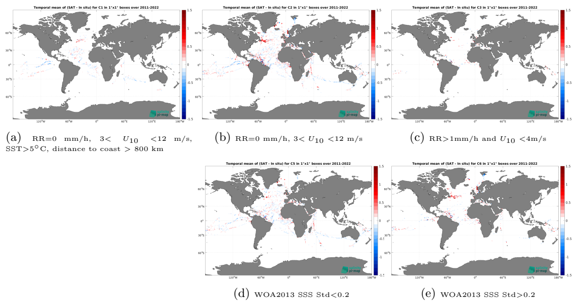
Figure 14: Temporal mean gridded over spatial boxes of size 1^\circ \times 1^\circ of \Delta SSS (SMAP SSS L4 OI v3 - Daily (ESR) - TSG (GOSUD-Research-vessel)) for 5 different subdatasets corresponding to: RR=0 mm/h, 3 < U_{10} < 12 m/s, SST > 5^\circ\text{C} , distance to coast > 800 km (a), RR=0 mm/h, 3 < U_{10} < 12 m/s (b), RR > 1 mm/h and U_{10} < 4 m/s (c), WOA2013 SSS Std < 0.2 (d), WOA2013 SSS Std > 0.2 (e).
