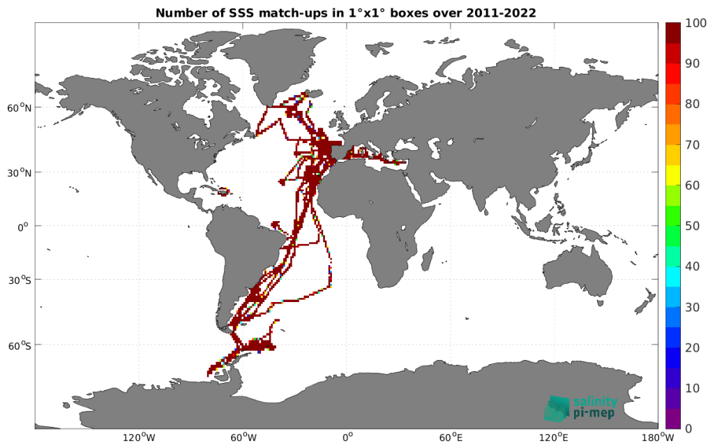
Figure 5: Number of SSS match-ups between TSG (CSIC-UTM) SSS and the SMAP SSS L4 OI v3 - Daily (ESR) SSS product for the Global Ocean Pi-MEP region over 1°x1° boxes and for the full satellite product period.
