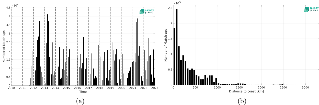
Figure 2: Number of match-ups between TSG (CSIC-UTM) and SMAP SSS L4 OI v3 - Daily (ESR) SSS as a function of time (a) and as function of the distance to coast (b) over the Global Ocean Pi-MEP region and for the full satellite product period.
