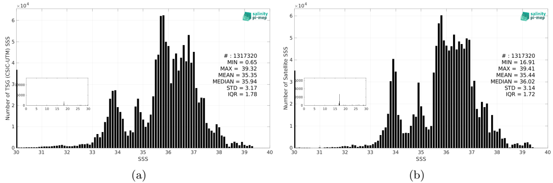
Figure 3: Histograms of SSS from TSG (CSIC-UTM) (a) and SMAP SSS L4 OI v3 - Daily (ESR) (b) considering all match-up pairs per bins of 0.1 over the Global Ocean Pi-MEP region and for the full satellite product period.
