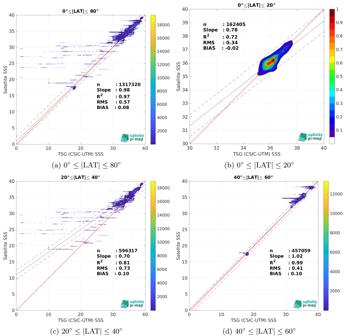
Figure 10: Contour maps of the concentration of SMAP SSS L4 OI v3 - Daily (ESR) SSS (y-axis) versus TSG (CSIC-UTM) SSS (x-axis) at match-up pairs for different latitude bands. For each plot, the red line shows x=y . The black thin and dashed lines indicate a linear fit through the data cloud and the \pm 95\% confidence levels, respectively. The number match-up pairs n , the slope and R^2 coefficient of the linear fit, the root mean square (RMS) and the mean bias between satellite and in situ data are indicated for each latitude band in each plots.
