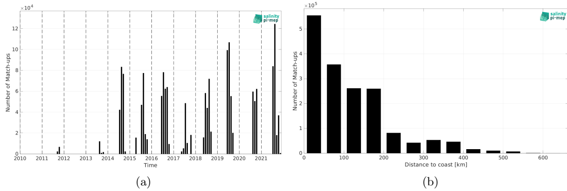
Figure 2: Number of match-ups between TSG (Amundsen) and SMAP SSS L4 OI v3 - Daily (ESR) SSS as a function of time (a) and as function of the distance to coast (b) over the Global Ocean Pi-MEP region and for the full satellite product period.
