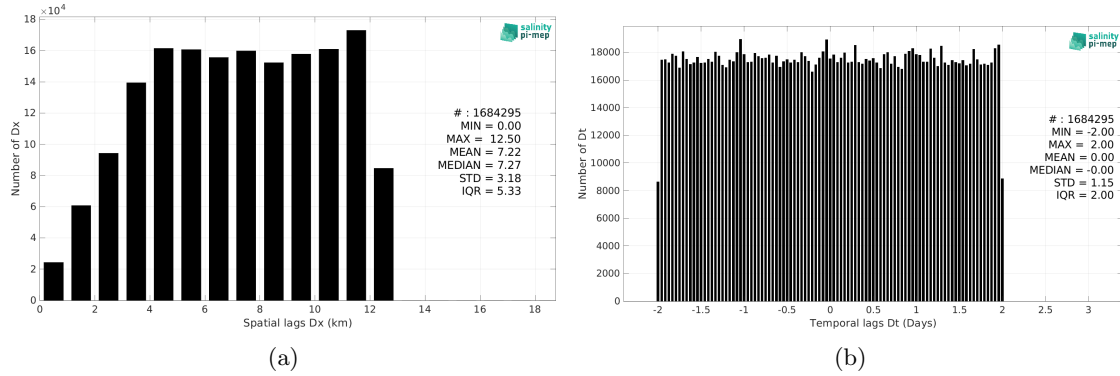
Figure 6: Histograms of the spatial (a) and temporal (b) lags between the location/time of the TSG (Amundsen) measurement and the date of the corresponding SMAP SSS L4 OI v3 - Daily (ESR) SSS pixel.
