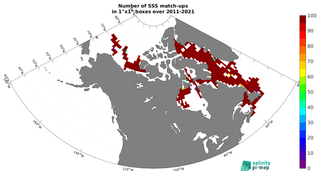
Figure 5: Number of SSS match-ups between TSG (Amundsen) SSS and the SMAP SSS L4 OI v3 - Daily (ESR) SSS product for the Global Ocean Pi-MEP region over 1^\circ \times 1^\circ boxes and for the full satellite product period.
