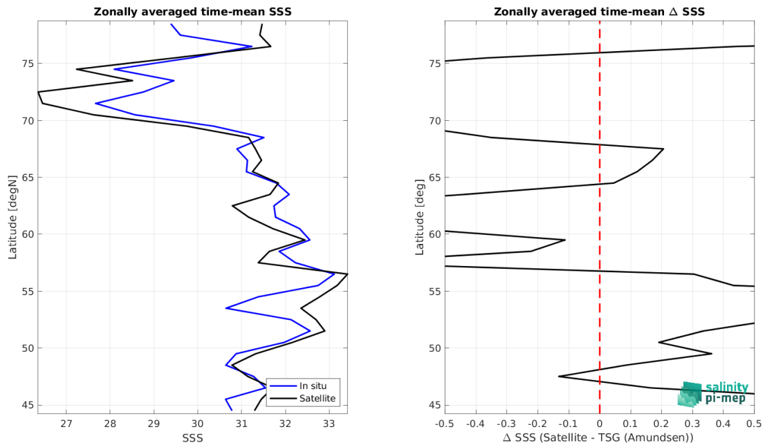
Figure 9: Left panel: Zonal mean SSS from SMAP SSS L4 OI v3 - Daily (ESR) satellite product (black) and from TSG (Amundsen) (blue). Right panel: Zonal mean of \Delta SSS (Satellite - TSG (Amundsen)) for all the collected Pi-MEP match-up pairs estimated over the full satellite product period.
