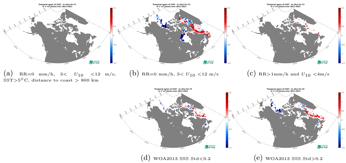
Figure 14: Temporal mean gridded over spatial boxes of size 1^\circ \times 1^\circ of \Delta SSS (SMAP SSS L4 OI v3 - Daily (ESR) - TSG (Amundsen)) for 5 different subdatasets corresponding to:RR=0 mm/h, 3 < U_{10} < 12 m/s, SST>5°C, distance to coast > 800 km (a), RR=0 mm/h, 3 < U_{10} < 12 m/s (b), RR>1mm/h and U_{10} < 4 m/s (c), WOA2013 SSS Std<0.2 (d), WOA2013 SSS Std>0.2 (e).
