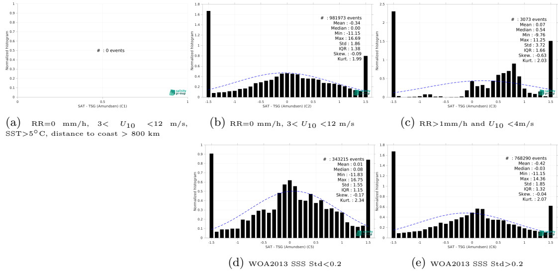
Figure 15: Normalized histogram of \Delta SSS (SMAP SSS L4 OI v3 - Daily (ESR) - TSG (Amundsen)) for 5 different subdatasets corresponding to: RR=0 mm/h, 3 < U_{10} < 12 m/s, SST > 5°C, distance to coast > 800 km (a), RR=0 mm/h, 3 < U_{10} < 12 m/s (b), RR > 1mm/h and U_{10} < 4 m/s (c), WOA2013 SSS Std < 0.2 (d), WOA2013 SSS Std > 0.2 (e).
