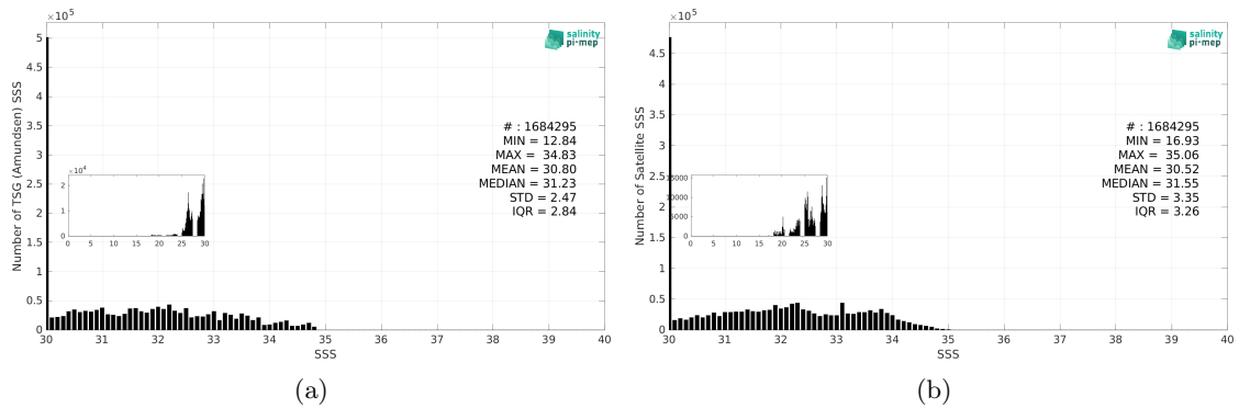
Figure 3: Histograms of SSS from TSG (Amundsen) (a) and SMAP SSS L4 OI v3 - Daily (ESR) (b) considering all match-up pairs per bins of 0.1 over the Global Ocean Pi-MEP region and for the full satellite product period.
