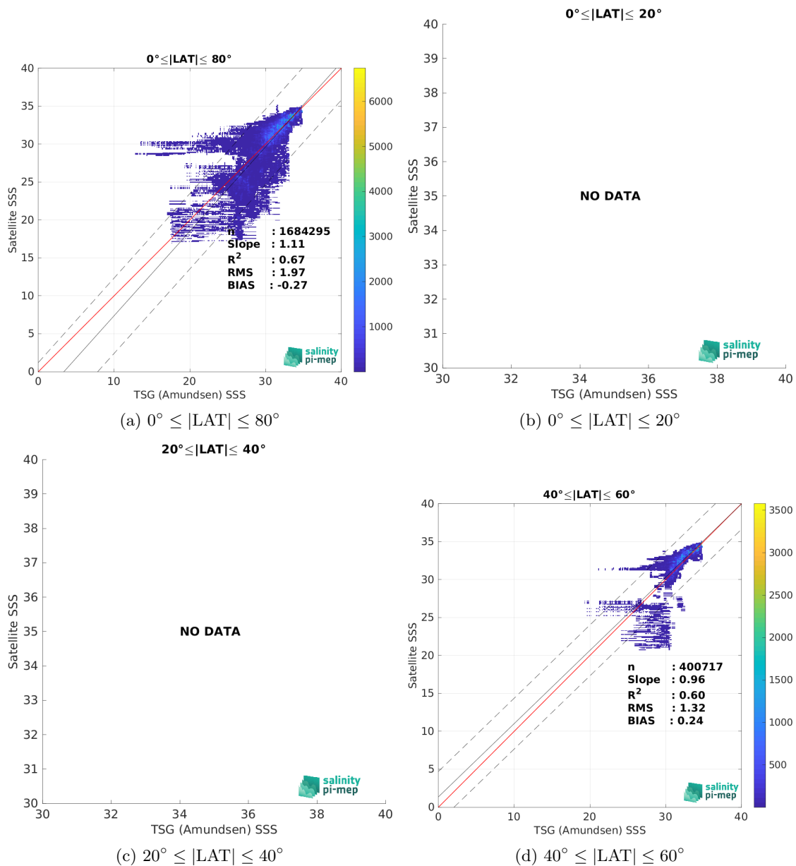
Figure 10: Contour maps of the concentration of SMAP SSS L4 OI v3 - Daily (ESR) SSS (y-axis) versus TSG (Amundsen) SSS (x-axis) at match-up pairs for different latitude bands. For each plot, the red line shows x=y . The black thin and dashed lines indicate a linear fit through the data cloud and the \pm 95\% confidence levels, respectively. The number match-up pairs n , the slope and R^2 coefficient of the linear fit, the root mean square (RMS) and the mean bias between satellite and in situ data are indicated for each latitude band in each plot.
