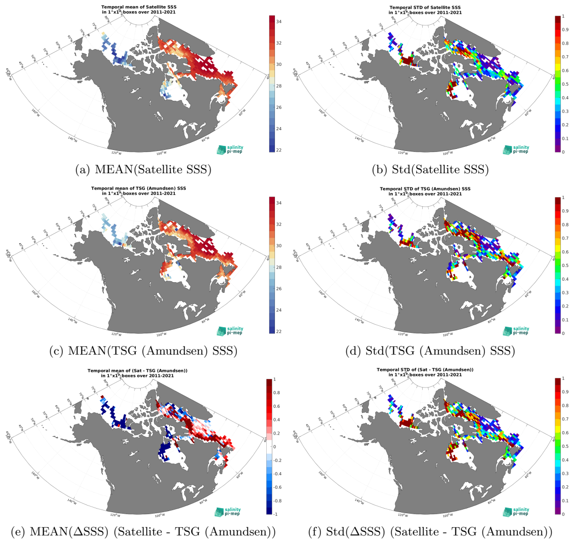
Figure 7: Temporal mean (left) and Std (right) of SSS from SMAP SSS L4 OI v3 - Daily (ESR) (top), TSG (Amundsen) (middle), and of \Delta SSS (Satellite - TSG (Amundsen)). Only match-up pairs are used to generate these maps.
