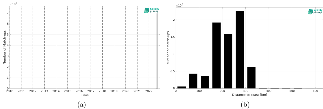
Figure 2: Number of match-ups between SASSIE and SMAP SSS L4 OI v3 - Daily (ESR) SSS as a function of time (a) and as function of the distance to coast (b) over the Global Ocean Pi-MEP region and for the full satellite product period.
