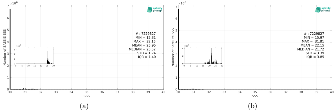
Figure 3: Histograms of SSS from SASSIE (a) and SMAP SSS L4 OI v3 - Daily (ESR) (b) considering all match-up pairs per bins of 0.1 over the Global Ocean Pi-MEP region and for the full satellite product period.
