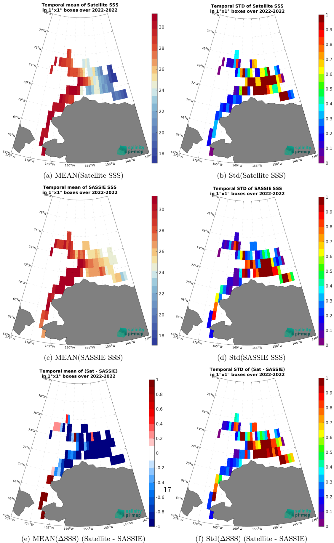
Figure 7: Temporal mean (left) and Std (right) of SSS from SMAP SSS L4 OI v3 - Daily (ESR) (top), SASSIE (middle), and of \Delta SSS (Satellite - SASSIE). Only match-up pairs are used to generate these maps.
