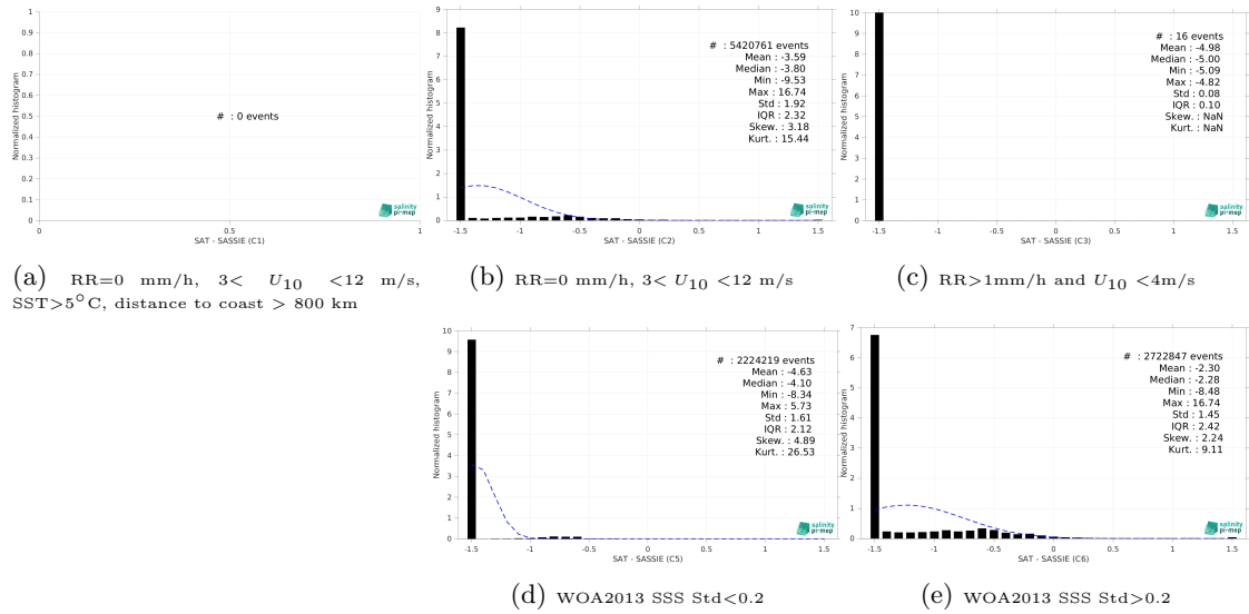
Figure 15: Normalized histogram of \Delta SSS (SMAP SSS L4 OI v3 - Daily (ESR) - SASSIE) for 5 different subdatasets corresponding to: RR=0 mm/h, 3 < U_{10} < 12 m/s, SST > 5°C, distance to coast > 800 km (a), RR=0 mm/h, 3 < U_{10} < 12 m/s (b), RR > 1mm/h and U_{10} < 4 m/s (c), WOA2013 SSS Std < 0.2 (d), WOA2013 SSS Std > 0.2 (e).
