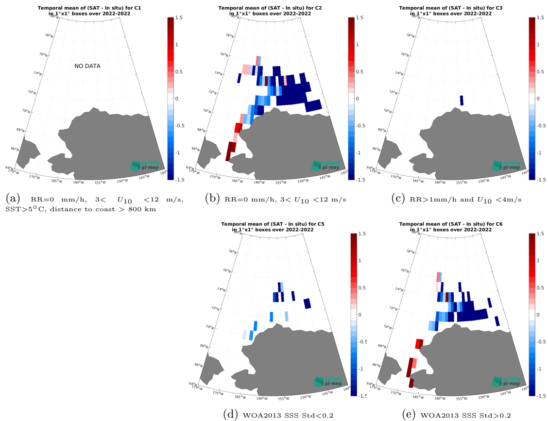
Figure 14: Temporal mean gridded over spatial boxes of size 1^\circ \times 1^\circ of \Delta\text{SSS} (SMAP SSS L4 OI v3 - Daily (ESR) - SASSIE) for 5 different subdatasets corresponding to:RR=0 mm/h, 3 < U_{10} < 12 m/s, SST>5°C, distance to coast > 800 km (a), RR=0 mm/h, 3 < U_{10} < 12 m/s (b), RR>1mm/h and U_{10} < 4 m/s (c), WOA2013 SSS Std<0.2 (d), WOA2013 SSS Std>0.2 (e).
