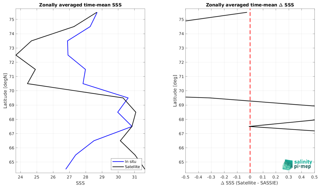
Figure 9: Left panel: Zonal mean SSS from SMAP SSS L4 OI v3 - Daily (ESR) satellite product (black) and from SASSIE (blue). Right panel: Zonal mean of \Delta SSS (Satellite - SASSIE) for all the collected Pi-MEP match-up pairs estimated over the full satellite product period.
