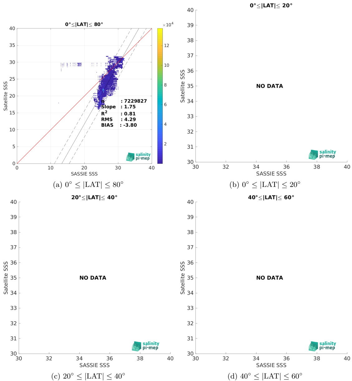
Figure 10: Contour maps of the concentration of SMAP SSS L4 OI v3 - Daily (ESR) SSS (y-axis) versus SASSIE SSS (x-axis) at match-up pairs for different latitude bands. For each plot, the red line shows x=y . The black thin and dashed lines indicate a linear fit through the data cloud and the \pm 95\% confidence levels, respectively. The number match-up pairs n , the slope and R^2 coefficient of the linear fit, the root mean square (RMS) and the mean bias between satellite and in situ data are indicated for each latitude band in each plots.
