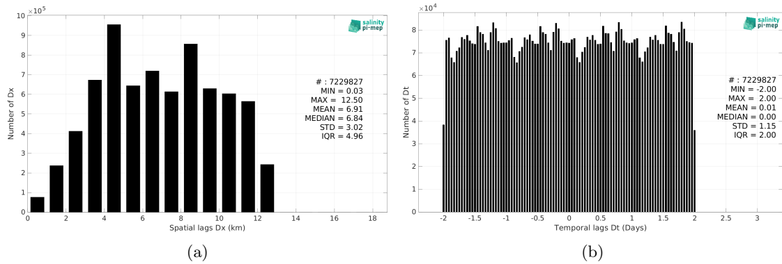
Figure 6: Histograms of the spatial (a) and temporal (b) lags between the location/time of the SASSIE measurement and the date of the corresponding SMAP SSS L4 OI v3 - Daily (ESR) SSS pixel.
