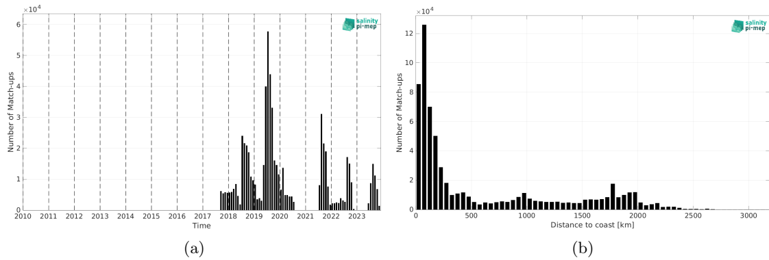
Figure 2: Number of match-ups between Saildrone and SMAP SSS L4 OI v3 - Daily (ESR) SSS as a function of time (a) and as function of the distance to coast (b) over the Global Ocean Pi-MEP region and for the full satellite product period.
