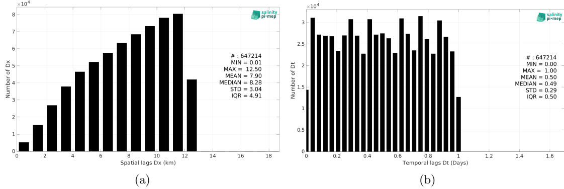
Figure 6: Histograms of the spatial (a) and temporal (b) lags between the location/time of the Saildrone measurement and the date of the corresponding SMAP SSS L4 OI v3 - Daily (ESR) SSS pixel.
