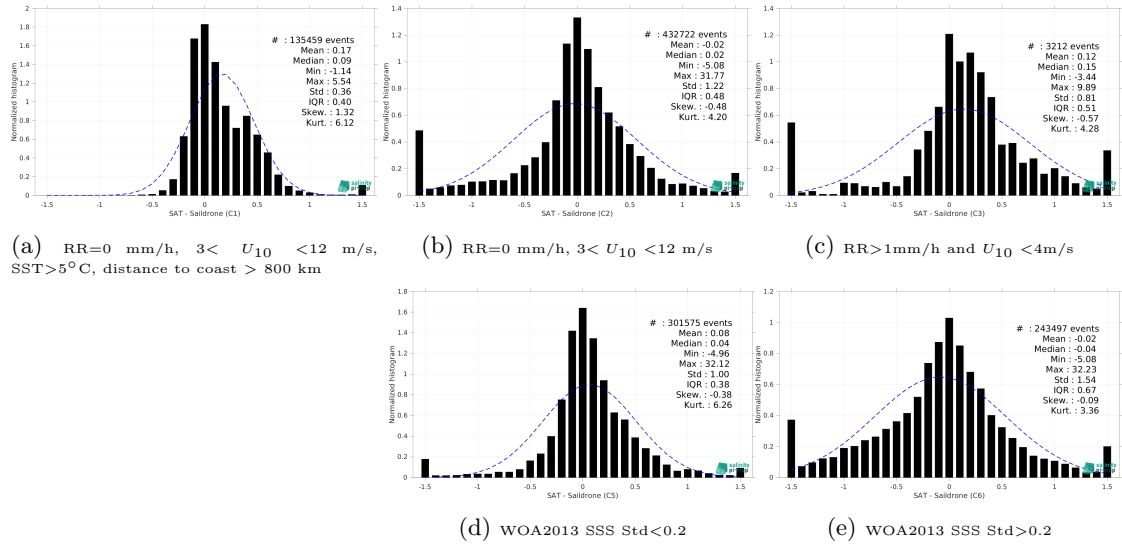
Figure 15: Normalized histogram of \Delta\text{SSS} (SMAP SSS L4 OI v3 - Daily (ESR) - Saildrone) for 5 different subdatasets corresponding to: RR=0 mm/h, 3 < U_{10} < 12 m/s, SST>5°C, distance to coast > 800 km (a), RR=0 mm/h, 3 < U_{10} < 12 m/s (b), RR>1mm/h and U_{10} < 4 m/s (c), WOA2013 SSS Std<0.2 (d), WOA2013 SSS Std>0.2 (e).
