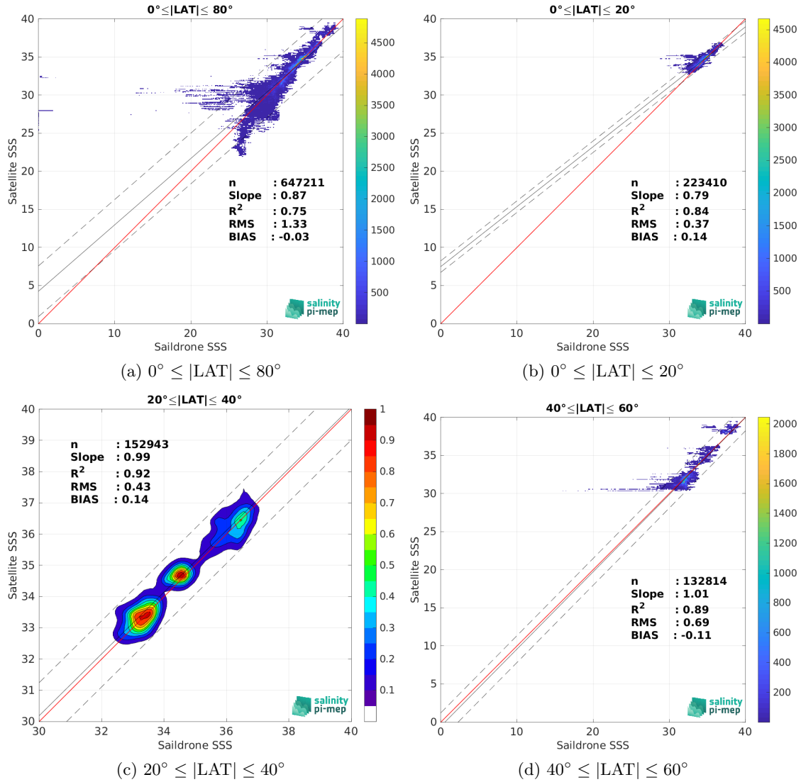
Figure 10: Contour maps of the concentration of SMAP SSS L4 OI v3 - Daily (ESR) SSS (y-axis) versus Saildrone SSS (x-axis) at match-up pairs for different latitude bands. For each plot, the red line shows x=y . The black thin and dashed lines indicate a linear fit through the data cloud and the \pm 95\% confidence levels, respectively. The number match-up pairs n , the slope and R^2 coefficient of the linear fit, the root mean square (RMS) and the mean bias between satellite and in situ data are indicated for each latitude band in each plots.
