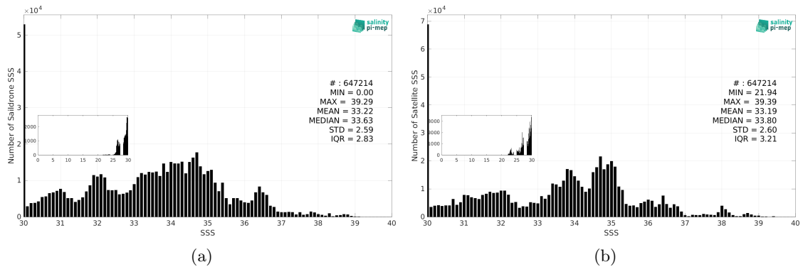
Figure 3: Histograms of SSS from Saildrone (a) and SMAP SSS L4 OI v3 - Daily (ESR) (b) considering all match-up pairs per bins of 0.1 over the Global Ocean Pi-MEP region and for the full satellite product period.
