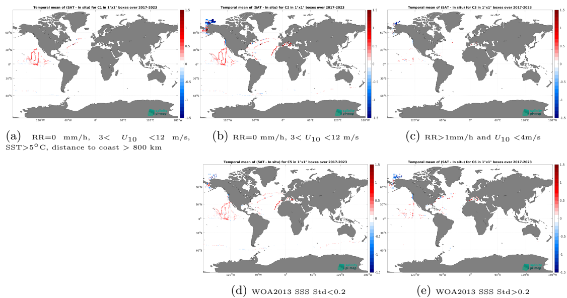
Figure 14: Temporal mean gridded over spatial boxes of size 1^\circ \times 1^\circ of \Delta SSS (SMAP SSS L4 OI v3 - Daily (ESR) - Saildrone) for 5 different subdatasets corresponding to:RR=0 mm/h, 3 < U_{10} < 12 m/s, SST > 5^\circ\text{C} , distance to coast > 800 km (a), RR=0 mm/h, 3 < U_{10} < 12 m/s (b), RR > 1 mm/h and U_{10} < 4 m/s (c), WOA2013 SSS Std < 0.2 (d), WOA2013 SSS Std > 0.2 (e).
