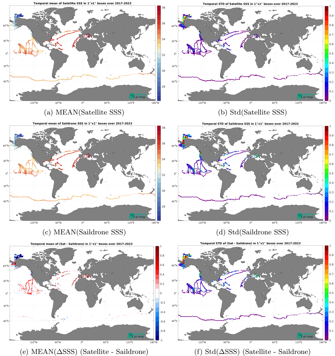
Figure 7: Temporal mean (left) and Std (right) of SSS from SMAP SSS L4 OI v3 - Daily (ESR) (top), Saildrone (middle), and of \Delta SSS (Satellite - Saildrone). Only match-up pairs are used to generate these maps.
