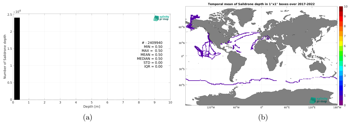
Figure 4: Histograms of the depth of the upper level SSS measurements from Salldrone in the Match-up DataBase for the Global Ocean Pi-MEP region (a) and temporal mean spatial distribution of pressure of the in situ SSS data over 1^\circ \times 1^\circ boxes and for the full satellite product period (b).
