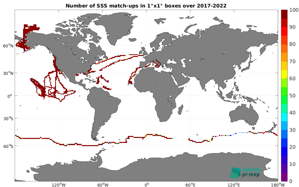
Figure 5: Number of SSS match-ups between Salldrone SSS and the SMAP SSS L4 OI v3 - Daily (ESR) SSS product for the Global Ocean Pi-MEP region over 1^\circ \times 1^\circ boxes and for the full satellite product period.
