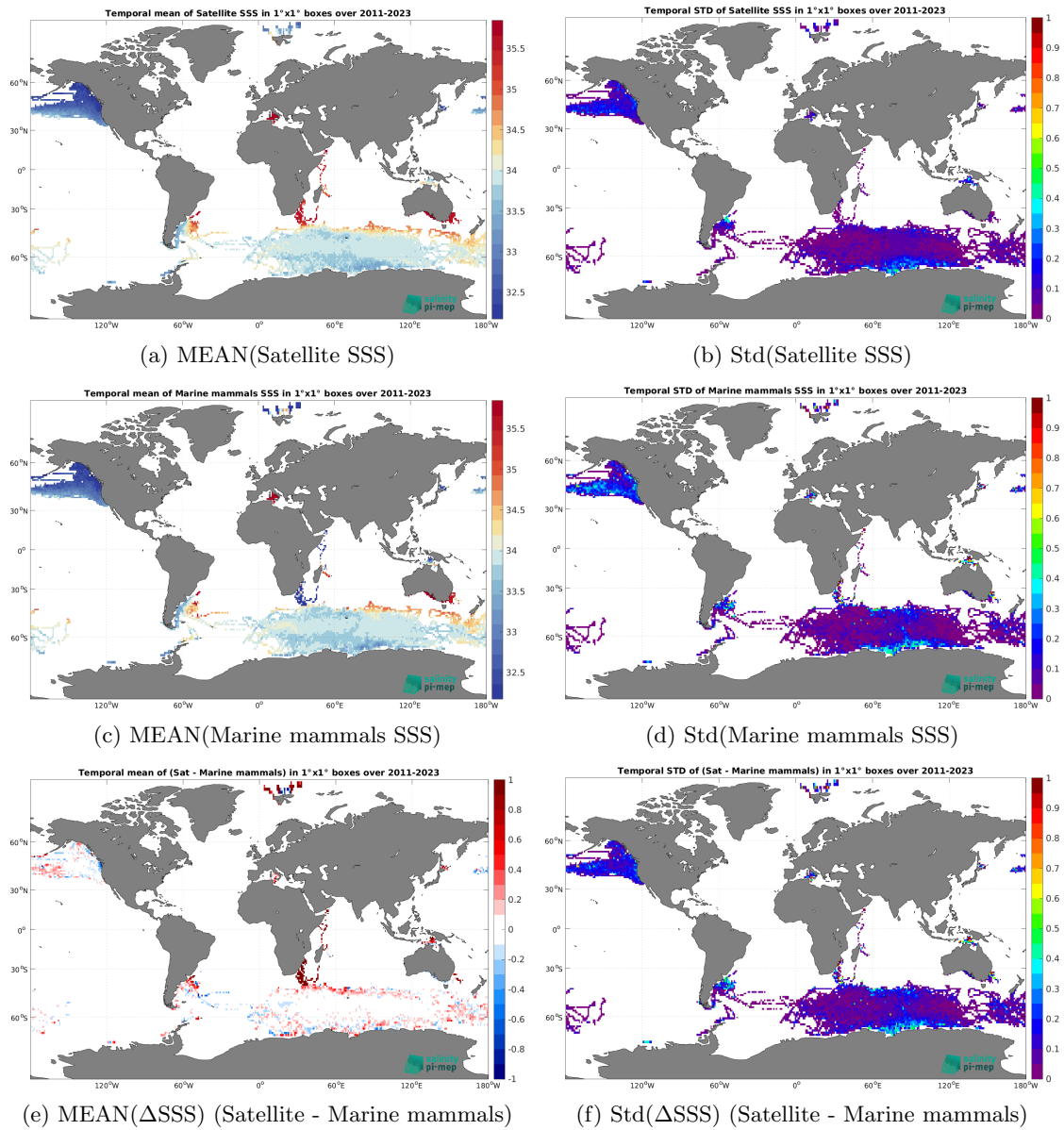
Figure 7: Temporal mean (left) and Std (right) of SSS from SMAP SSS L4 OI v3 - Daily (ESR) (top), Marine mammals (middle), and of \Delta SSS (Satellite - Marine mammals). Only match-up pairs are used to generate these maps.
