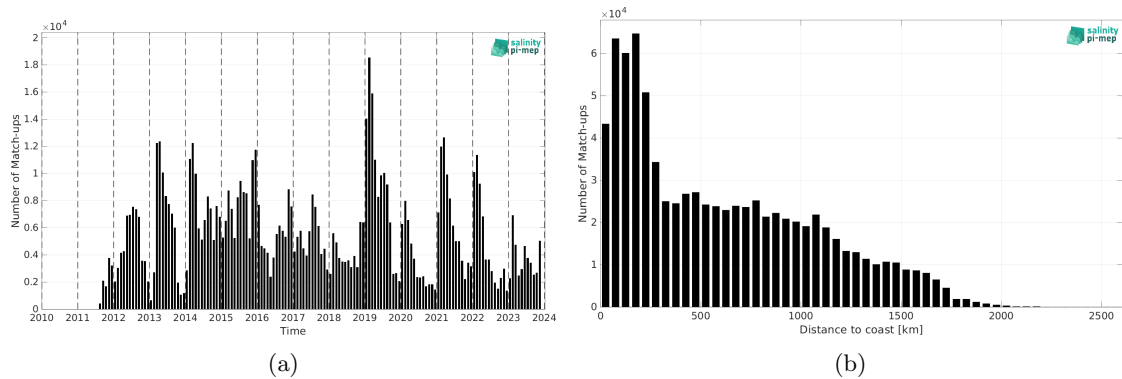
Figure 2: Number of match-ups between Marine mammals and SMAP SSS L4 OI v3 - Daily (ESR) SSS as a function of time (a) and as function of the distance to coast (b) over the Global Ocean Pi-MEP region and for the full satellite product period.
