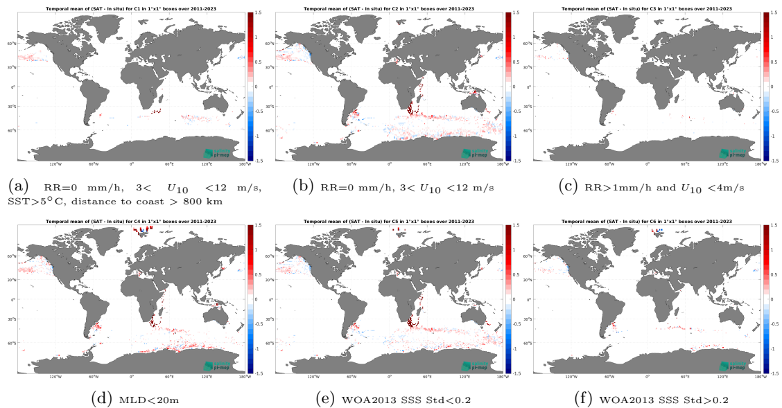
Figure 14: Temporal mean gridded over spatial boxes of size 1^\circ \times 1^\circ of \Delta SSS (SMAP SSS L4 OI v3 - Daily (ESR) - Marine mammals) for 6 different subdatasets corresponding to:RR=0 mm/h, 3 < U_{10} < 12 m/s, SST >5^\circ C, distance to coast > 800 km (a), RR=0 mm/h, 3 < U_{10} < 12 m/s (b), RR >1 mm/h and U_{10} < 4 m/s (c),MLD <20 m (d),WOA2013 SSS Std <0.2 (e),WOA2013 SSS Std >0.2 (f).
