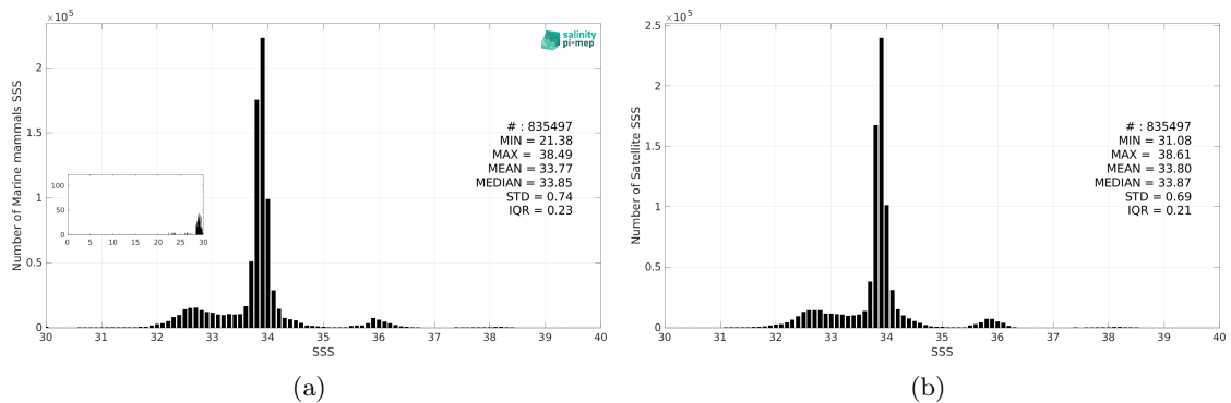
Figure 3: Histograms of SSS from Marine mammals (a) and SMAP SSS L4 OI v3 - Daily (ESR) (b) considering all match-up pairs per bins of 0.1 over the Global Ocean Pi-MEP region and for the full satellite product period.
