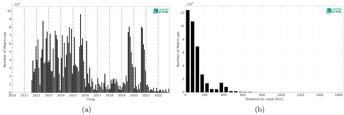
Figure 2: Number of match-ups between ICES and SMAP SSS L4 OI v3 - Daily (ESR) SSS as a function of time (a) and as function of the distance to coast (b) over the Global Ocean Pi-MEP region and for the full satellite product period.
