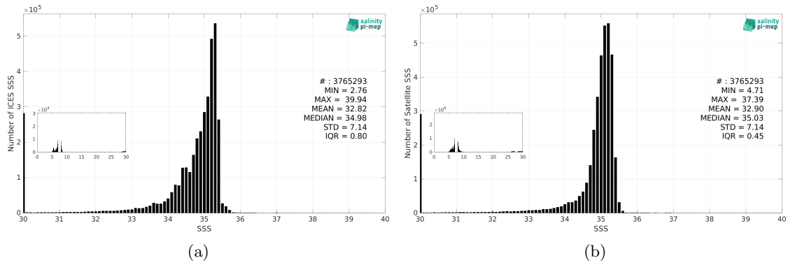
Figure 3: Histograms of SSS from ICES (a) and SMAP SSS L4 OI v3 - Daily (ESR) (b) considering all match-up pairs per bins of 0.1 over the Global Ocean Pi-MEP region and for the full satellite product period.
