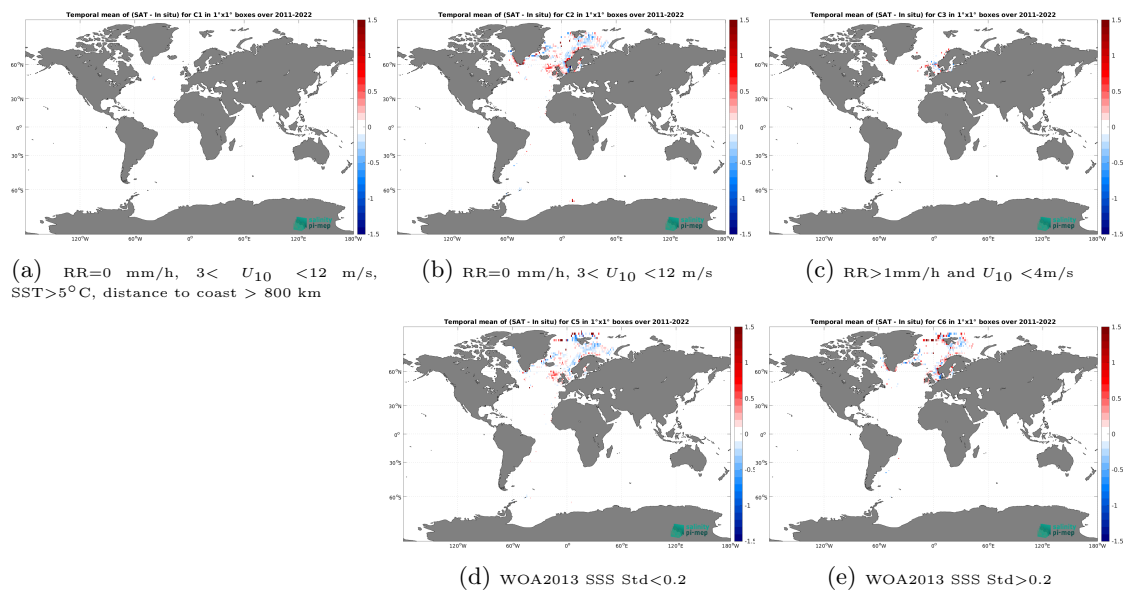
Figure 14: Temporal mean gridded over spatial boxes of size 1^\circ \times 1^\circ of \Delta SSS (SMAP SSS L4 OI v3 - Daily (ESR) - ICES) for 5 different subdatasets corresponding to:RR=0 mm/h, 3 < U_{10} < 12 m/s, SST > 5^\circ\text{C} , distance to coast > 800 km (a), RR=0 mm/h, 3 < U_{10} < 12 m/s (b), RR > 1 mm/h and U_{10} < 4 m/s (c), WOA2013 SSS Std < 0.2 (d), WOA2013 SSS Std > 0.2 (e).
