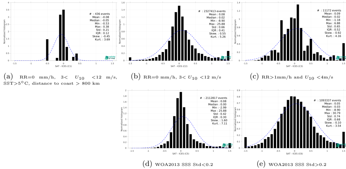
Figure 15: Normalized histogram of \Delta\text{SSS} (SMAP SSS L4 OI v3 - Daily (ESR) - ICES) for 5 different subdatasets corresponding to: RR=0 mm/h, 3 < U_{10} < 12 m/s, SST>5°C, distance to coast > 800 km (a), RR=0 mm/h, 3 < U_{10} < 12 m/s (b), RR>1mm/h and U_{10} < 4 m/s (c), WOA2013 SSS Std<0.2 (d), WOA2013 SSS Std>0.2 (e).
