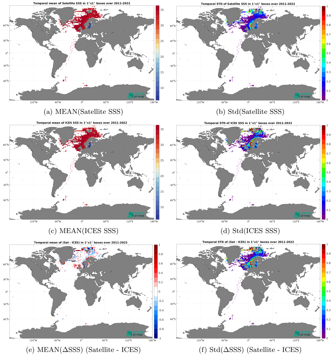
Figure 7: Temporal mean (left) and Std (right) of SSS from SMAP SSS L4 OI v3 - Daily (ESR) (top), ICES (middle), and of \Delta SSS (Satellite - ICES). Only match-up pairs are used to generate these maps.
