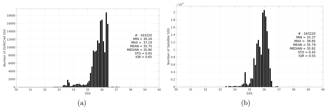
Figure 3: Histograms of SSS from EUREC4A (a) and SMAP SSS L4 OI v3 - Daily (ESR) (b) considering all match-up pairs per bins of 0.1 over the Global Ocean Pi-MEP region and for the full satellite product period.
