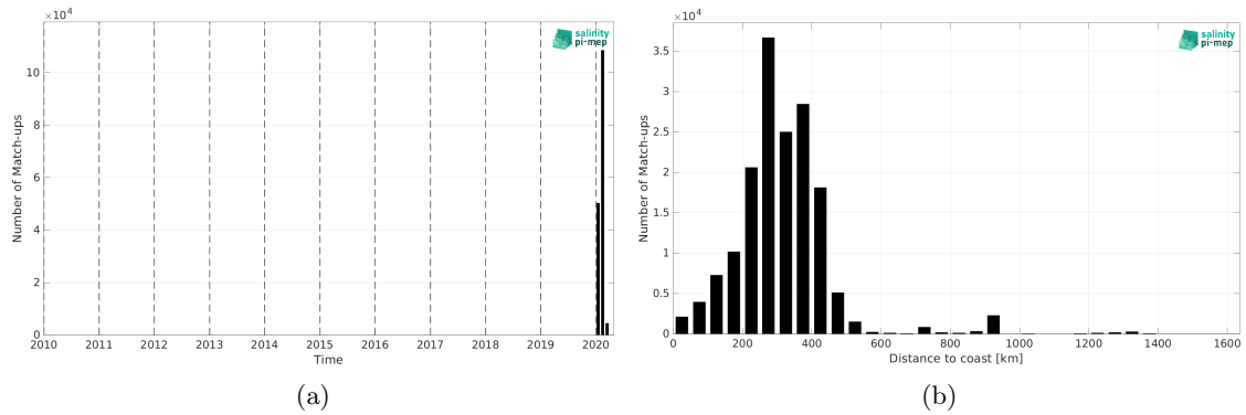
Figure 2: Number of match-ups between EUREC4A and SMAP SSS L4 OI v3 - Daily (ESR) SSS as a function of time (a) and as function of the distance to coast (b) over the Global Ocean Pi-MEP region and for the full satellite product period.
