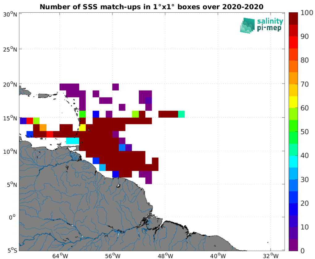
Figure 5: Number of SSS match-ups between EUREC4A SSS and the SMAP SSS L4 OI v3 - Daily (ESR) SSS product for the Global Ocean Pi-MEP region over 1^\circ \times 1^\circ boxes and for the full satellite product period.
