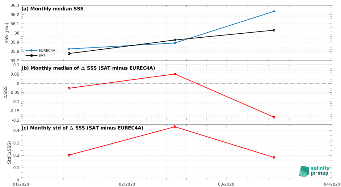
Figure 8: Time series of the monthly median SSS (top), median of \Delta SSS (Satellite - EUREC4A) and Std of \Delta SSS (Satellite - EUREC4A) over the Global Ocean Pi-MEP region considering all match-ups collected by the Pi-MEP.
