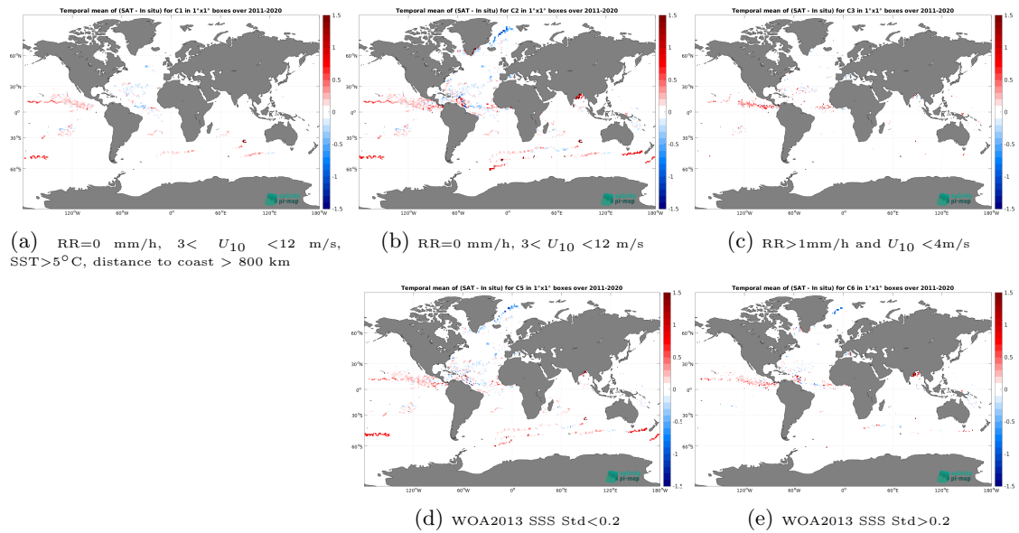
Figure 13: Temporal mean gridded over spatial boxes of size 1^\circ \times 1^\circ of \Delta SSS (SMAP SSS L4 OI v3 - Daily (ESR) - Surface drifters) for 5 different subdatasets corresponding to:RR=0 mm/h, 3 < U_{10} < 12 m/s, SST > 5^\circ\text{C} , distance to coast > 800 km (a), RR=0 mm/h, 3 < U_{10} < 12 m/s (b), RR > 1 mm/h and U_{10} < 4 m/s (c), WOA2013 SSS Std < 0.2 (d), WOA2013 SSS Std > 0.2 (e).
