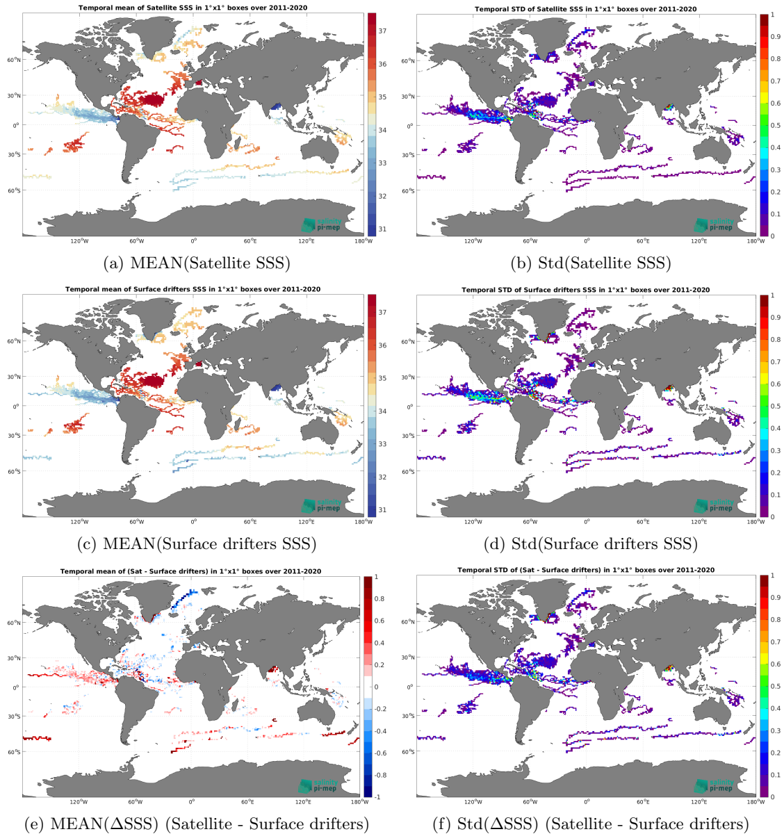
Figure 6: Temporal mean (left) and Std (right) of SSS from SMAP SSS L4 OI v3 - Daily (ESR) (top), Surface drifters (middle), and of \Delta SSS (Satellite - Surface drifters). Only match-up pairs are used to generate these maps.
