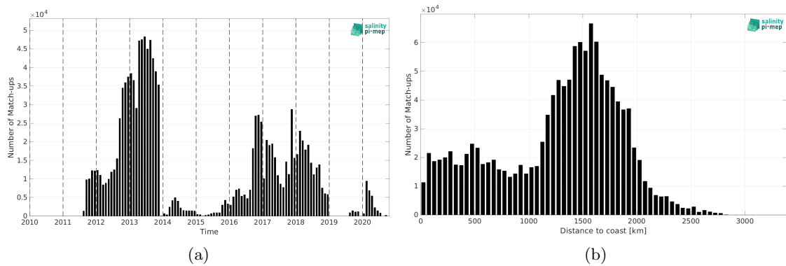
Figure 2: Number of match-ups between Surface drifters and SMAP SSS L4 OI v3 - Daily (ESR) SSS as a function of time (a) and as function of the distance to coast (b) over the Global Ocean Pi-MEP region and for the full satellite product period.
