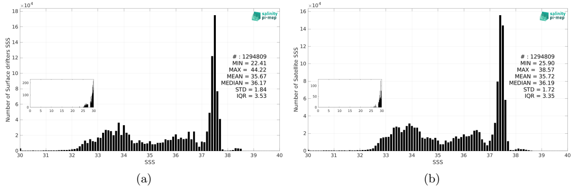
Figure 3: Histograms of SSS from Surface drifters (a) and SMAP SSS L4 OI v3 - Daily (ESR) (b) considering all match-up pairs per bins of 0.1 over the Global Ocean Pi-MEP region and for the full satellite product period.
