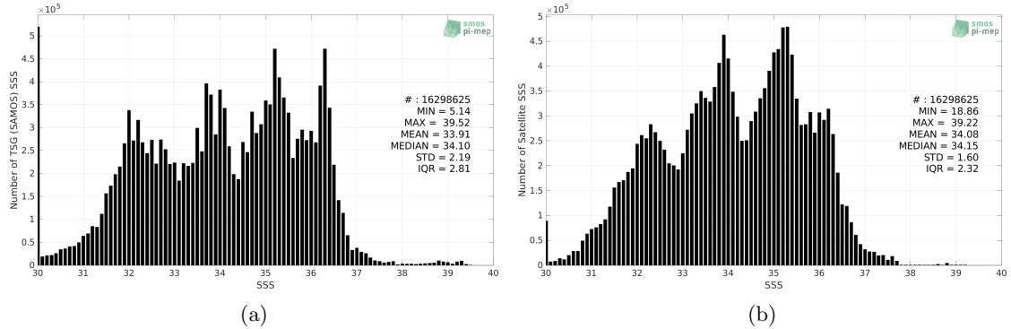
Figure 2: Histograms of SSS from TSG (SAMOS) (a) and SMAP SSS L4 OI v2 - 7 Days (ESR) (b) considering all match-up pairs per bins of 0.1 over the Global Ocean Pi-MEP region and for the full satellite product period.
