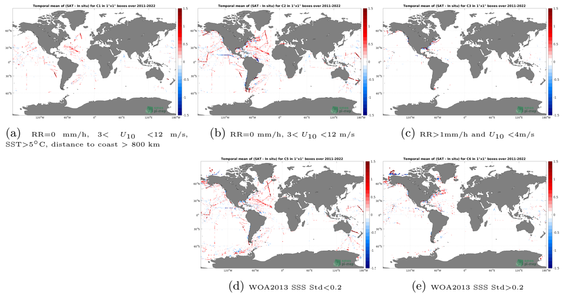
Figure 12: Temporal mean gridded over spatial boxes of size 1^\circ \times 1^\circ of \Delta SSS (SMAP SSS L4 OI v2 - 7 Days (ESR) - TSG (SAMOS)) for 5 different subdatasets corresponding to:RR=0 mm/h, 3 < U_{10} < 12 m/s, SST > 5^\circ\text{C} , distance to coast > 800 km (a), RR=0 mm/h, 3 < U_{10} < 12 m/s (b), RR > 1 mm/h and U_{10} < 4 m/s (c), WOA2013 SSS Std < 0.2 (d), WOA2013 SSS Std > 0.2 (e).
