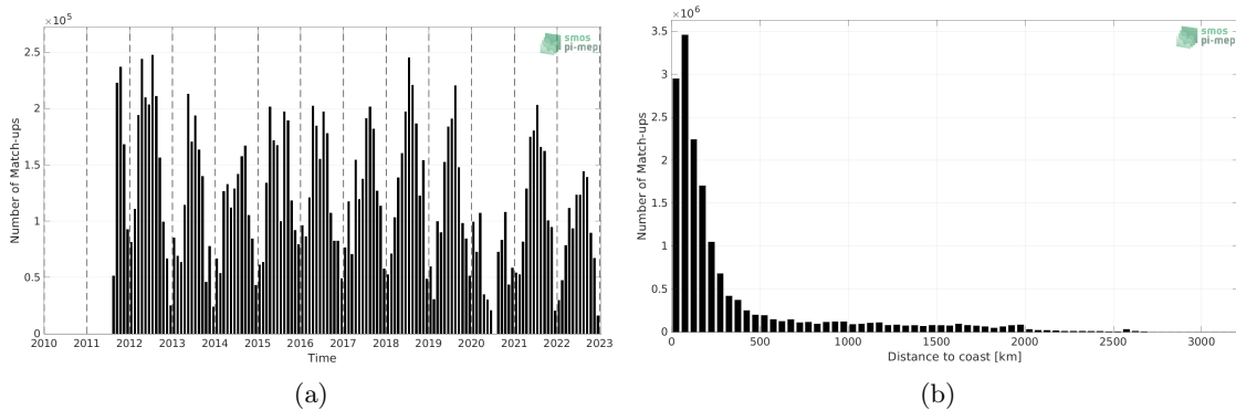
Figure 1: Number of match-ups between TSG (SAMOS) and SMAP SSS L4 OI v2 - 7 Days (ESR) SSS as a function of time (a) and as function of the distance to coast (b) over the Global Ocean Pi-MEP region and for the full satellite product period.
