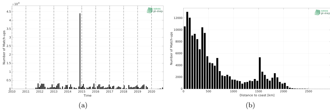
Figure 1: Number of match-ups between TSG (Polarstern) and SMAP SSS L4 OI v2 - 7 Days (ESR) SSS as a function of time (a) and as function of the distance to coast (b) over the Global Ocean Pi-MEP region and for the full satellite product period.
