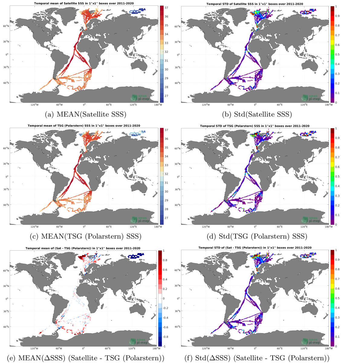
Figure 6: Temporal mean (left) and Std (right) of SSS from SMAP SSS L4 OI v2 - 7 Days (ESR) (top), TSG (Polarstern) (middle), and of \Delta SSS (Satellite - TSG (Polarstern)). Only match-up pairs are used to generate these maps.
