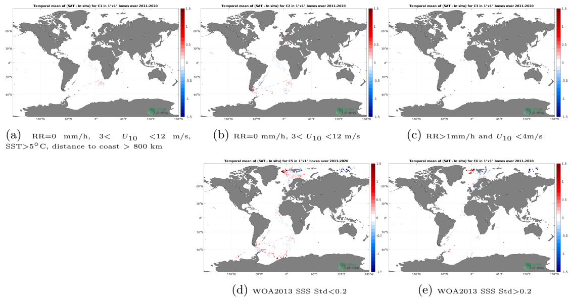
Figure 12: Temporal mean gridded over spatial boxes of size 1^\circ \times 1^\circ of \Delta SSS (SMAP SSS L4 OI v2 - 7 Days (ESR) - TSG (Polarstern)) for 5 different subdatasets corresponding to:RR=0 mm/h, 3 < U_{10} < 12 m/s, SST >5^\circ C, distance to coast > 800 km (a), RR=0 mm/h, 3 < U_{10} < 12 m/s (b), RR >1 mm/h and U_{10} < 4 m/s (c), WOA2013 SSS Std <0.2 (d), WOA2013 SSS Std >0.2 (e).
