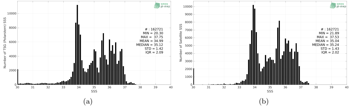
Figure 2: Histograms of SSS from TSG (Polarstern) (a) and SMAP SSS L4 OI v2 - 7 Days (ESR) (b) considering all match-up pairs per bins of 0.1 over the Global Ocean Pi-MEP region and for the full satellite product period.
