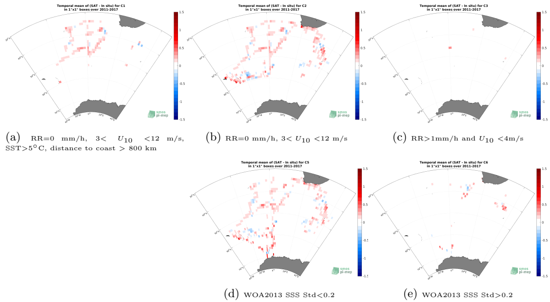
Figure 12: Temporal mean gridded over spatial boxes of size 1^\circ \times 1^\circ of \Delta SSS (SMAP SSS L4 OI v2 - 7 Days (ESR) - TSG (NCEI-0170743)) for 5 different subdatasets corresponding to:RR=0 mm/h, 3 < U_{10} < 12 m/s, SST > 5^\circ\text{C} , distance to coast > 800 km (a), RR=0 mm/h, 3 < U_{10} < 12 m/s (b), RR > 1 mm/h and U_{10} < 4 m/s (c), WOA2013 SSS Std < 0.2 (d), WOA2013 SSS Std > 0.2 (e).
