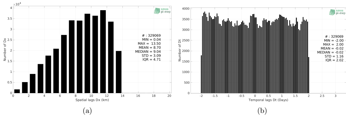
Figure 5: Histograms of the spatial (a) and temporal (b) lags between the location/time of the TSG (NCEI-0170743) measurement and the date of the corresponding SMAP SSS L4 OI v2 - 7 Days (ESR) SSS pixel.
