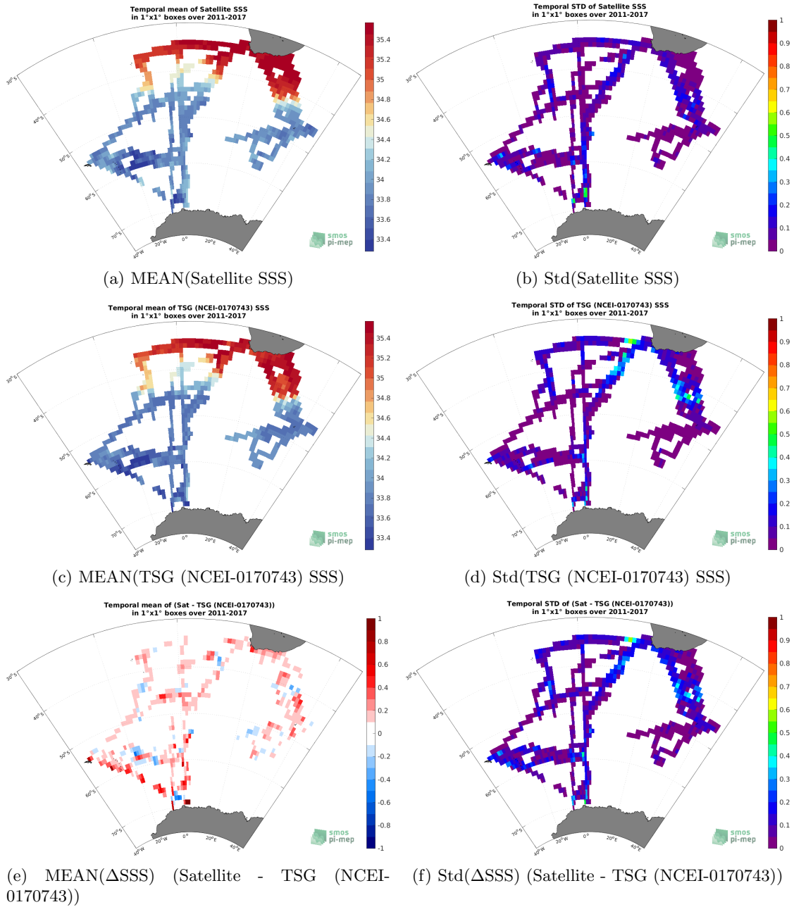
Figure 6: Temporal mean (left) and Std (right) of SSS from SMAP SSS L4 OI v2 - 7 Days (ESR) (top), TSG (NCEI-0170743) (middle), and of \Delta SSS (Satellite - TSG (NCEI-0170743)). Only match-up pairs are used to generate these maps.
