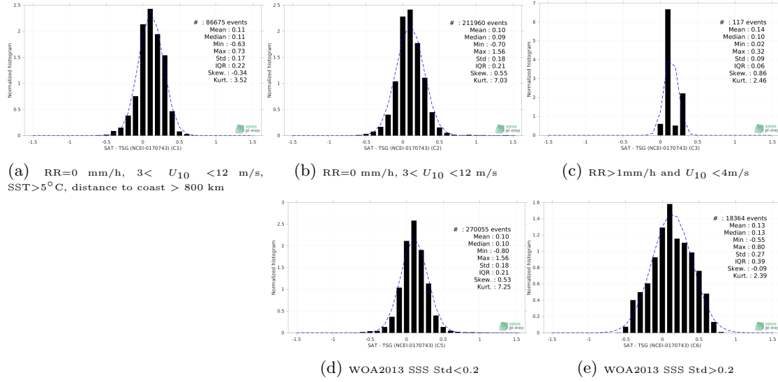
Figure 13: Normalized histogram of \Delta SSS (SMAP SSS L4 OI v2 - 7 Days (ESR) - TSG (NCEI-0170743)) for 5 different subdatasets corresponding to: RR=0 mm/h, 3 < U_{10} < 12 m/s, SST>5°C, distance to coast > 800 km (a), RR=0 mm/h, 3 < U_{10} < 12 m/s (b), RR>1mm/h and U_{10} < 4 m/s (c), WOA2013 SSS Std<0.2 (d), WOA2013 SSS Std>0.2 (e).
