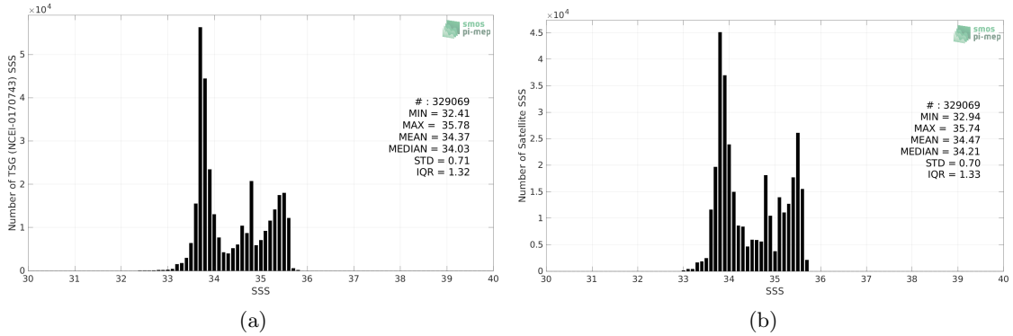
Figure 2: Histograms of SSS from TSG (NCEI-0170743) (a) and SMAP SSS L4 OI v2 - 7 Days (ESR) (b) considering all match-up pairs per bins of 0.1 over the Global Ocean Pi-MEP region and for the full satellite product period.
