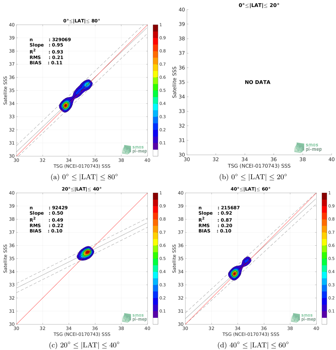
Figure 9: Contour maps of the concentration of SMAP SSS L4 OI v2 - 7 Days (ESR) SSS (y-axis) versus TSG (NCEI-0170743) SSS (x-axis) at match-up pairs for different latitude bands. For each plot, the red line shows x=y . The black thin and dashed lines indicate a linear fit through the data cloud and the \pm 95\% confidence levels, respectively. The number match-up pairs n , the slope and R^2 coefficient of the linear fit, the root mean square (RMS) and the mean bias between satellite and in situ data are indicated for each latitude band in each plots.
