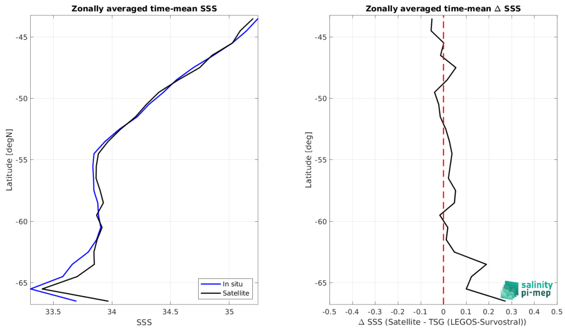
Figure 8: Left panel: Zonal mean SSS from SMAP SSS L4 OI v2 - 7 Days (ESR) satellite product (black) and from TSG (LEGOS-Survostral) (blue). Right panel: Zonal mean of \Delta SSS (Satellite - TSG (LEGOS-Survostral)) for all the collected Pi-MEP match-up pairs estimated over the full satellite product period.
