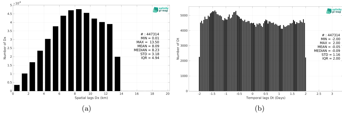
Figure 5: Histograms of the spatial (a) and temporal (b) lags between the location/time of the TSG (LEGOS-Survostral) measurement and the date of the corresponding SMAP SSS L4 OI v2 - 7 Days (ESR) SSS pixel.
