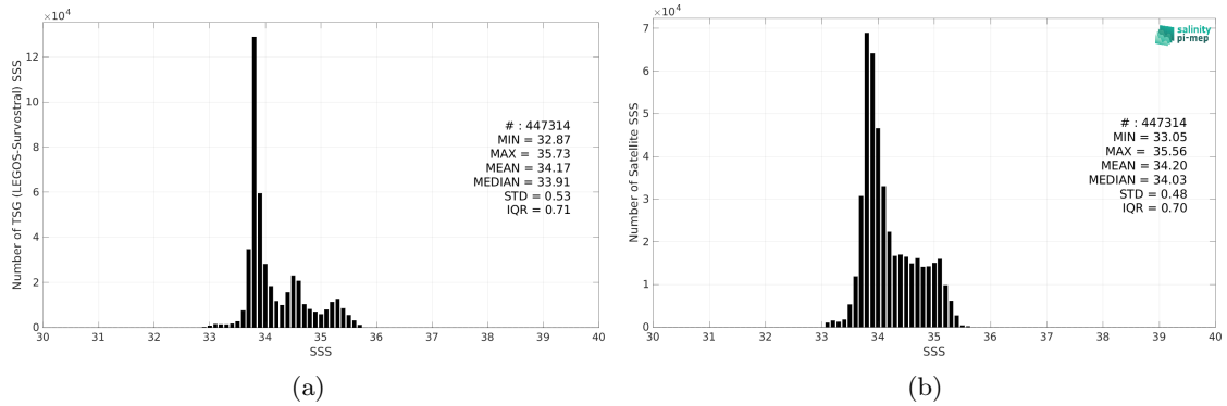
Figure 2: Histograms of SSS from TSG (LEGOS-Survostral) (a) and SMAP SSS L4 OI v2 - 7 Days (ESR) (b) considering all match-up pairs per bins of 0.1 over the Global Ocean Pi-MEP region and for the full satellite product period.
