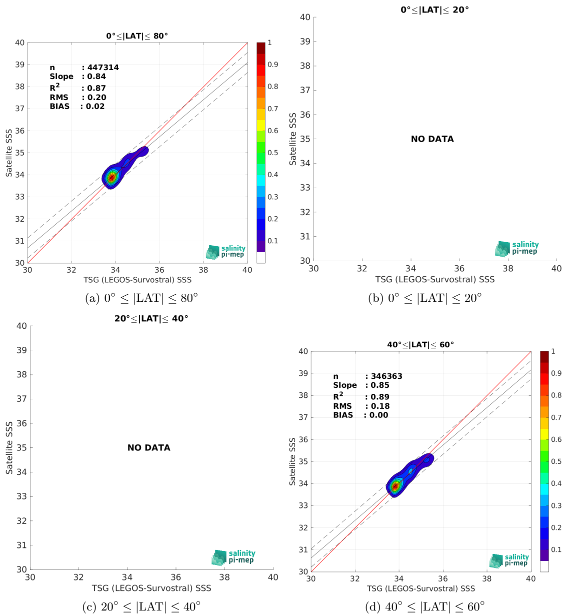
Figure 9: Contour maps of the concentration of SMAP SSS L4 OI v2 - 7 Days (ESR) SSS (y-axis) versus TSG (LEGOS-Survostral) SSS (x-axis) at match-up pairs for different latitude bands. For each plot, the red line shows x=y . The black thin and dashed lines indicate a linear fit through the data cloud and the \pm 95\% confidence levels, respectively. The number match-up pairs n , the slope and R^2 coefficient of the linear fit, the root mean square (RMS) and the mean bias between satellite and in situ data are indicated for each latitude band in each plots.
