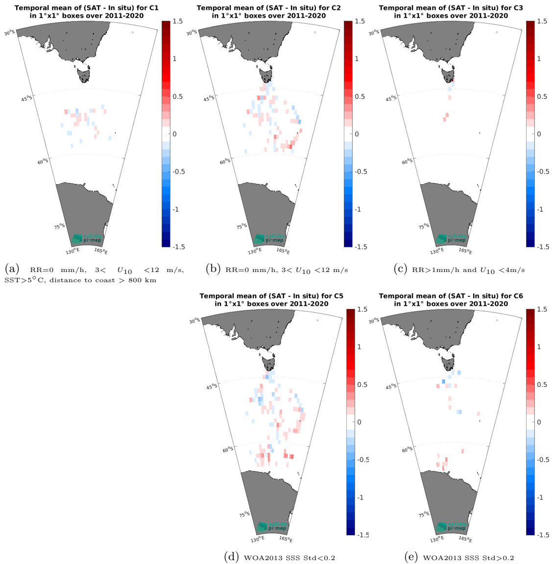
Figure 12: Temporal mean gridded over spatial boxes of size 1^\circ \times 1^\circ of \Delta SSS (SMAP SSS L4 OI v2 - 7 Days (ESR) - TSG (LEGOS-Survostral)) for 5 different subdatasets corresponding to:RR=0 mm/h, 3 < U_{10} < 12 m/s, SST>5°C, distance to coast > 800 km (a), RR=0 mm/h, 3 < U_{10} < 12 m/s (b), RR>1mm/h and U_{10} < 4 m/s (c), WOA2013 SSS Std<0.2 (d), WOA2013 SSS Std>0.2 (e).
