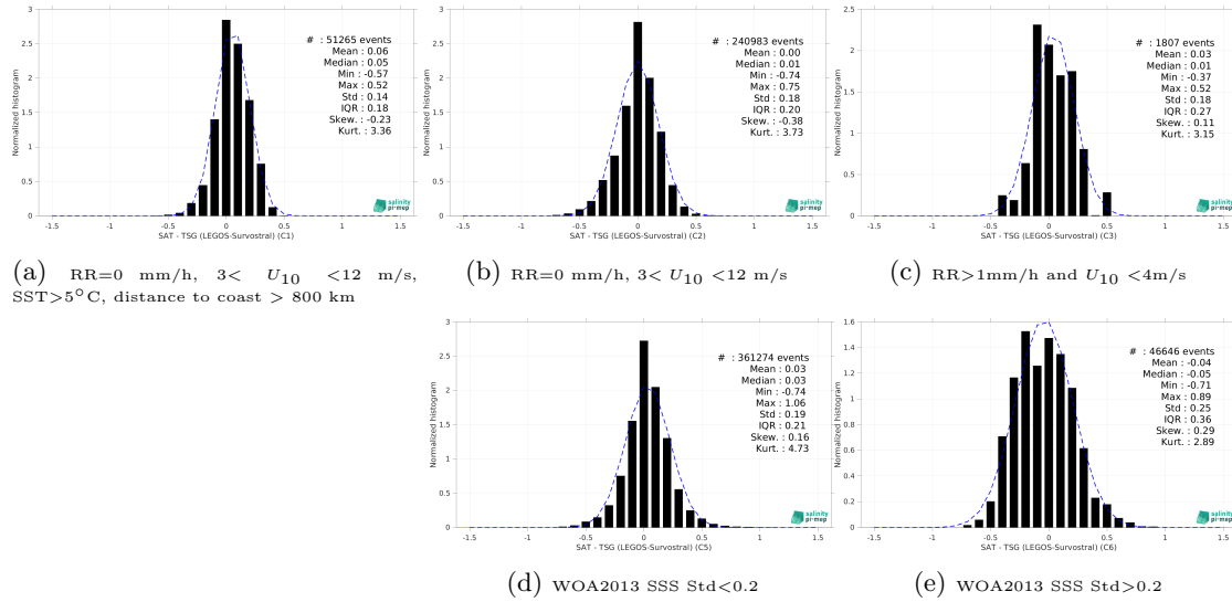
Figure 13: Normalized histogram of \Delta SSS (SMAP SSS L4 OI v2 - 7 Days (ESR) - TSG (LEGOS-Survostral)) for 5 different subdatasets corresponding to: RR=0 mm/h, 3 < U_{10} < 12 m/s, SST>5°C, distance to coast > 800 km (a), RR=0 mm/h, 3 < U_{10} < 12 m/s (b), RR>1mm/h and U_{10} < 4 m/s (c), WOA2013 SSS Std<0.2 (d), WOA2013 SSS Std>0.2 (e).
