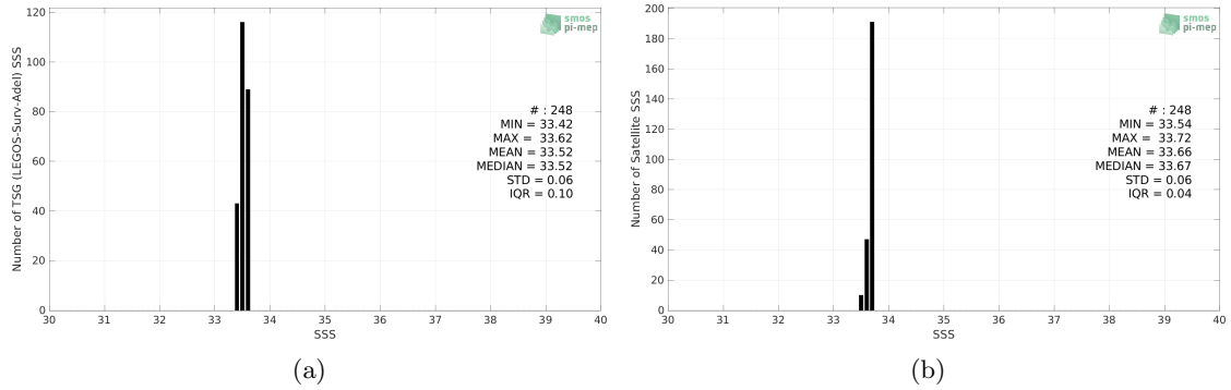
Figure 2: Histograms of SSS from TSG (LEGOS-Surv-Adel) (a) and SMAP SSS L4 OI v2 - 7 Days (ESR) (b) considering all match-up pairs per bins of 0.1 over the Global Ocean Pi-MEP region and for the full satellite product period.
