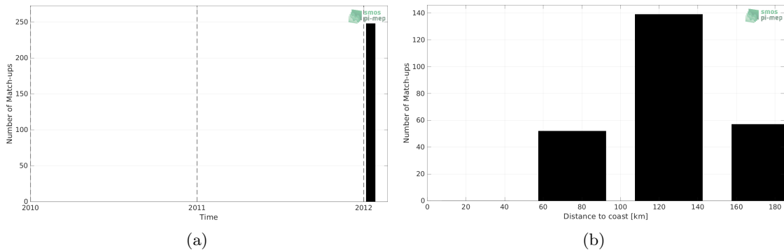
Figure 1: Number of match-ups between TSG (LEGOS-Surv-Adel) and SMAP SSS L4 OI v2 - 7 Days (ESR) SSS as a function of time (a) and as function of the distance to coast (b) over the Global Ocean Pi-MEP region and for the full satellite product period.
