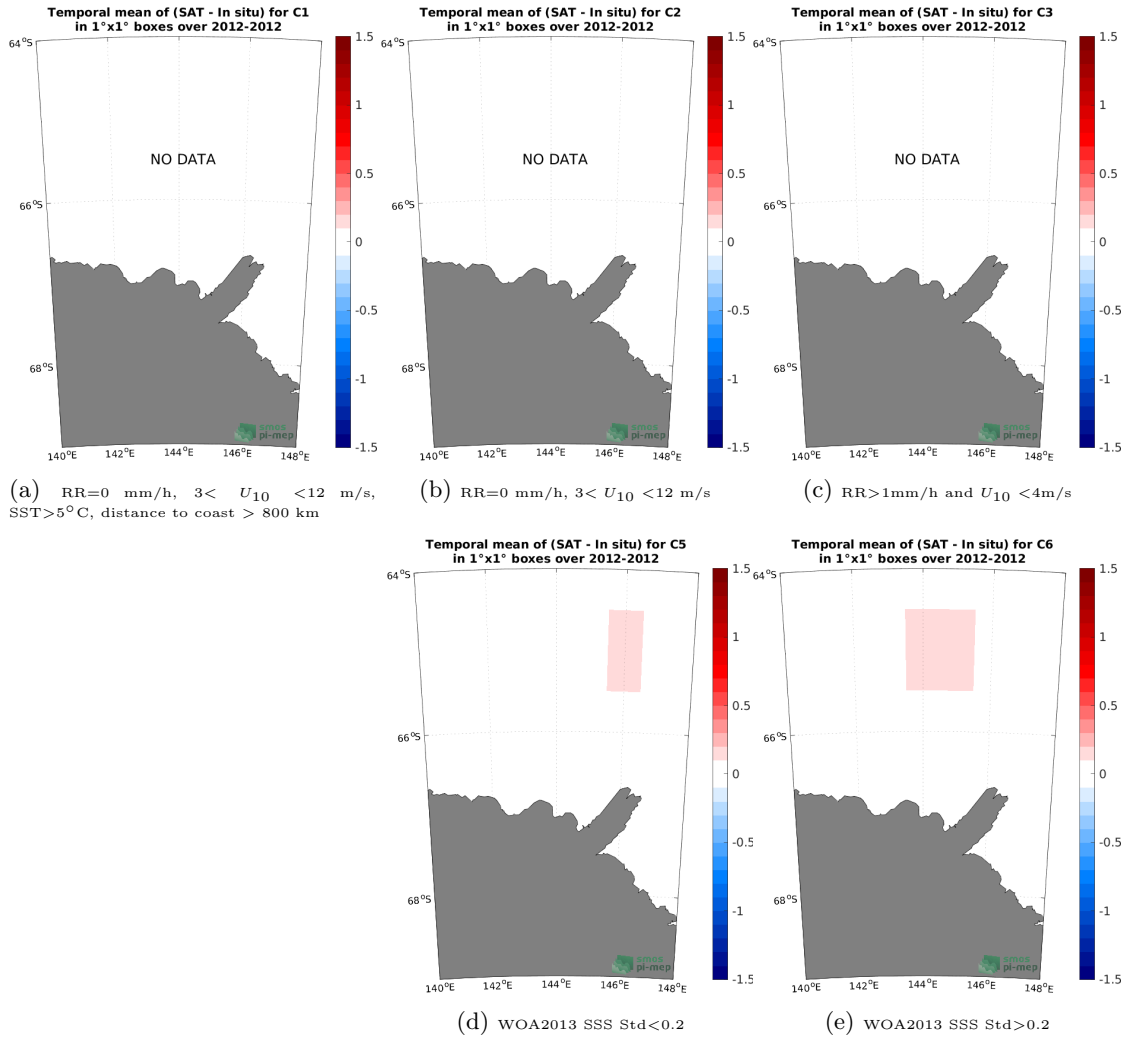
Figure 12: Temporal mean gridded over spatial boxes of size 1^\circ \times 1^\circ of \Delta SSS (SMAP SSS L4 OI v2 - 7 Days (ESR) - TSG (LEGOS-Surv-Adel)) for 5 different subdatasets corresponding to: RR=0 mm/h, 3 < U_{10} < 12 m/s, SST>5°C, distance to coast > 800 km (a), RR=0 mm/h, 3 < U_{10} < 12 m/s (b), RR>1mm/h and U_{10} < 4 m/s (c), WOA2013 SSS Std<0.2 (d), WOA2013 SSS Std>0.2 (e).
