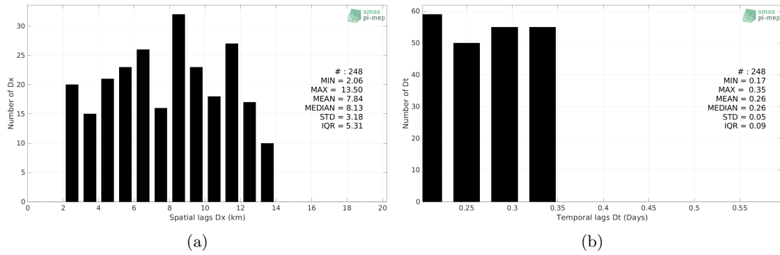
Figure 5: Histograms of the spatial (a) and temporal (b) lags between the location/time of the TSG (LEGOS-Surv-Adel) measurement and the date of the corresponding SMAP SSS L4 OI v2 - 7 Days (ESR) SSS pixel.
