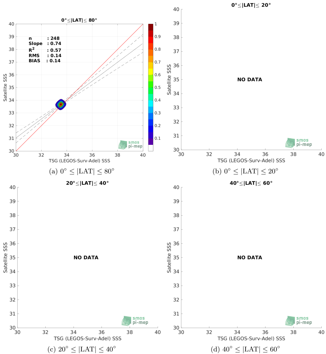
Figure 9: Contour maps of the concentration of SMAP SSS L4 OI v2 - 7 Days (ESR) SSS (y-axis) versus TSG (LEGOS-Surv-Adel) SSS (x-axis) at match-up pairs for different latitude bands. For each plot, the red line shows x=y . The black thin and dashed lines indicate a linear fit through the data cloud and the \pm 95\% confidence levels, respectively. The number match-up pairs n , the slope and R^2 coefficient of the linear fit, the root mean square (RMS) and the mean bias between satellite and in situ data are indicated for each latitude band in each plots.
