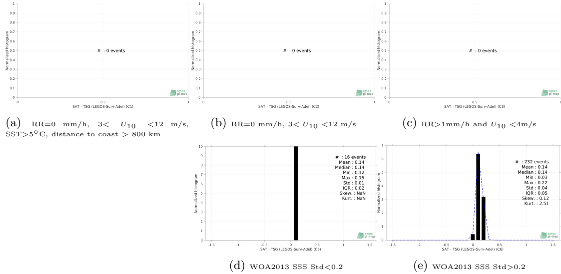
Figure 13: Normalized histogram of \Delta\text{SSS} (SMAP SSS L4 OI v2 - 7 Days (ESR) - TSG (LEGOS-Surv-Adel)) for 5 different subdatasets corresponding to: RR=0 mm/h, 3 < U_{10} < 12 m/s, SST > 5^\circ\text{C} , distance to coast > 800 km (a), RR=0 mm/h, 3 < U_{10} < 12 m/s (b), RR > 1\text{mm/h} and U_{10} < 4\text{m/s} (c), WOA2013 SSS \text{Std} < 0.2 (d), WOA2013 SSS \text{Std} > 0.2 (e).
