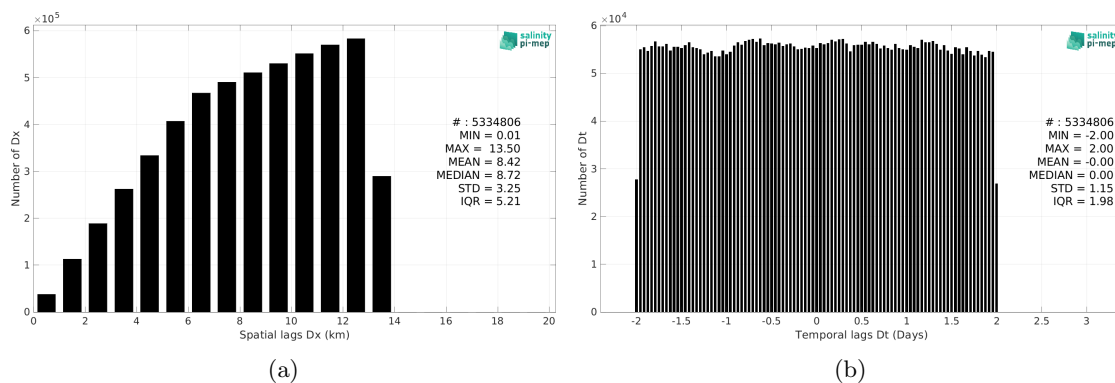
Figure 5: Histograms of the spatial (a) and temporal (b) lags between the location/time of the TSG (LEGOS-DM) measurement and the date of the corresponding SMAP SSS L4 OI v2 - 7 Days (ESR) SSS pixel.
