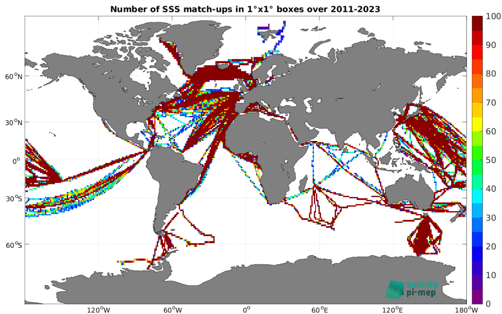
Figure 4: Number of SSS match-ups between TSG (LEGOS-DM) SSS and the SMAP SSS L4 OI v2 - 7 Days (ESR) SSS product for the Global Ocean Pi-MEP region over 1^\circ \times 1^\circ boxes and for the full satellite product period.
