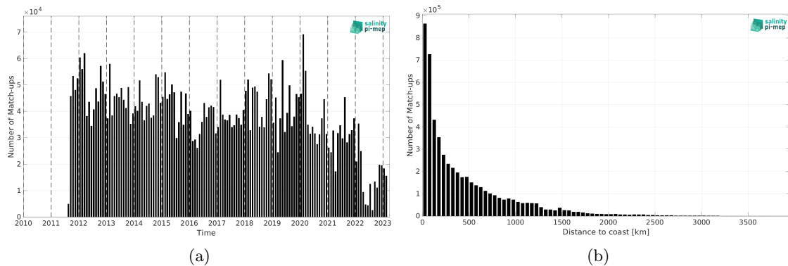
Figure 1: Number of match-ups between TSG (LEGOS-DM) and SMAP SSS L4 OI v2 - 7 Days (ESR) SSS as a function of time (a) and as function of the distance to coast (b) over the Global Ocean Pi-MEP region and for the full satellite product period.
