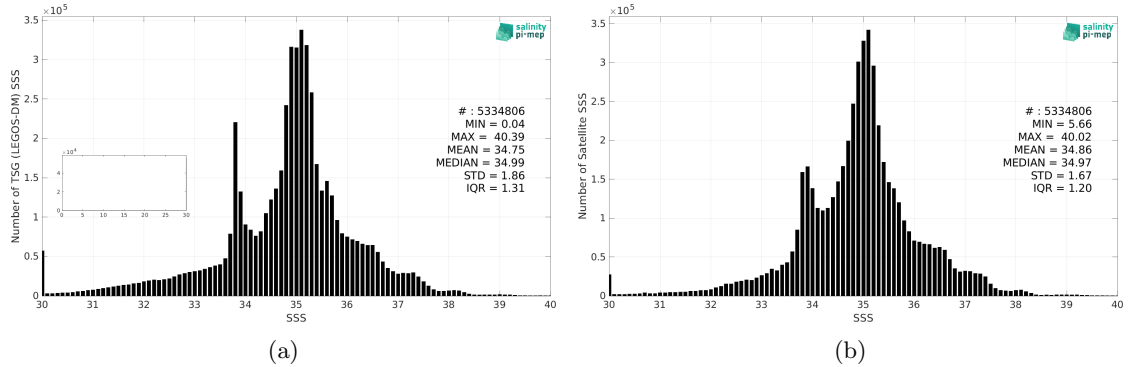
Figure 2: Histograms of SSS from TSG (LEGOS-DM) (a) and SMAP SSS L4 OI v2 - 7 Days (ESR) (b) considering all match-up pairs per bins of 0.1 over the Global Ocean Pi-MEP region and for the full satellite product period.
