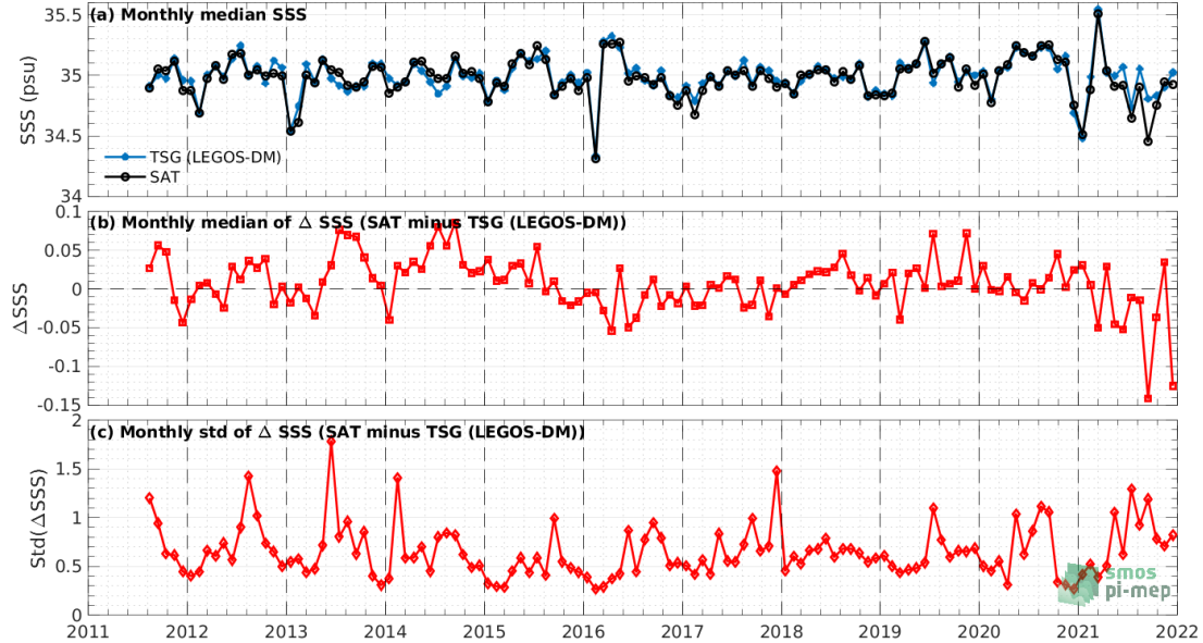
Figure 7: Time series of the monthly median SSS (top), median of \Delta SSS (Satellite - TSG (LEGOS-DM)) and Std of \Delta SSS (Satellite - TSG (LEGOS-DM)) over the Global Ocean Pi-MEP region considering all match-ups collected by the Pi-MEP.
