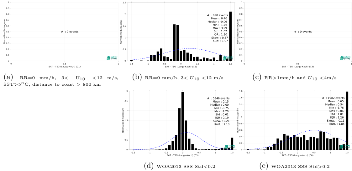
Figure 13: Normalized histogram of \Delta SSS (SMAP SSS L4 OI v2 - 7 Days (ESR) - TSG (Lauge-Koch)) for 5 different subdatasets corresponding to: RR=0 mm/h, 3 < U_{10} < 12 m/s, SST > 5°C, distance to coast > 800 km (a), RR=0 mm/h, 3 < U_{10} < 12 m/s (b), RR > 1mm/h and U_{10} < 4 m/s (c), WOA2013 SSS Std < 0.2 (d), WOA2013 SSS Std > 0.2 (e).
