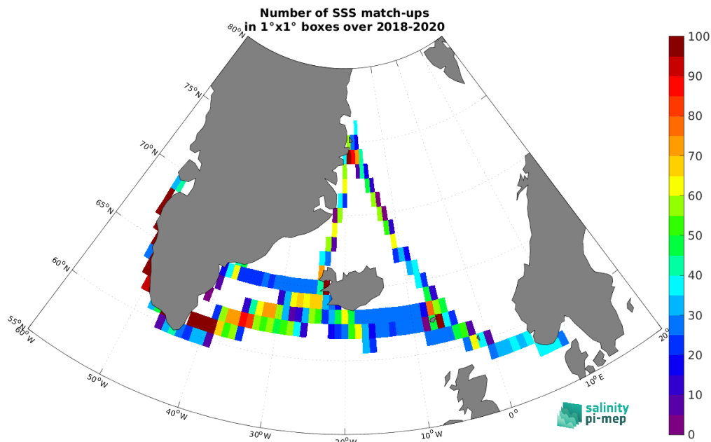
Figure 4: Number of SSS match-ups between TSG (Lauge-Koch) SSS and the SMAP SSS L4 OI v2 - 7 Days (ESR) SSS product for the Global Ocean Pi-MEP region over 1^\circ \times 1^\circ boxes and for the full satellite product period.
