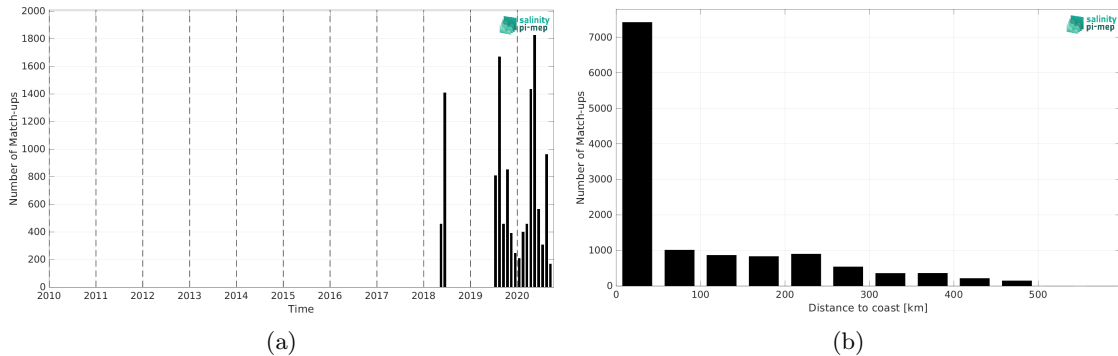
Figure 1: Number of match-ups between TSG (Lauge-Koch) and SMAP SSS L4 OI v2 - 7 Days (ESR) SSS as a function of time (a) and as function of the distance to coast (b) over the Global Ocean Pi-MEP region and for the full satellite product period.
