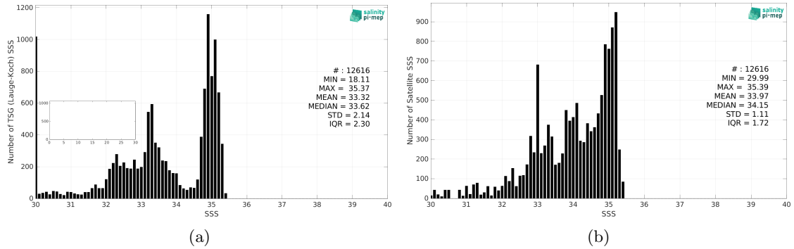
Figure 2: Histograms of SSS from TSG (Lauge-Koch) (a) and SMAP SSS L4 OI v2 - 7 Days (ESR) (b) considering all match-up pairs per bins of 0.1 over the Global Ocean Pi-MEP region and for the full satellite product period.
