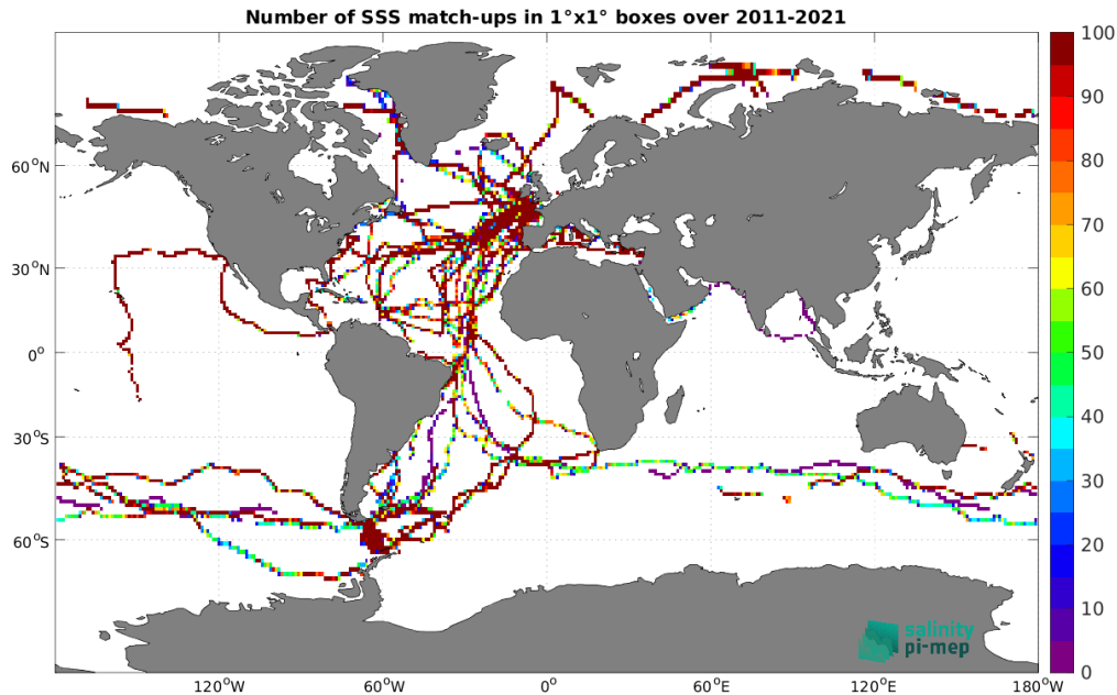
Figure 4: Number of SSS match-ups between TSG (GOSUD-Sailing-ship) SSS and the SMAP SSS L4 OI v2 - 7 Days (ESR) SSS product for the Global Ocean Pi-MEP region over 1^\circ \times 1^\circ boxes and for the full satellite product period.
