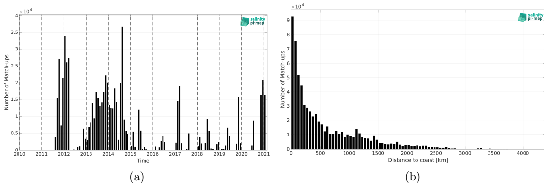
Figure 1: Number of match-ups between TSG (GOSUD-Sailing-ship) and SMAP SSS L4 OI v2 - 7 Days (ESR) SSS as a function of time (a) and as function of the distance to coast (b) over the Global Ocean Pi-MEP region and for the full satellite product period.
