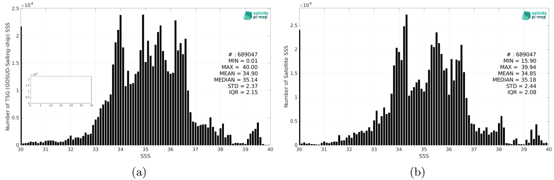
Figure 2: Histograms of SSS from TSG (GOSUD-Sailing-ship) (a) and SMAP SSS L4 OI v2 - 7 Days (ESR) (b) considering all match-up pairs per bins of 0.1 over the Global Ocean Pi-MEP region and for the full satellite product period.
