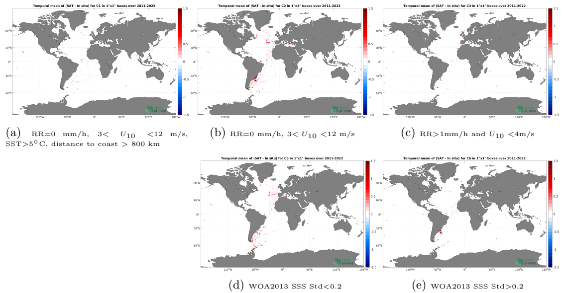
Figure 12: Temporal mean gridded over spatial boxes of size 1^\circ \times 1^\circ of \Delta SSS (SMAP SSS L4 OI v2 - 7 Days (ESR) - TSG (CSIC-UTM)) for 5 different subdatasets corresponding to:RR=0 mm/h, 3 < U_{10} < 12 m/s, SST >5^\circ C, distance to coast > 800 km (a), RR=0 mm/h, 3 < U_{10} < 12 m/s (b), RR >1 mm/h and U_{10} < 4 m/s (c), WOA2013 SSS Std <0.2 (d), WOA2013 SSS Std >0.2 (e).
