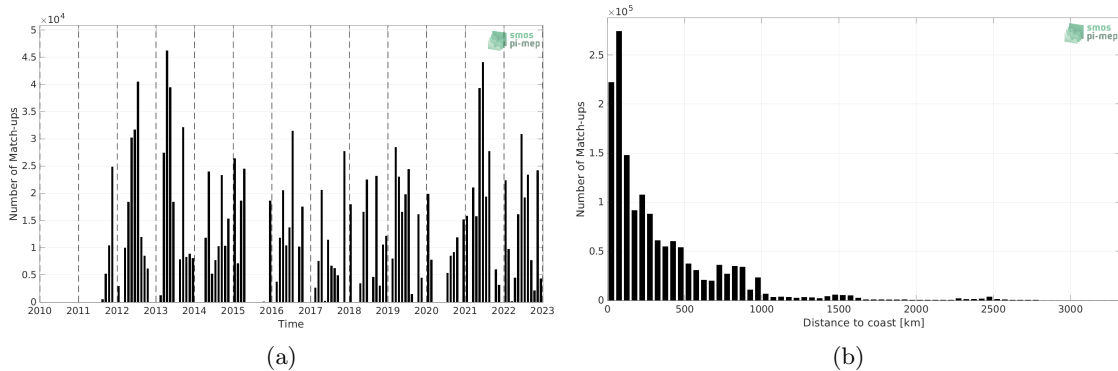
Figure 1: Number of match-ups between TSG (CSIC-UTM) and SMAP SSS L4 OI v2 - 7 Days (ESR) SSS as a function of time (a) and as function of the distance to coast (b) over the Global Ocean Pi-MEP region and for the full satellite product period.
