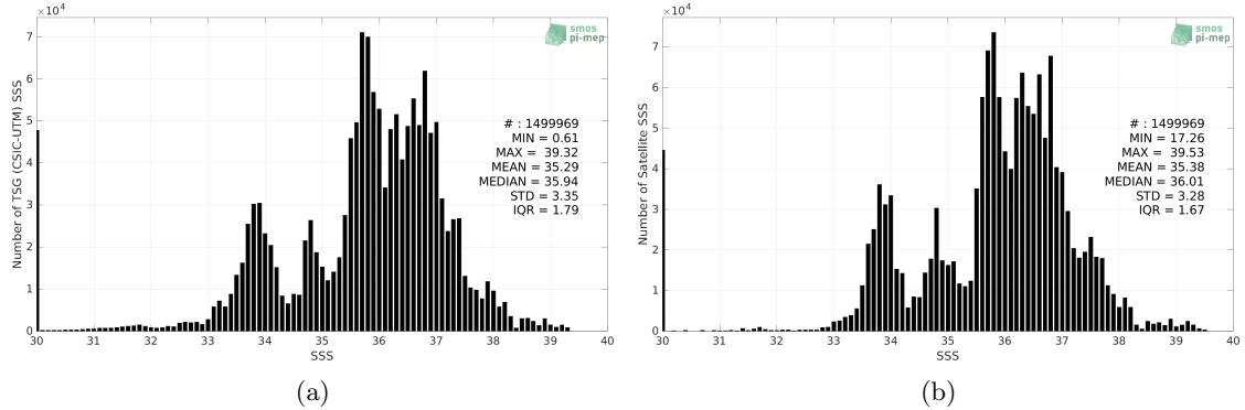
Figure 2: Histograms of SSS from TSG (CSIC-UTM) (a) and SMAP SSS L4 OI v2 - 7 Days (ESR) (b) considering all match-up pairs per bins of 0.1 over the Global Ocean Pi-MEP region and for the full satellite product period.
