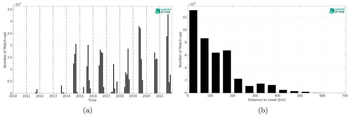
Figure 1: Number of match-ups between TSG (Amundsen) and SMAP SSS L4 OI v2 - 7 Days (ESR) SSS as a function of time (a) and as function of the distance to coast (b) over the Global Ocean Pi-MEP region and for the full satellite product period.
