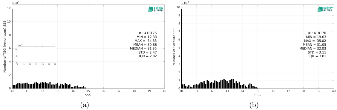
Figure 2: Histograms of SSS from TSG (Amundsen) (a) and SMAP SSS L4 OI v2 - 7 Days (ESR) (b) considering all match-up pairs per bins of 0.1 over the Global Ocean Pi-MEP region and for the full satellite product period.
