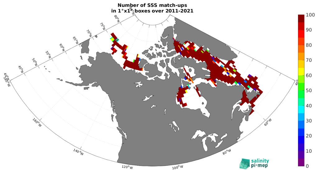
Figure 4: Number of SSS match-ups between TSG (Amundsen) SSS and the SMAP SSS L4 OI v2 - 7 Days (ESR) SSS product for the Global Ocean Pi-MEP region over 1^\circ \times 1^\circ boxes and for the full satellite product period.
