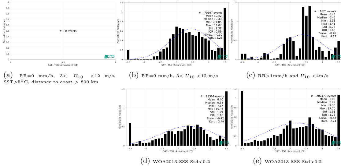
Figure 13: Normalized histogram of \Delta SSS (SMAP SSS L4 OI v2 - 7 Days (ESR) - TSG (Amundsen)) for 5 different subdatasets corresponding to: RR=0 mm/h, 3 < U_{10} < 12 m/s, SST > 5°C, distance to coast > 800 km (a), RR=0 mm/h, 3 < U_{10} < 12 m/s (b), RR > 1mm/h and U_{10} < 4 m/s (c), WOA2013 SSS Std < 0.2 (d), WOA2013 SSS Std > 0.2 (e).
