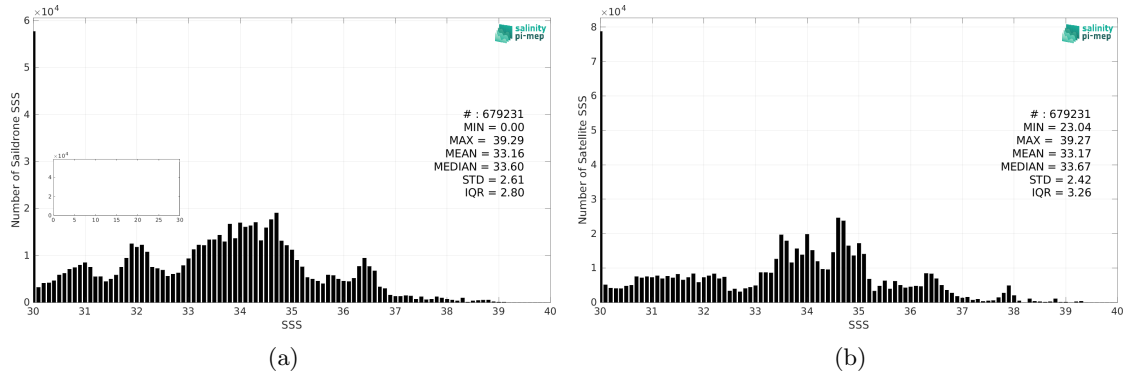
Figure 2: Histograms of SSS from Saildrone (a) and SMAP SSS L4 OI v2 - 7 Days (ESR) (b) considering all match-up pairs per bins of 0.1 over the Global Ocean Pi-MEP region and for the full satellite product period.
