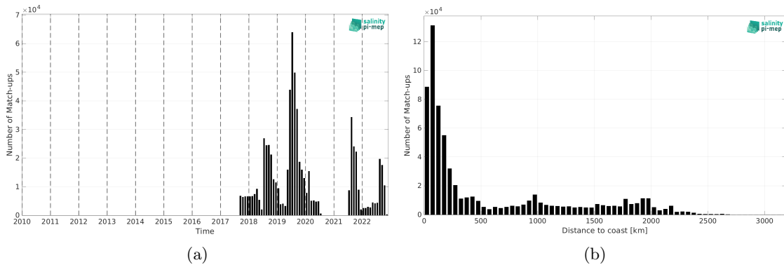
Figure 1: Number of match-ups between Saildrone and SMAP SSS L4 OI v2 - 7 Days (ESR) SSS as a function of time (a) and as function of the distance to coast (b) over the Global Ocean Pi-MEP region and for the full satellite product period.
