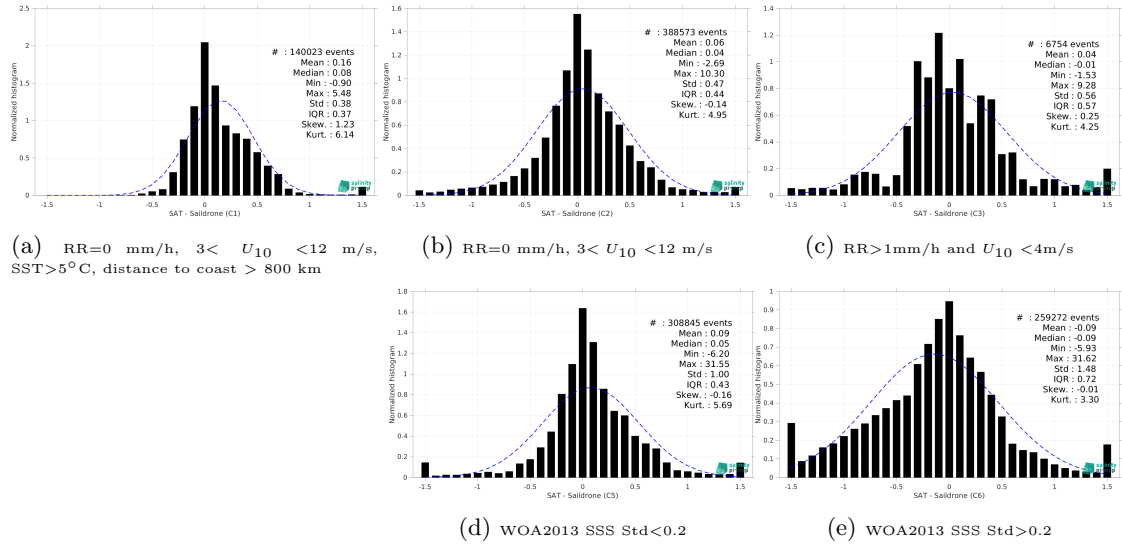
Figure 13: Normalized histogram of \Delta\text{SSS} (SMAP SSS L4 OI v2 - 7 Days (ESR) - SAILDRONE) for 5 different subdatasets corresponding to: RR=0 mm/h, 3 < U_{10} < 12 m/s, SST > 5°C, distance to coast > 800 km (a), RR=0 mm/h, 3 < U_{10} < 12 m/s (b), RR > 1mm/h and U_{10} < 4 m/s (c), WOA2013 SSS Std < 0.2 (d), WOA2013 SSS Std > 0.2 (e).
