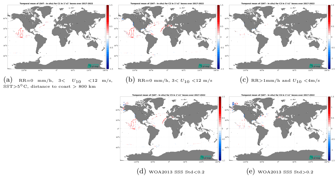
Figure 12: Temporal mean gridded over spatial boxes of size 1^\circ \times 1^\circ of \Delta SSS (SMAP SSS L4 OI v2 - 7 Days (ESR) - Saildrone) for 5 different subdatasets corresponding to:RR=0 mm/h, 3 < U_{10} < 12 m/s, SST > 5^\circ\text{C} , distance to coast > 800 km (a), RR=0 mm/h, 3 < U_{10} < 12 m/s (b), RR > 1 mm/h and U_{10} < 4 m/s (c), WOA2013 SSS Std < 0.2 (d), WOA2013 SSS Std > 0.2 (e).
