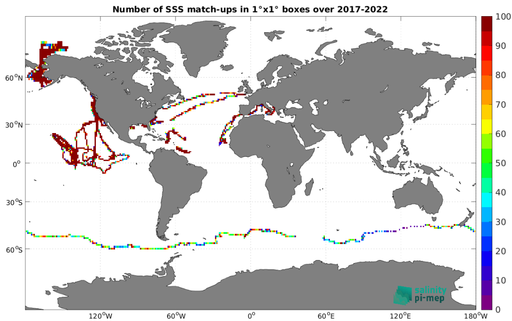
Figure 4: Number of SSS match-ups between Saildrone SSS and the SMAP SSS L4 OI v2 - 7 Days (ESR) SSS product for the Global Ocean Pi-MEP region over 1^\circ \times 1^\circ boxes and for the full satellite product period.
