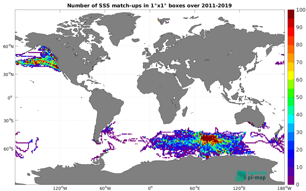
Figure 4: Number of SSS match-ups between Marine mammals SSS and the SMAP SSS L4 OI v2 - 7 Days (ESR) SSS product for the Global Ocean Pi-MEP region over 1^\circ \times 1^\circ boxes and for the full satellite product period.
