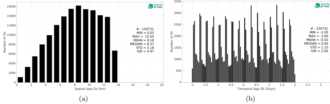
Figure 5: Histograms of the spatial (a) and temporal (b) lags between the location/time of the Marine mammals measurement and the date of the corresponding SMAP SSS L4 OI v2 - 7 Days (ESR) SSS pixel.
