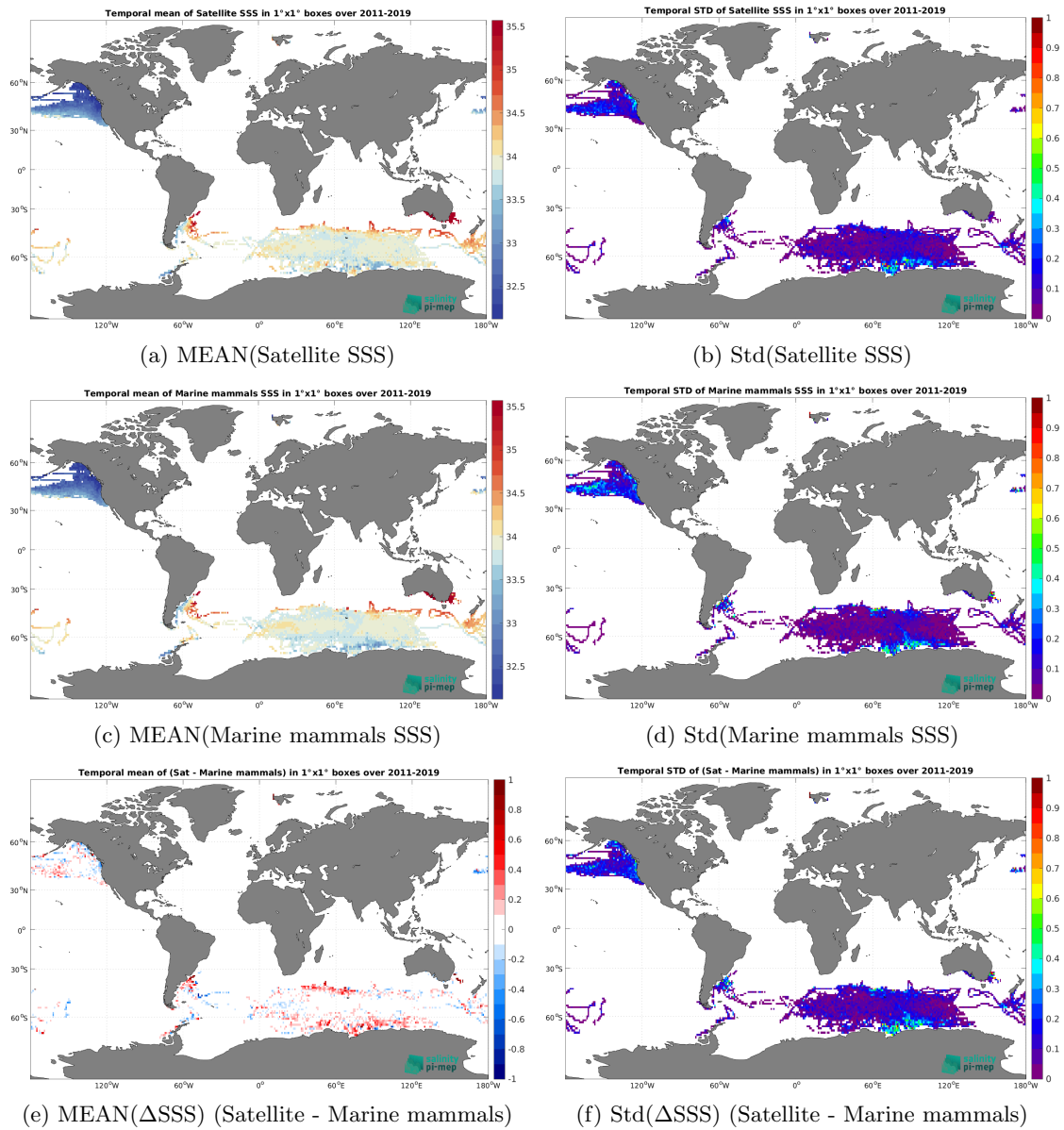
Figure 6: Temporal mean (left) and Std (right) of SSS from SMAP SSS L4 OI v2 - 7 Days (ESR) (top), Marine mammals (middle), and of \Delta SSS (Satellite - Marine mammals). Only match-up pairs are used to generate these maps.
