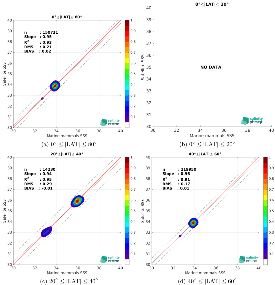
Figure 9: Contour maps of the concentration of SMAP SSS L4 OI v2 - 7 Days (ESR) SSS (y-axis) versus Marine mammals SSS (x-axis) at match-up pairs for different latitude bands. For each plot, the red line shows x=y . The black thin and dashed lines indicate a linear fit through the data cloud and the \pm 95\% confidence levels, respectively. The number match-up pairs n , the slope and R^2 coefficient of the linear fit, the root mean square (RMS) and the mean bias between satellite and in situ data are indicated for each latitude band in each plots.
