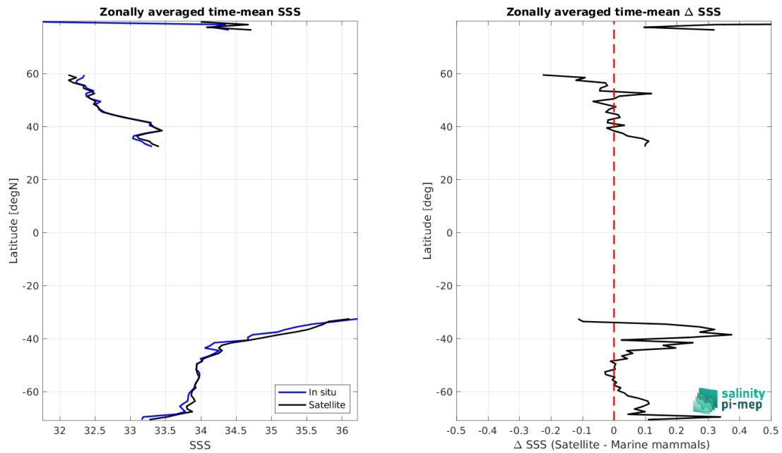
Figure 8: Left panel: Zonal mean SSS from SMAP SSS L4 OI v2 - 7 Days (ESR) satellite product (black) and from Marine mammals (blue). Right panel: Zonal mean of \Delta SSS (Satellite - Marine mammals) for all the collected Pi-MEP match-up pairs estimated over the full satellite product period.
