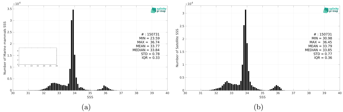
Figure 2: Histograms of SSS from Marine mammals (a) and SMAP SSS L4 OI v2 - 7 Days (ESR) (b) considering all match-up pairs per bins of 0.1 over the Global Ocean Pi-MEP region and for the full satellite product period.
