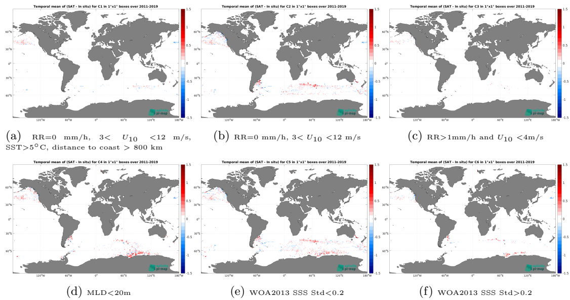
Figure 12: Temporal mean gridded over spatial boxes of size 1^\circ \times 1^\circ of \Delta SSS (SMAP SSS L4 OI v2 - 7 Days (ESR) - Marine mammals) for 6 different subdatasets corresponding to:RR=0 mm/h, 3 < U_{10} < 12 m/s, SST >5^\circ C, distance to coast > 800 km (a), RR=0 mm/h, 3 < U_{10} < 12 m/s (b), RR >1 mm/h and U_{10} < 4 m/s (c),MLD <20 m (d),WOA2013 SSS Std <0.2 (e),WOA2013 SSS Std >0.2 (f).
