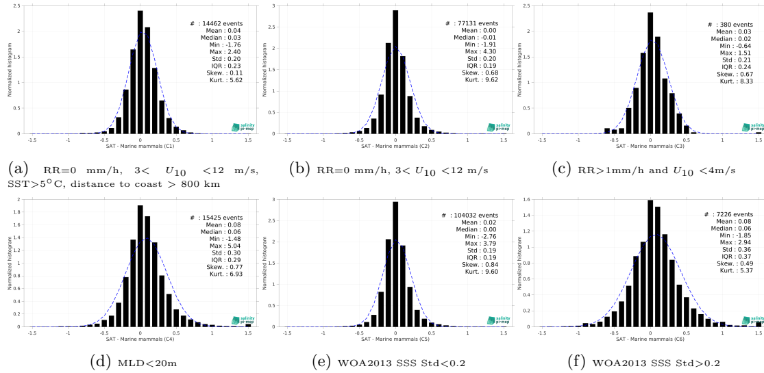
Figure 13: Normalized histogram of \Delta SSS (SMAP SSS L4 OI v2 - 7 Days (ESR) - Marine mammals) for 6 different subdatasets corresponding to: RR=0 mm/h, 3 < U_{10} < 12 m/s, SST > 5°C, distance to coast > 800 km (a), RR=0 mm/h, 3 < U_{10} < 12 m/s (b), RR > 1mm/h and U_{10} < 4 m/s (c), MLD < 20m (d), WOA2013 SSS Std < 0.2 (e), WOA2013 SSS Std > 0.2 (f).
