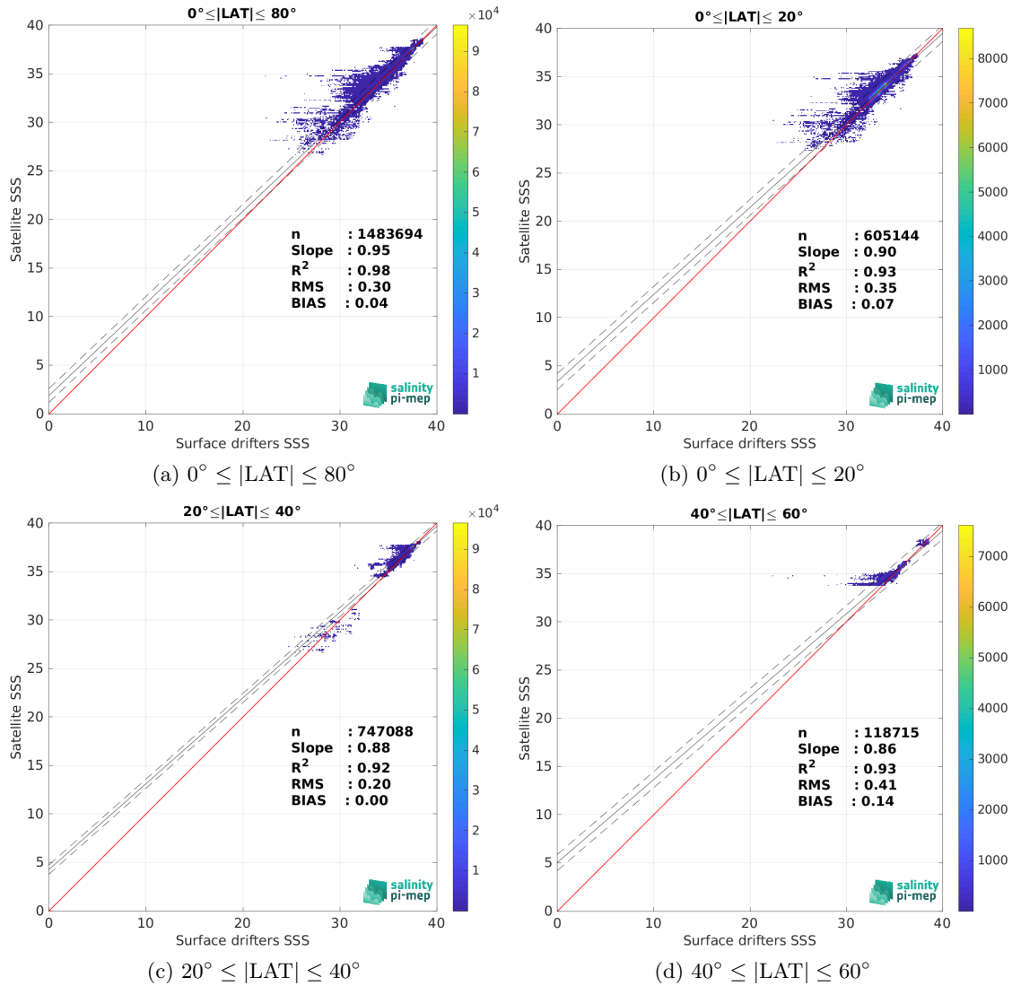
Figure 8: Contour maps of the concentration of SMAP SSS L4 OI v2 - 7 Days (ESR) SSS (y-axis) versus Surface drifters SSS (x-axis) at match-up pairs for different latitude bands. For each plot, the red line shows x=y . The black thin and dashed lines indicate a linear fit through the data cloud and the \pm 95\% confidence levels, respectively. The number match-up pairs n , the slope and R^2 coefficient of the linear fit, the root mean square (RMS) and the mean bias between satellite and in situ data are indicated for each latitude band in each plots.
