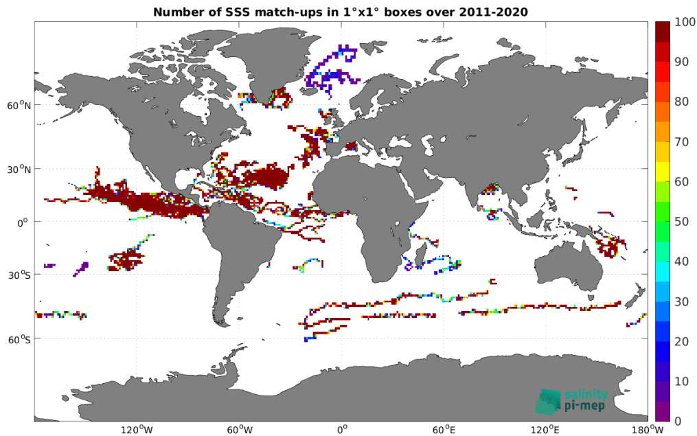
Figure 3: Number of SSS match-ups between Surface drifters SSS and the SMAP SSS L4 OI v2 - 7 Days (ESR) SSS product for the Global Ocean Pi-MEP region over 1^\circ \times 1^\circ boxes and for the full satellite product period.
