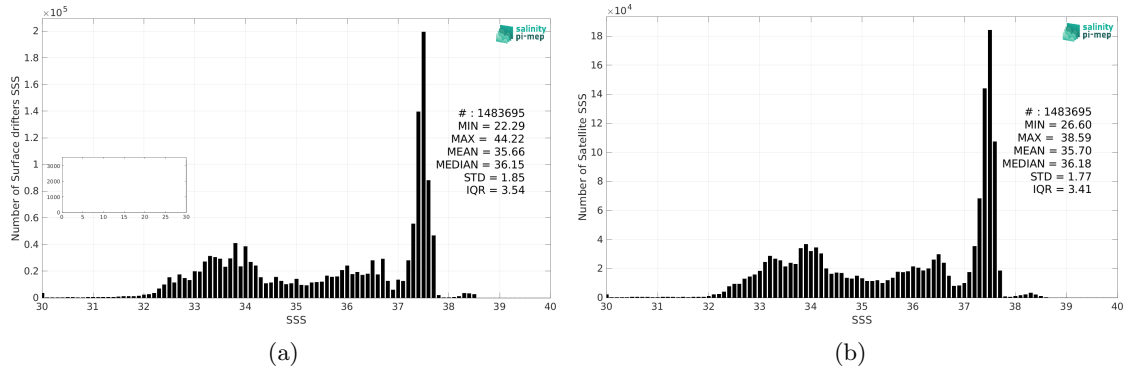
Figure 2: Histograms of SSS from Surface drifters (a) and SMAP SSS L4 OI v2 - 7 Days (ESR) (b) considering all match-up pairs per bins of 0.1 over the Global Ocean Pi-MEP region and for the full satellite product period.
