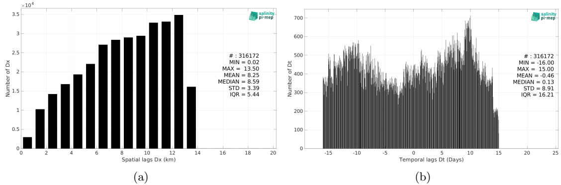
Figure 5: Histograms of the spatial (a) and temporal (b) lags between the location/time of the TSG (Polarstern) measurement and the date of the corresponding SMAP SSS L4 OI v2 - Monthly (IPRC) SSS pixel.
