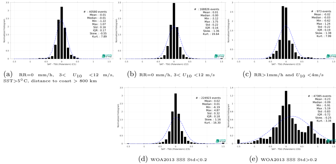
Figure 13: Normalized histogram of \Delta SSS (SMAP SSS L4 OI v2 - Monthly (IPRC) - TSG (Polarstern)) for 5 different subdatasets corresponding to: RR=0 mm/h, 3 < U_{10} < 12 m/s, SST > 5°C, distance to coast > 800 km (a), RR=0 mm/h, 3 < U_{10} < 12 m/s (b), RR > 1mm/h and U_{10} < 4 m/s (c), WOA2013 SSS Std < 0.2 (d), WOA2013 SSS Std > 0.2 (e).
