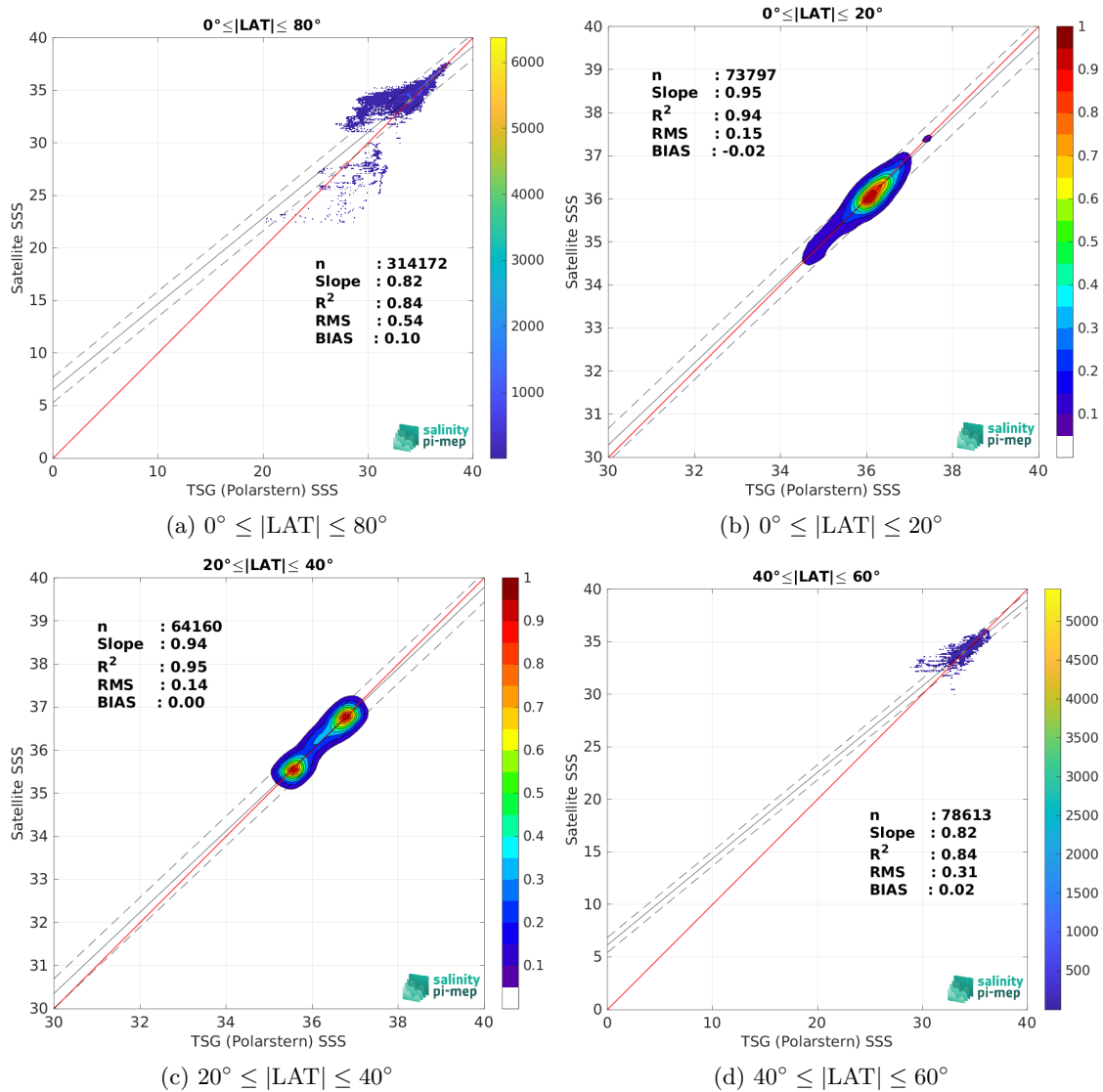
Figure 9: Contour maps of the concentration of SMAP SSS L4 OI v2 - Monthly (IPRC) SSS (y-axis) versus TSG (Polarstern) SSS (x-axis) at match-up pairs for different latitude bands. For each plot, the red line shows x=y . The black thin and dashed lines indicate a linear fit through the data cloud and the \pm 95\% confidence levels, respectively. The number match-up pairs n , the slope and R^2 coefficient of the linear fit, the root mean square (RMS) and the mean bias between satellite and in situ data are indicated for each latitude band in each plots.
