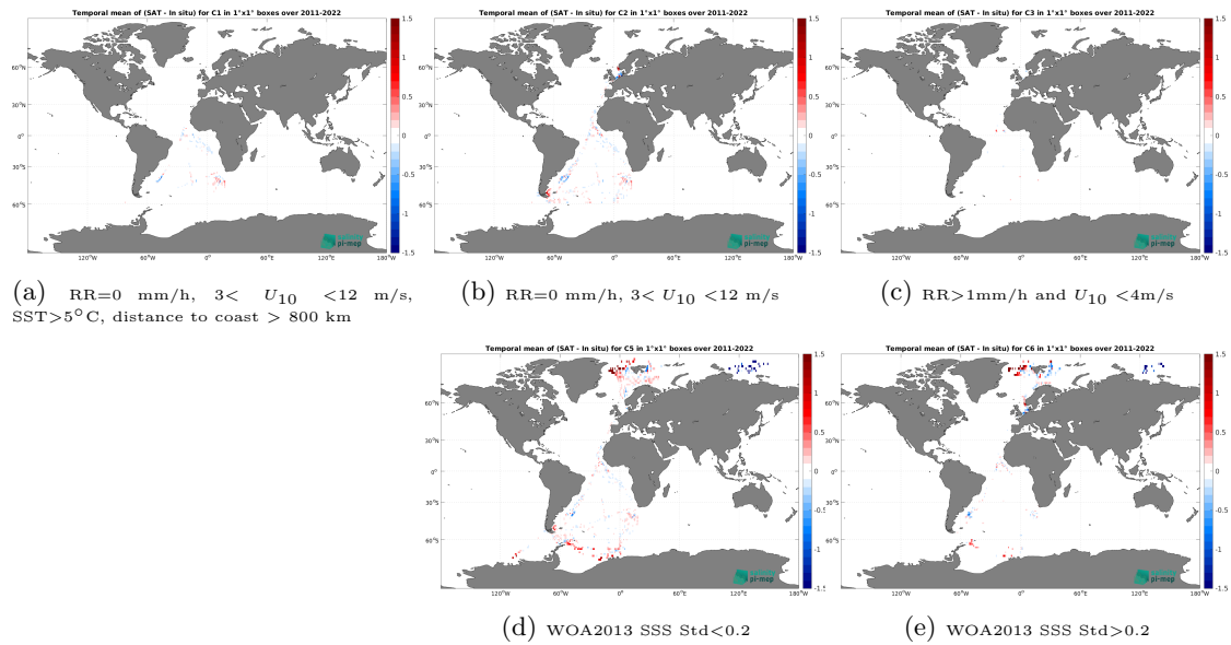
Figure 12: Temporal mean gridded over spatial boxes of size 1^\circ \times 1^\circ of \Delta SSS (SMAP SSS L4 OI v2 - Monthly (IPRC) - TSG (Polarstern)) for 5 different subdatasets corresponding to:RR=0 mm/h, 3 < U_{10} < 12 m/s, SST > 5^\circ\text{C} , distance to coast > 800 km (a), RR=0 mm/h, 3 < U_{10} < 12 m/s (b), RR > 1 mm/h and U_{10} < 4 m/s (c), WOA2013 SSS Std < 0.2 (d), WOA2013 SSS Std > 0.2 (e).
