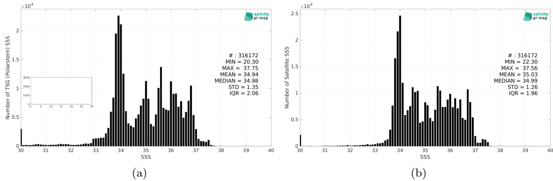
Figure 2: Histograms of SSS from TSG (Polarstern) (a) and SMAP SSS L4 OI v2 - Monthly (IPRC) (b) considering all match-up pairs per bins of 0.1 over the Global Ocean Pi-MEP region and for the full satellite product period.
