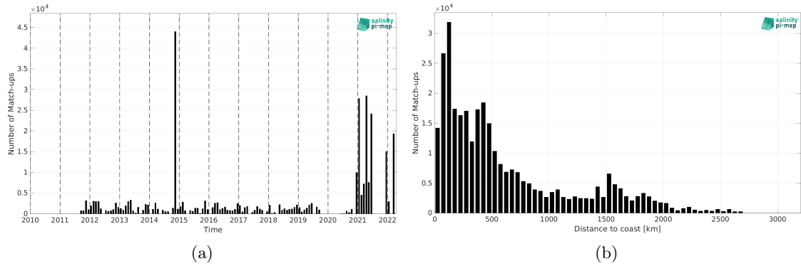
Figure 1: Number of match-ups between TSG (Polarstern) and SMAP SSS L4 OI v2 - Monthly (IPRC) SSS as a function of time (a) and as function of the distance to coast (b) over the Global Ocean Pi-MEP region and for the full satellite product period.
