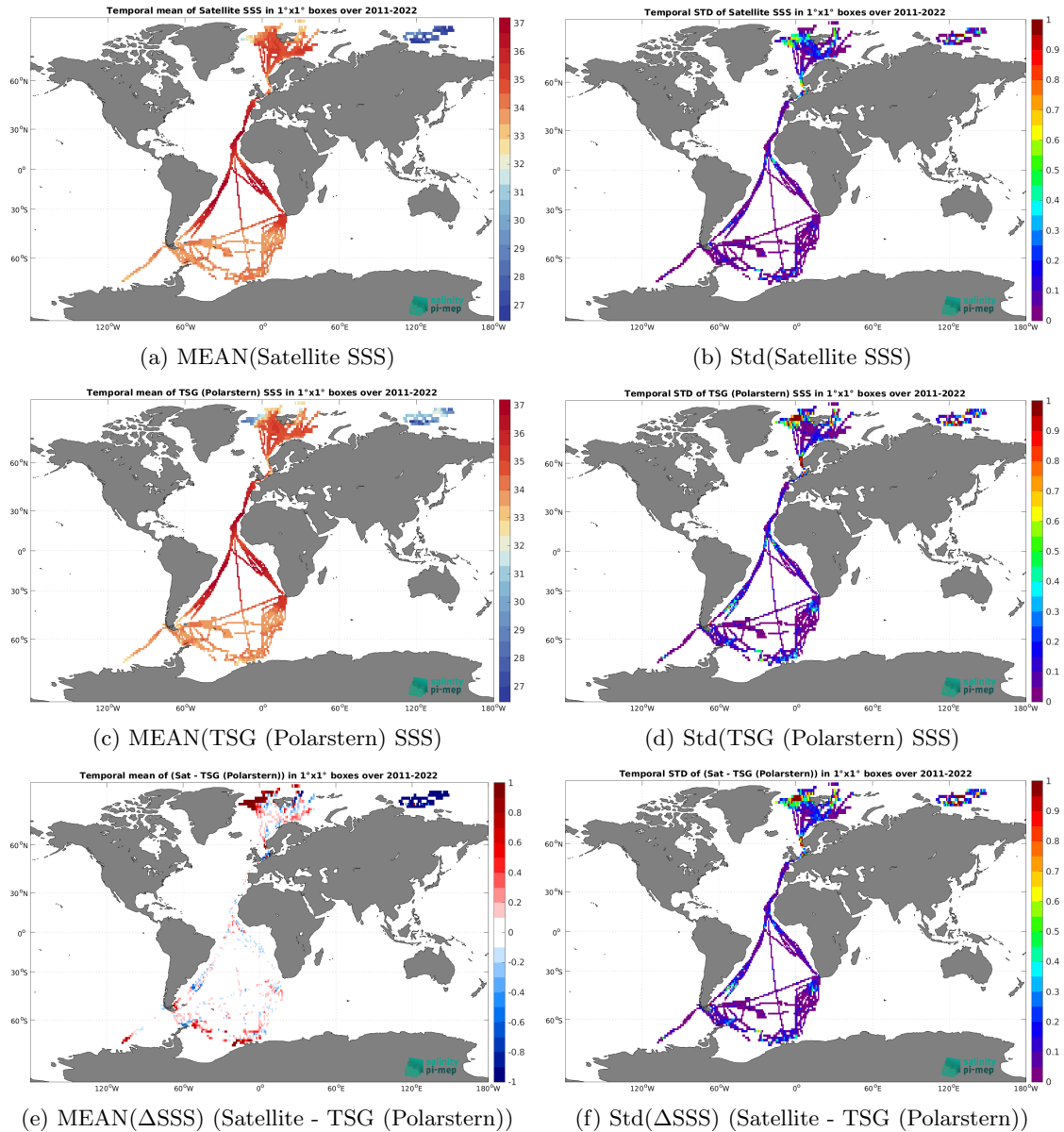
Figure 6: Temporal mean (left) and Std (right) of SSS from SMAP SSS L4 OI v2 - Monthly (IPRC) (top), TSG (Polarstern) (middle), and of \Delta SSS (Satellite - TSG (Polarstern)). Only match-up pairs are used to generate these maps.
