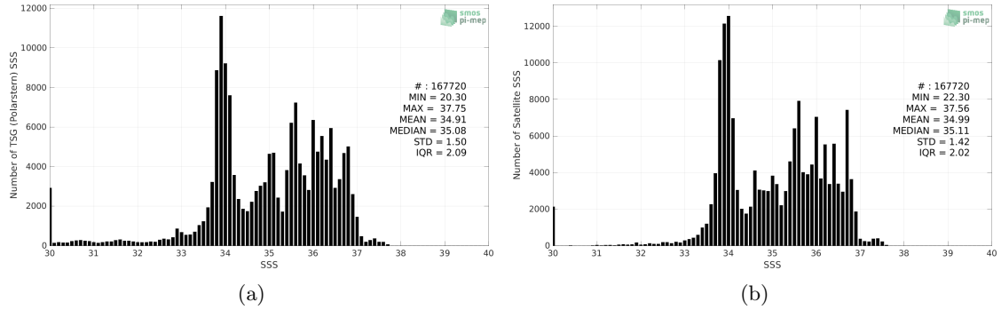
Figure 2: Histograms of SSS from TSG (Polarstern) (a) and SMAP SSS L4 OI v2 - Monthly (IPRC) (b) considering all match-up pairs per bins of 0.1 over the Global Ocean Pi-MEP region and for the full satellite product period.
