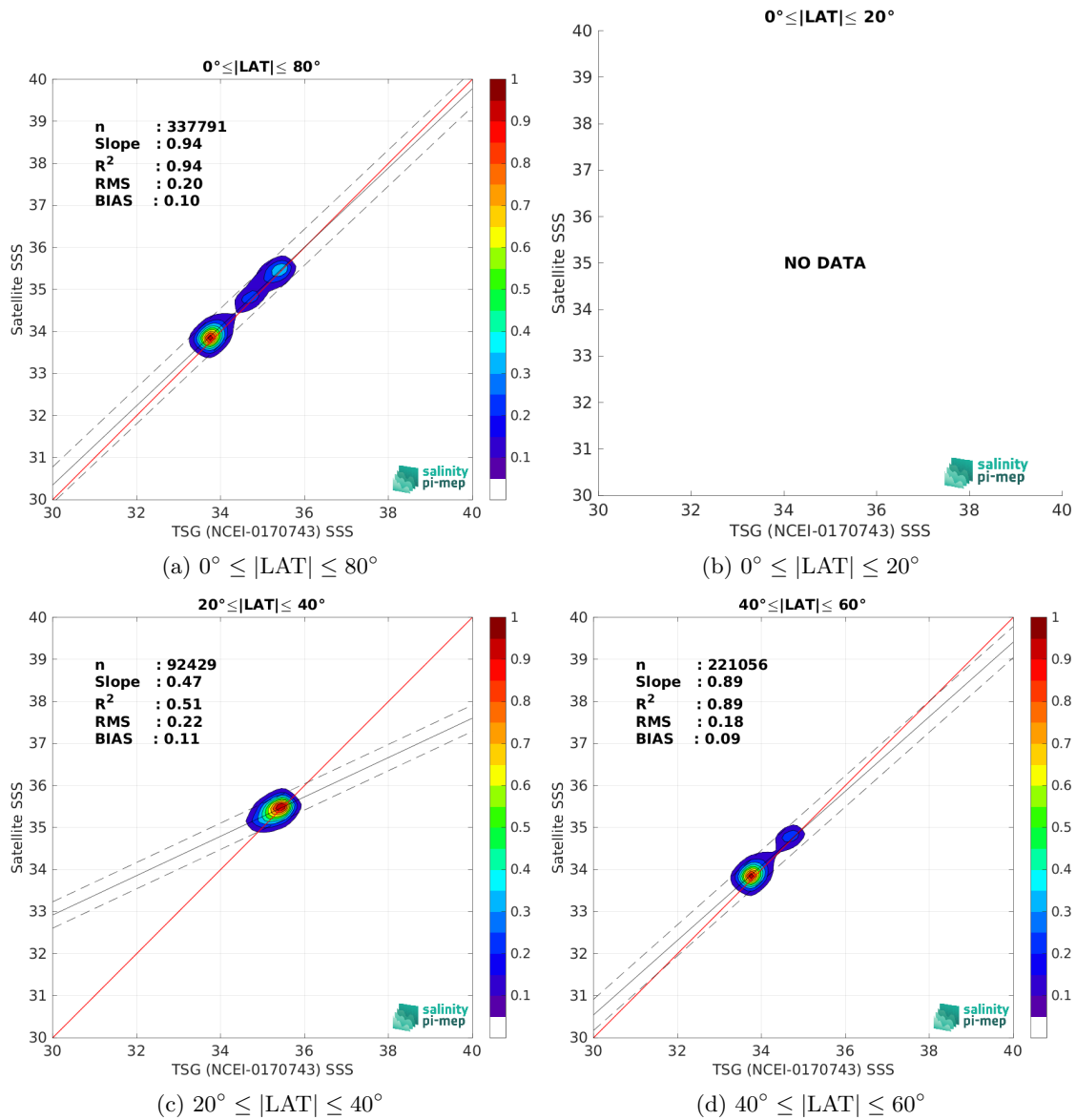
Figure 9: Contour maps of the concentration of SMAP SSS L4 OI v2 - Monthly (IPRC) SSS (y-axis) versus TSG (NCEI-0170743) SSS (x-axis) at match-up pairs for different latitude bands. For each plot, the red line shows x=y . The black thin and dashed lines indicate a linear fit through the data cloud and the \pm 95\% confidence levels, respectively. The number match-up pairs n , the slope and R^2 coefficient of the linear fit, the root mean square (RMS) and the mean bias between satellite and in situ data are indicated for each latitude band in each plots.
