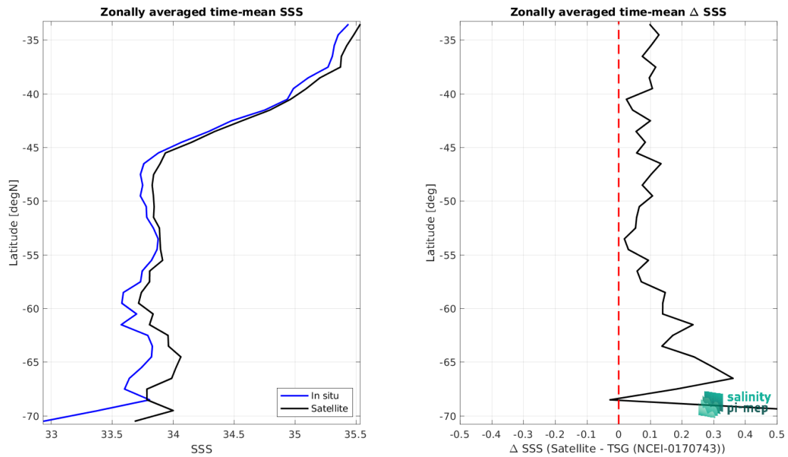
Figure 8: Left panel: Zonal mean SSS from SMAP SSS L4 OI v2 - Monthly (IPRC) satellite product (black) and from TSG (NCEI-0170743) (blue). Right panel: Zonal mean of \Delta SSS (Satellite - TSG (NCEI-0170743)) for all the collected Pi-MEP match-up pairs estimated over the full satellite product period.
