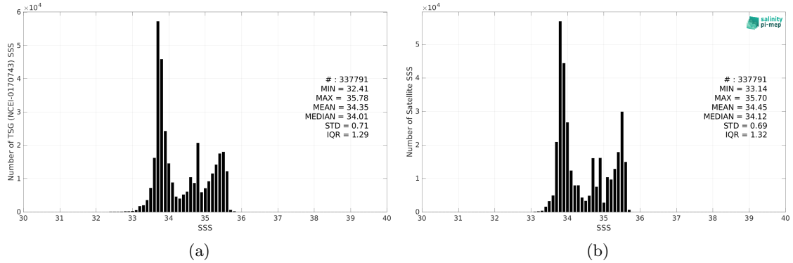
Figure 2: Histograms of SSS from TSG (NCEI-0170743) (a) and SMAP SSS L4 OI v2 - Monthly (IPRC) (b) considering all match-up pairs per bins of 0.1 over the Global Ocean Pi-MEP region and for the full satellite product period.
