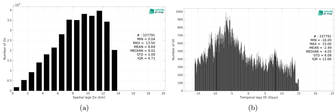
Figure 5: Histograms of the spatial (a) and temporal (b) lags between the location/time of the TSG (NCEI-0170743) measurement and the date of the corresponding SMAP SSS L4 OI v2 - Monthly (IPRC) SSS pixel.
