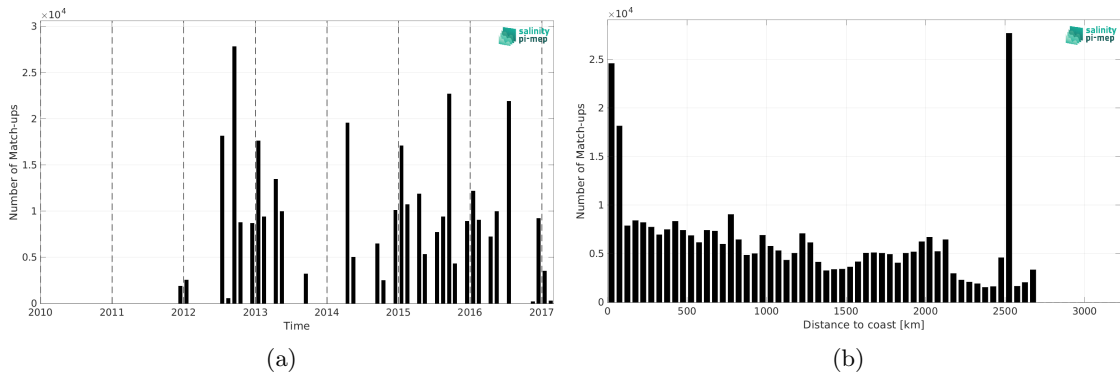
Figure 1: Number of match-ups between TSG (NCEI-0170743) and SMAP SSS L4 OI v2 - Monthly (IPRC) SSS as a function of time (a) and as function of the distance to coast (b) over the Global Ocean Pi-MEP region and for the full satellite product period.
