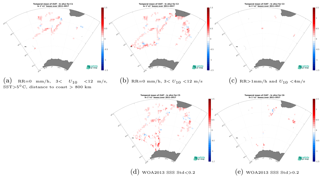
Figure 12: Temporal mean gridded over spatial boxes of size 1^\circ \times 1^\circ of \Delta SSS (SMAP SSS L4 OI v2 - Monthly (IPRC) - TSG (NCEI-0170743)) for 5 different subdatasets corresponding to:RR=0 mm/h, 3 < U_{10} < 12 m/s, SST >5^\circ\text{C} , distance to coast > 800 km (a), RR=0 mm/h, 3 < U_{10} < 12 m/s (b), RR >1 mm/h and U_{10} < 4 m/s (c), WOA2013 SSS Std <0.2 (d), WOA2013 SSS Std >0.2 (e).
