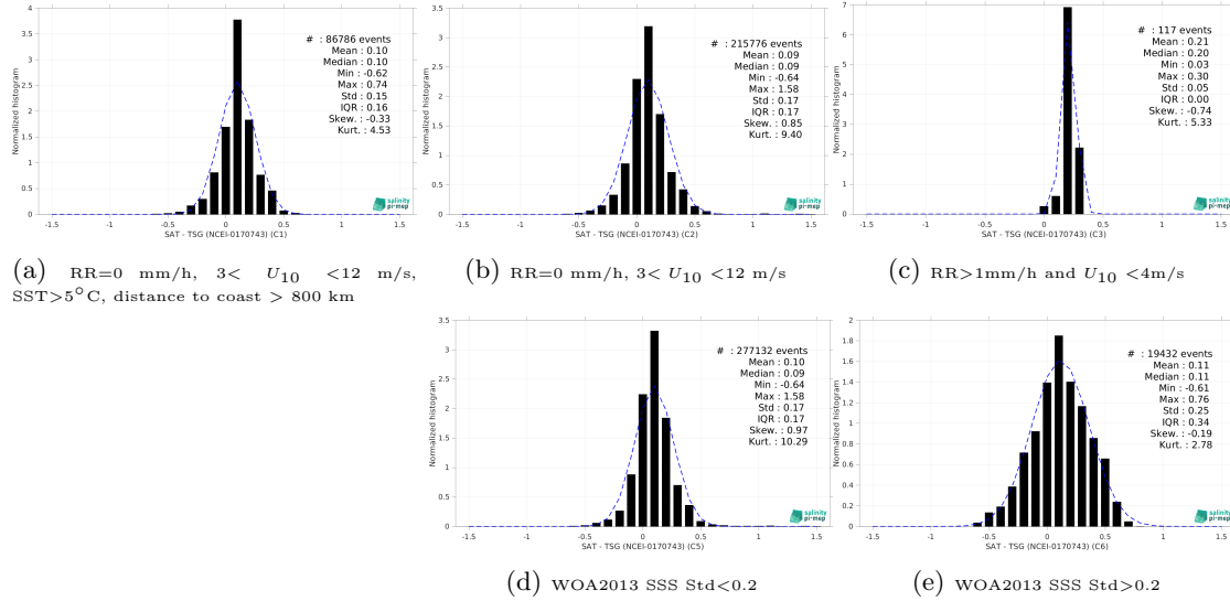
Figure 13: Normalized histogram of \Delta SSS (SMAP SSS L4 OI v2 - Monthly (IPRC) - TSG (NCEI-0170743)) for 5 different subdatasets corresponding to: RR=0 mm/h, 3 < U_{10} < 12 m/s, SST>5°C, distance to coast > 800 km (a), RR=0 mm/h, 3 < U_{10} < 12 m/s (b), RR>1mm/h and U_{10} < 4 m/s (c), WOA2013 SSS Std<0.2 (d), WOA2013 SSS Std>0.2 (e).
