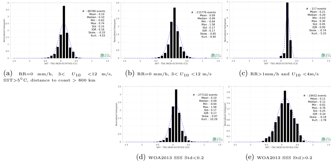
Figure 13: Normalized histogram of \Delta SSS (SMAP SSS L4 OI v2 - Monthly (IPRC) - TSG (NCEI-0170743)) for 5 different subdatasets corresponding to: RR=0 mm/h, 3 < U_{10} < 12 m/s, SST > 5°C, distance to coast > 800 km (a), RR=0 mm/h, 3 < U_{10} < 12 m/s (b), RR > 1mm/h and U_{10} < 4 m/s (c), WOA2013 SSS Std < 0.2 (d), WOA2013 SSS Std > 0.2 (e).
