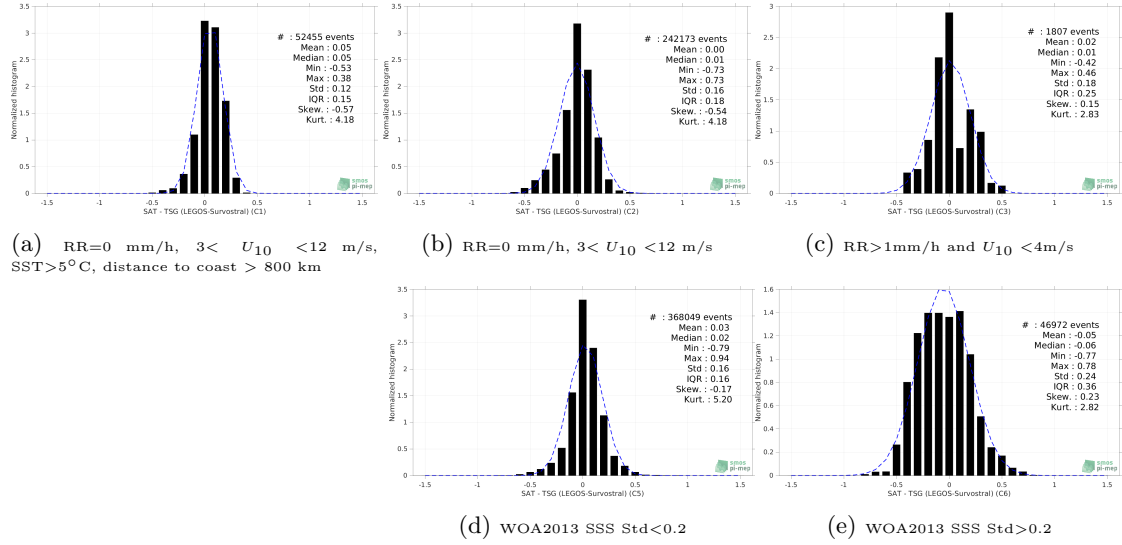
Figure 13: Normalized histogram of \Delta SSS (SMAP SSS L4 OI v2 - Monthly (IPRC) - TSG (LEGOS-Survostral)) for 5 different subdatasets corresponding to: RR=0 mm/h, 3 < U_{10} < 12 m/s, SST>5°C, distance to coast > 800 km (a), RR=0 mm/h, 3 < U_{10} < 12 m/s (b), RR>1mm/h and U_{10} < 4 m/s (c), WOA2013 SSS Std<0.2 (d), WOA2013 SSS Std>0.2 (e).
