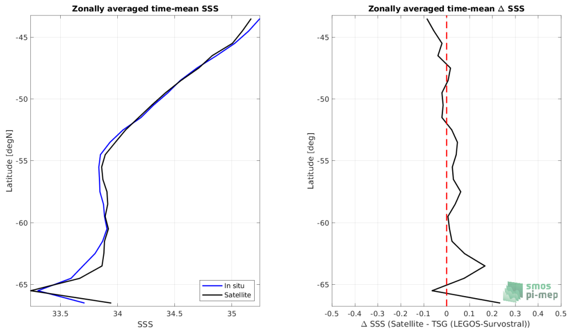
Figure 8: Left panel: Zonal mean SSS from SMAP SSS L4 OI v2 - Monthly (IPRC) satellite product (black) and from TSG (LEGOS-Survostral) (blue). Right panel: Zonal mean of \Delta SSS (Satellite - TSG (LEGOS-Survostral)) for all the collected Pi-MEP match-up pairs estimated over the full satellite product period.
