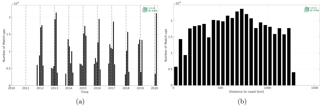
Figure 1: Number of match-ups between TSG (LEGOS-Survostral) and SMAP SSS L4 OI v2 - Monthly (IPRC) SSS as a function of time (a) and as function of the distance to coast (b) over the Global Ocean Pi-MEP region and for the full satellite product period.
