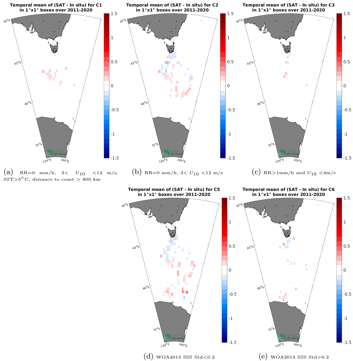
Figure 12: Temporal mean gridded over spatial boxes of size 1^\circ \times 1^\circ of \Delta SSS (SMAP SSS L4 OI v2 - Monthly (IPRC) - TSG (LEGOS-Survostral)) for 5 different subdatasets corresponding to: RR=0 mm/h, 3 < U_{10} < 12 m/s, SST>5°C, distance to coast > 800 km (a), RR=0 mm/h, 3 < U_{10} < 12 m/s (b), RR>1mm/h and U_{10} < 4 m/s (c), WOA2013 SSS Std<0.2 (d), WOA2013 SSS Std>0.2 (e).
