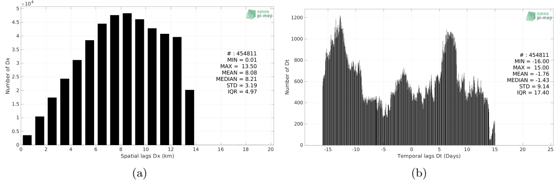
Figure 5: Histograms of the spatial (a) and temporal (b) lags between the location/time of the TSG (LEGOS-Survostral) measurement and the date of the corresponding SMAP SSS L4 OI v2 - Monthly (IPRC) SSS pixel.
