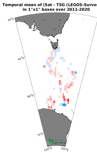
(e) MEAN( \Delta SSS) (Satellite - TSG (LEGOS-Survostral))
