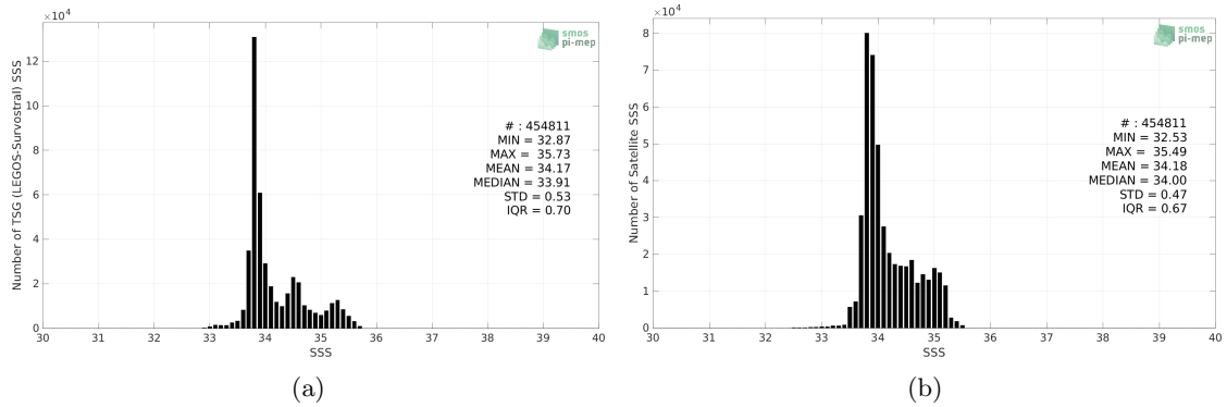
Figure 2: Histograms of SSS from TSG (LEGOS-Survostral) (a) and SMAP SSS L4 OI v2 - Monthly (IPRC) (b) considering all match-up pairs per bins of 0.1 over the Global Ocean Pi-MEP region and for the full satellite product period.
