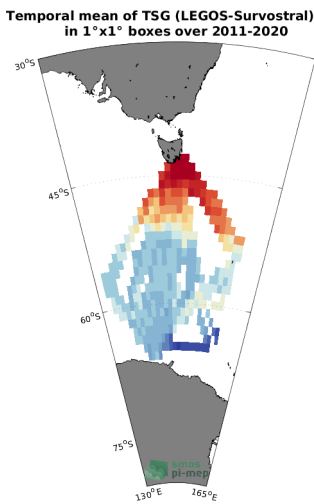
(c) MEAN(TSG (LEGOS-Survostral) SSS)
