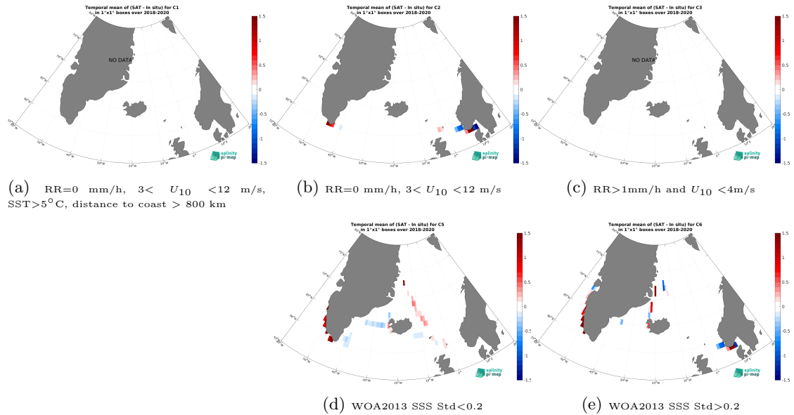
Figure 12: Temporal mean gridded over spatial boxes of size 1^{\circ}\times 1^{\circ} of \Delta\text{SSS} (SMAP SSS L4 OI v2 - Monthly (IPRC) - TSG (Lauge-Koch)) for 5 different subdatasets corresponding to:RR=0 mm/h, 3 < U_{10} < 12 m/s, SST >5^{\circ}\text{C} , distance to coast > 800 km (a), RR=0 mm/h, 3 < U_{10} < 12 m/s (b), RR >1 mm/h and U_{10} < 4 m/s (c), WOA2013 SSS Std <0.2 (d), WOA2013 SSS Std >0.2 (e).
