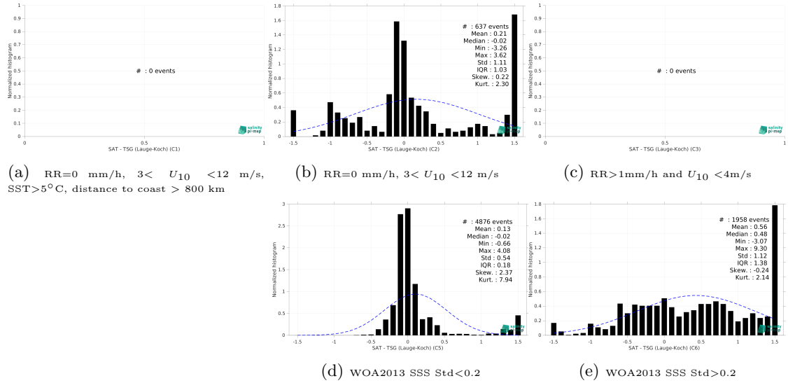
Figure 13: Normalized histogram of \Delta SSS (SMAP SSS L4 OI v2 - Monthly (IPRC) - TSG (Lauge-Koch)) for 5 different subdatasets corresponding to: RR=0 mm/h, 3 < U_{10} < 12 m/s, SST > 5°C, distance to coast > 800 km (a), RR=0 mm/h, 3 < U_{10} < 12 m/s (b), RR > 1mm/h and U_{10} < 4 m/s (c), WOA2013 SSS Std < 0.2 (d), WOA2013 SSS Std > 0.2 (e).
