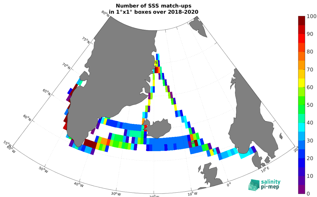
Figure 4: Number of SSS match-ups between TSG (Lauge-Koch) SSS and the SMAP SSS L4 OI v2 - Monthly (IPRC) SSS product for the Global Ocean Pi-MEP region over 1^\circ \times 1^\circ boxes and for the full satellite product period.
