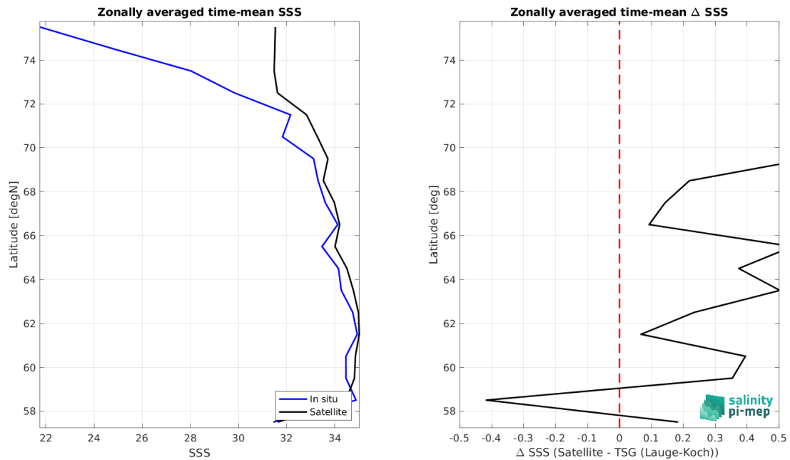
Figure 8: Left panel: Zonal mean SSS from SMAP SSS L4 OI v2 - Monthly (IPRC) satellite product (black) and from TSG (Lauge-Koch) (blue). Right panel: Zonal mean of \Delta SSS (Satellite - TSG (Lauge-Koch)) for all the collected Pi-MEP match-up pairs estimated over the full satellite product period.
