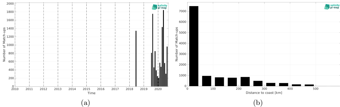
Figure 1: Number of match-ups between TSG (Lauge-Koch) and SMAP SSS L4 OI v2 - Monthly (IPRC) SSS as a function of time (a) and as function of the distance to coast (b) over the Global Ocean Pi-MEP region and for the full satellite product period.
