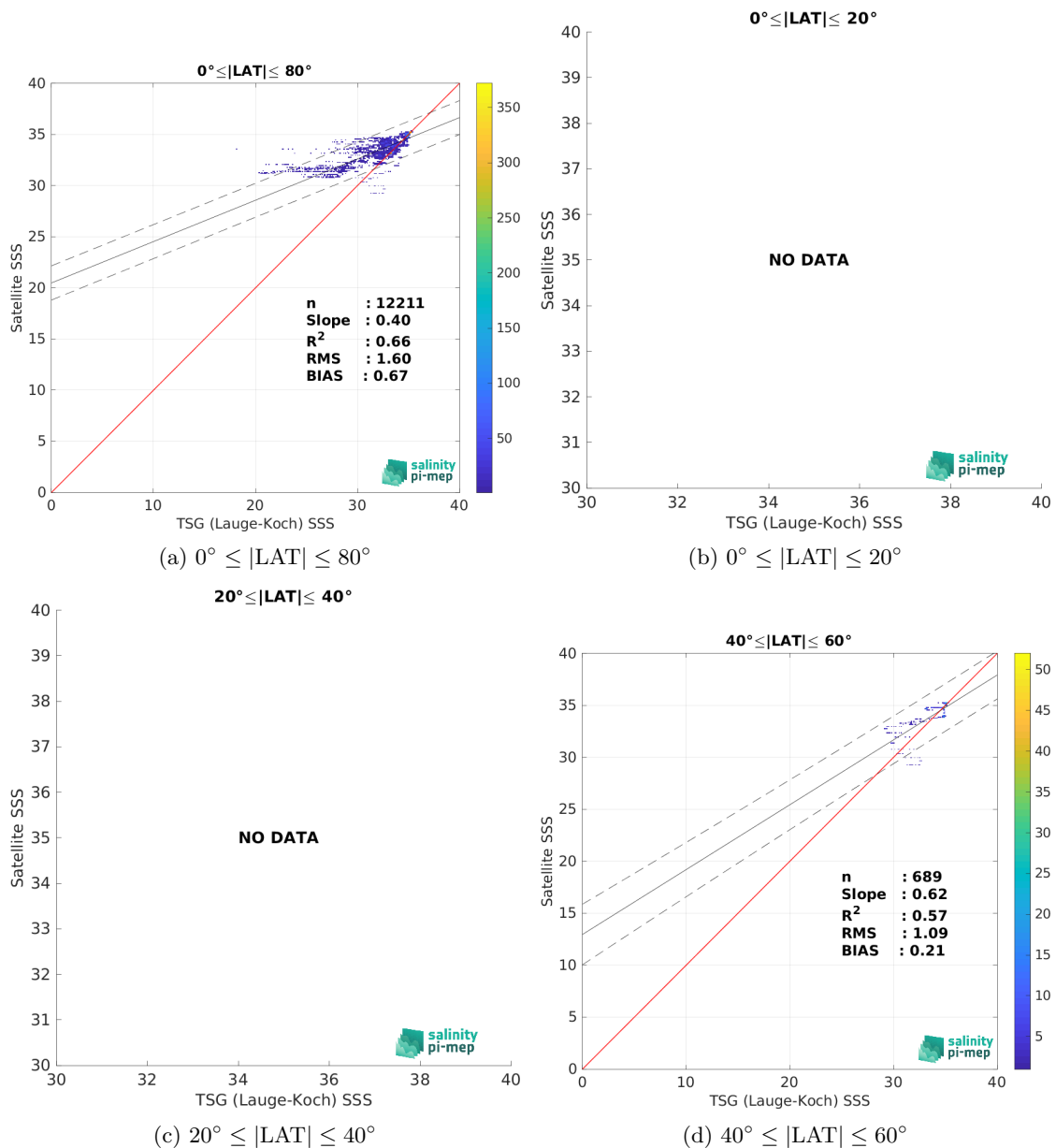
Figure 9: Contour maps of the concentration of SMAP SSS L4 OI v2 - Monthly (IPRC) SSS (y-axis) versus TSG (Lauge-Koch) SSS (x-axis) at match-up pairs for different latitude bands. For each plot, the red line shows x=y . The black thin and dashed lines indicate a linear fit through the data cloud and the \pm 95\% confidence levels, respectively. The number match-up pairs n , the slope and R^2 coefficient of the linear fit, the root mean square (RMS) and the mean bias between satellite and in situ data are indicated for each latitude band in each plots.
