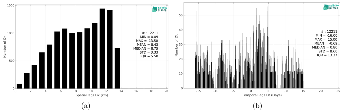
Figure 5: Histograms of the spatial (a) and temporal (b) lags between the location/time of the TSG (Lauge-Koch) measurement and the date of the corresponding SMAP SSS L4 OI v2 - Monthly (IPRC) SSS pixel.
