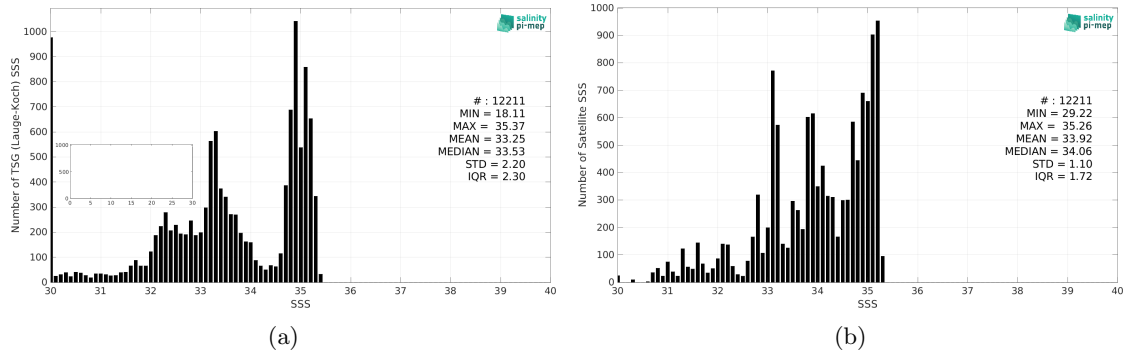
Figure 2: Histograms of SSS from TSG (Lauge-Koch) (a) and SMAP SSS L4 OI v2 - Monthly (IPRC) (b) considering all match-up pairs per bins of 0.1 over the Global Ocean Pi-MEP region and for the full satellite product period.
