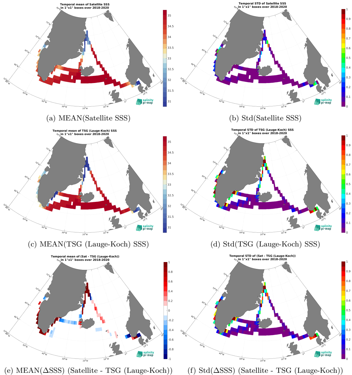
Figure 6: Temporal mean (left) and Std (right) of SSS from SMAP SSS L4 OI v2 - Monthly (IPRC) (top), TSG (Lauge-Koch) (middle), and of \Delta SSS (Satellite - TSG (Lauge-Koch)). Only match-up pairs are used to generate these maps.
