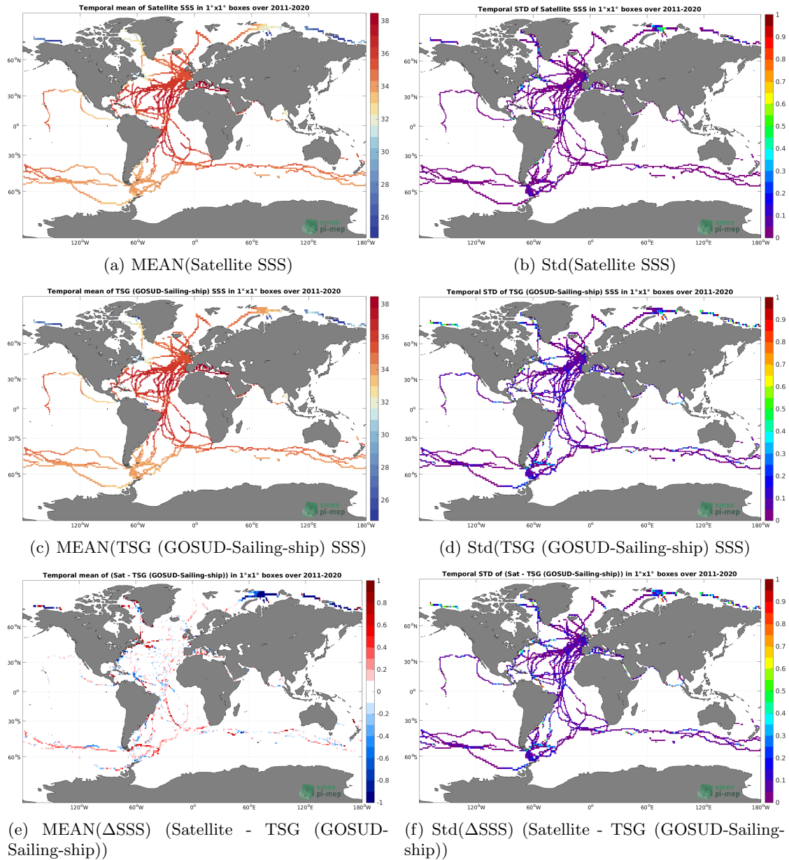
Figure 6: Temporal mean (left) and Std (right) of SSS from SMAP SSS L4 OI v2 - Monthly (IPRC) (top), TSG (GOSUD-Sailing-ship) (middle), and of \Delta SSS (Satellite - TSG (GOSUD-Sailing-ship)). Only match-up pairs are used to generate these maps.
