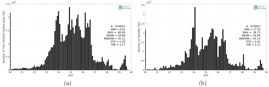
Figure 2: Histograms of SSS from TSG (GOSUD-Sailing-ship) (a) and SMAP SSS L4 OI v2 - Monthly (IPRC) (b) considering all match-up pairs per bins of 0.1 over the Global Ocean Pi-MEP region and for the full satellite product period.
