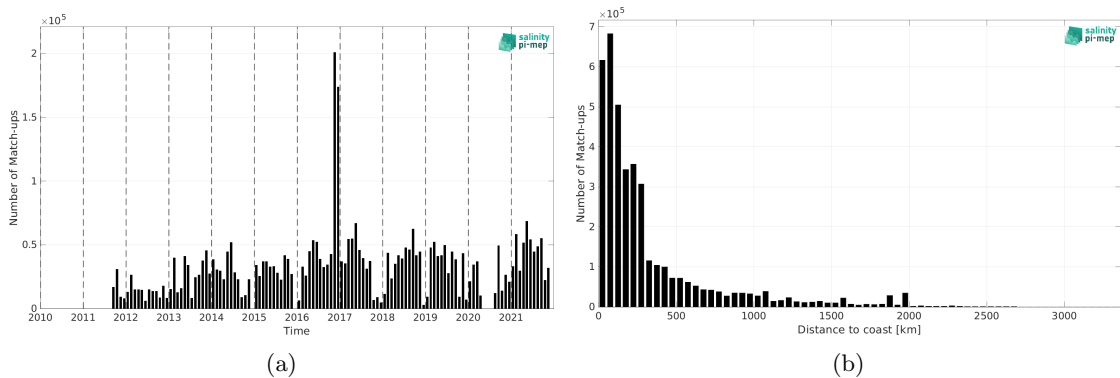
Figure 1: Number of match-ups between TSG (GOSUD-Research-vessel) and SMAP SSS L4 OI v2 - Monthly (IPRC) SSS as a function of time (a) and as function of the distance to coast (b) over the Global Ocean Pi-MEP region and for the full satellite product period.
