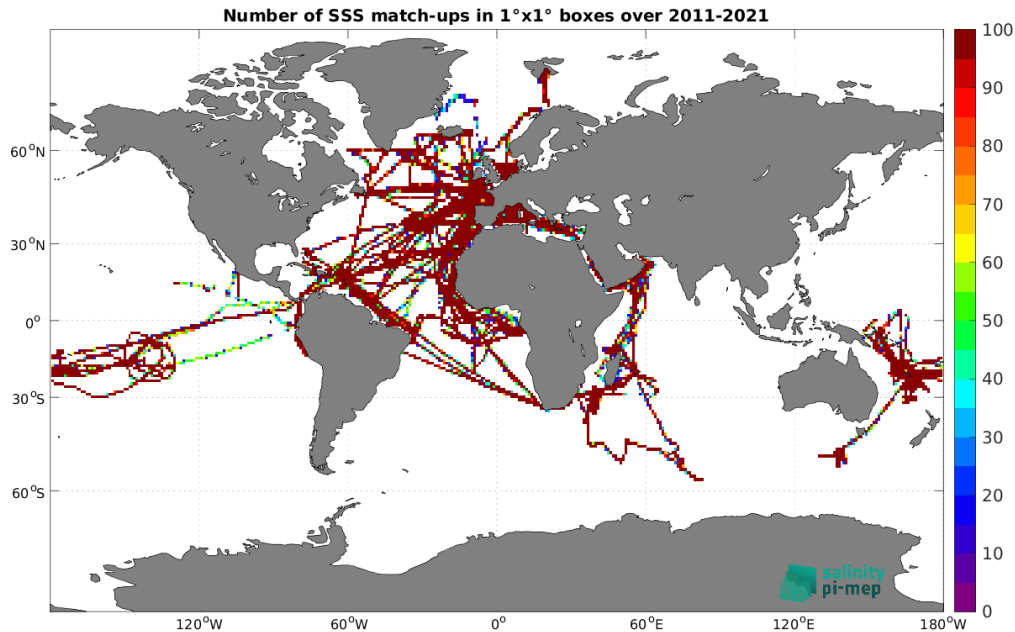
Figure 4: Number of SSS match-ups between TSG (GOSUD-Research-vessel) SSS and the SMAP SSS L4 OI v2 - Monthly (IPRC) SSS product for the Global Ocean Pi-MEP region over 1^\circ \times 1^\circ boxes and for the full satellite product period.
