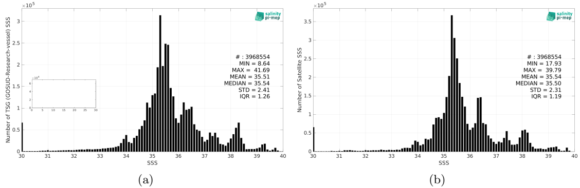
Figure 2: Histograms of SSS from TSG (GOSUD-Research-vessel) (a) and SMAP SSS L4 OI v2 - Monthly (IPRC) (b) considering all match-up pairs per bins of 0.1 over the Global Ocean Pi-MEP region and for the full satellite product period.
