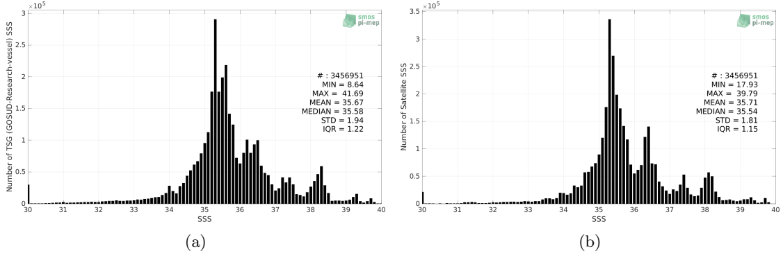
Figure 2: Histograms of SSS from TSG (GOSUD-Research-vessel) (a) and SMAP SSS L4 OI v2 - Monthly (IPRC) (b) considering all match-up pairs per bins of 0.1 over the Global Ocean Pi-MEP region and for the full satellite product period.
