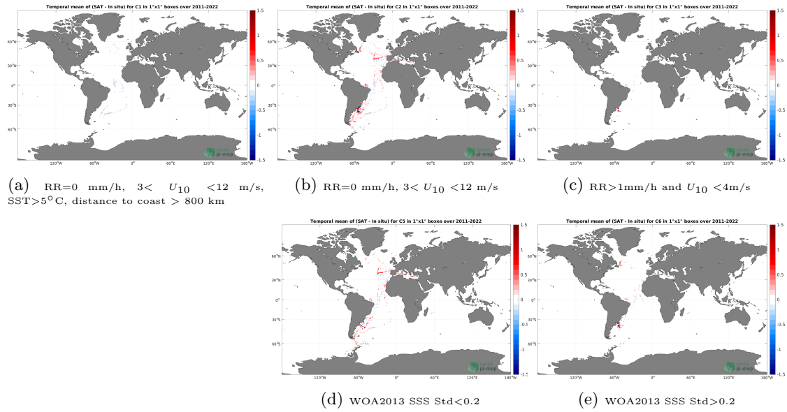
Figure 12: Temporal mean gridded over spatial boxes of size 1^\circ \times 1^\circ of \Delta SSS (SMAP SSS L4 OI v2 - Monthly (IPRC) - TSG (CSIC-UTM)) for 5 different subdatasets corresponding to:RR=0 mm/h, 3 < U_{10} < 12 m/s, SST >5^\circ C, distance to coast > 800 km (a), RR=0 mm/h, 3 < U_{10} < 12 m/s (b), RR >1 mm/h and U_{10} < 4 m/s (c), WOA2013 SSS Std <0.2 (d), WOA2013 SSS Std >0.2 (e).
