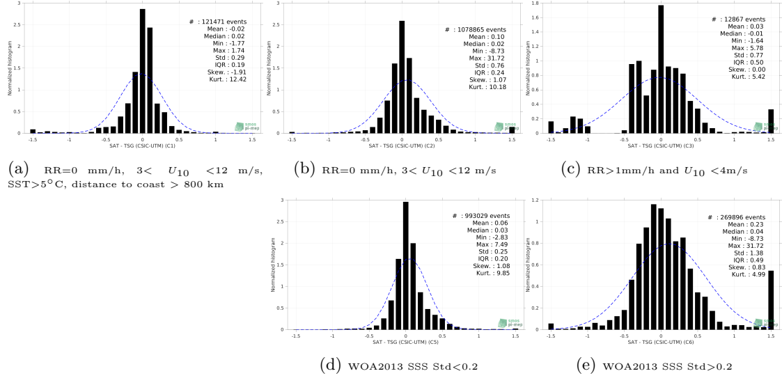
Figure 13: Normalized histogram of \Delta SSS (SMAP SSS L4 OI v2 - Monthly (IPRC) - TSG (CSIC-UTM)) for 5 different subdatasets corresponding to: RR=0 mm/h, 3 < U_{10} < 12 m/s, SST>5°C, distance to coast > 800 km (a), RR=0 mm/h, 3 < U_{10} < 12 m/s (b), RR>1mm/h and U_{10} < 4 m/s (c), WOA2013 SSS Std<0.2 (d), WOA2013 SSS Std>0.2 (e).
