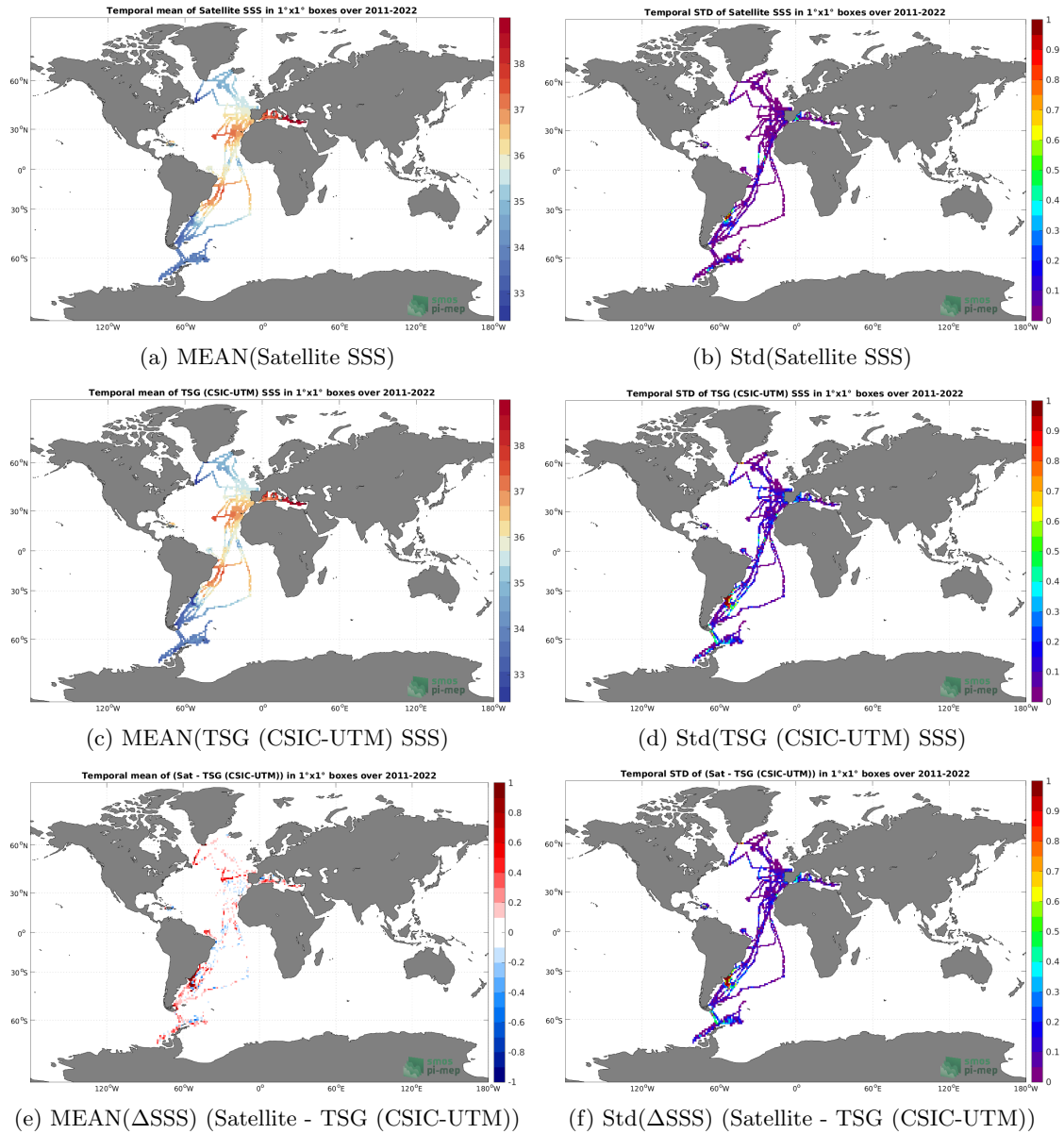
Figure 6: Temporal mean (left) and Std (right) of SSS from SMAP SSS L4 OI v2 - Monthly (IPRC) (top), TSG (CSIC-UTM) (middle), and of \Delta SSS (Satellite - TSG (CSIC-UTM)). Only match-up pairs are used to generate these maps.
