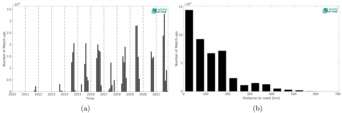
Figure 1: Number of match-ups between TSG (Amundsen) and SMAP SSS L4 OI v2 - Monthly (IPRC) SSS as a function of time (a) and as function of the distance to coast (b) over the Global Ocean Pi-MEP region and for the full satellite product period.
