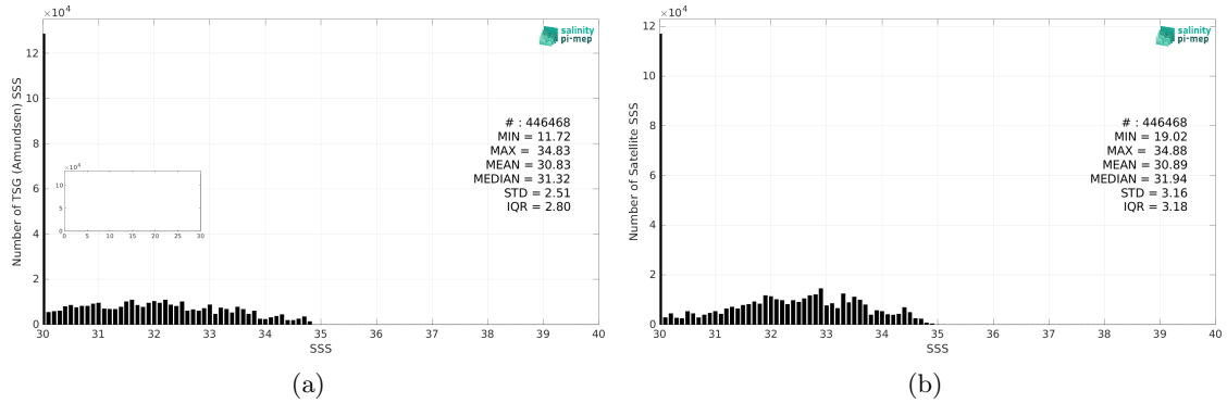
Figure 2: Histograms of SSS from TSG (Amundsen) (a) and SMAP SSS L4 OI v2 - Monthly (IPRC) (b) considering all match-up pairs per bins of 0.1 over the Global Ocean Pi-MEP region and for the full satellite product period.
