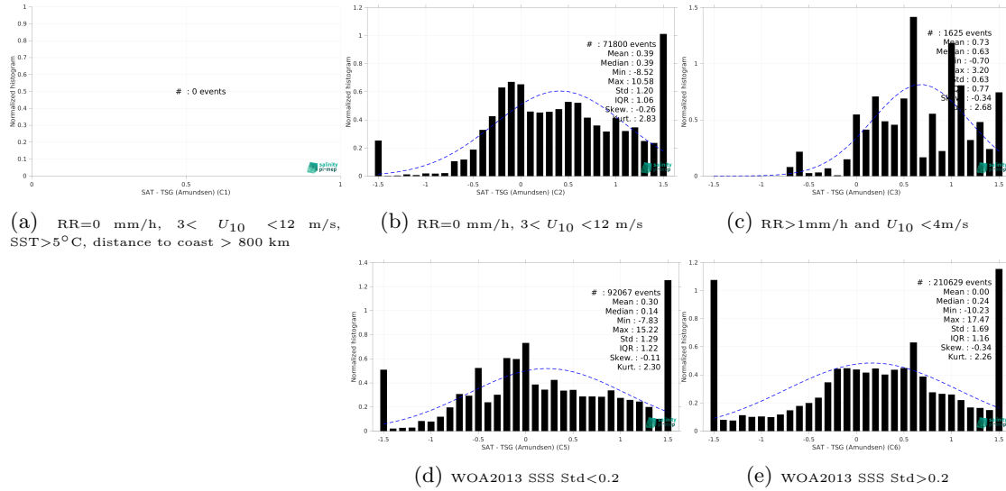
Figure 13: Normalized histogram of \Delta SSS (SMAP SSS L4 OI v2 - Monthly (IPRC) - TSG (Amundsen)) for 5 different subdatasets corresponding to: RR=0 mm/h, 3 < U_{10} < 12 m/s, SST > 5°C, distance to coast > 800 km (a), RR=0 mm/h, 3 < U_{10} < 12 m/s (b), RR > 1mm/h and U_{10} < 4 m/s (c), WOA2013 SSS Std < 0.2 (d), WOA2013 SSS Std > 0.2 (e).
