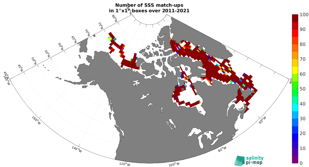
Figure 4: Number of SSS match-ups between TSG (Amundsen) SSS and the SMAP SSS L4 OI v2 - Monthly (IPRC) SSS product for the Global Ocean Pi-MEP region over 1^\circ \times 1^\circ boxes and for the full satellite product period.
