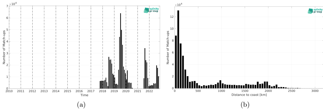
Figure 1: Number of match-ups between Saildrone and SMAP SSS L4 OI v2 - Monthly (IPRC) SSS as a function of time (a) and as function of the distance to coast (b) over the Global Ocean Pi-MEP region and for the full satellite product period.
