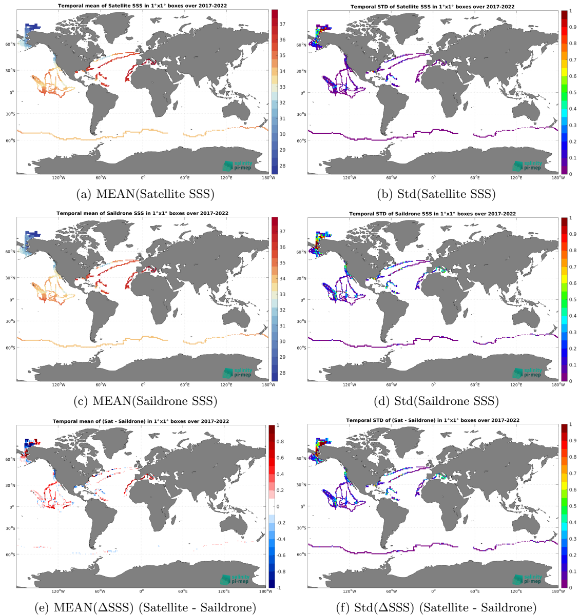
Figure 6: Temporal mean (left) and Std (right) of SSS from SMAP SSS L4 OI v2 - Monthly (IPRC) (top), Saildrone (middle), and of \Delta SSS (Satellite - Saildrone ). Only match-up pairs are used to generate these maps.
