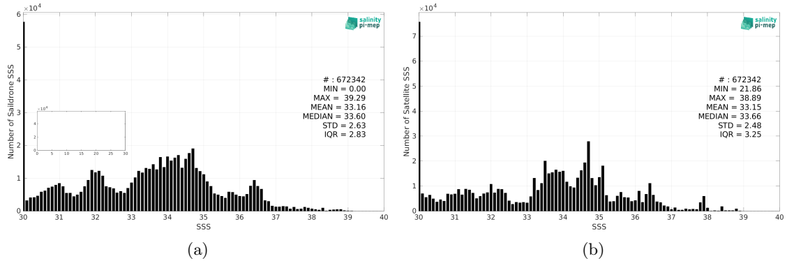
Figure 2: Histograms of SSS from Saildrone (a) and SMAP SSS L4 OI v2 - Monthly (IPRC) (b) considering all match-up pairs per bins of 0.1 over the Global Ocean Pi-MEP region and for the full satellite product period.
