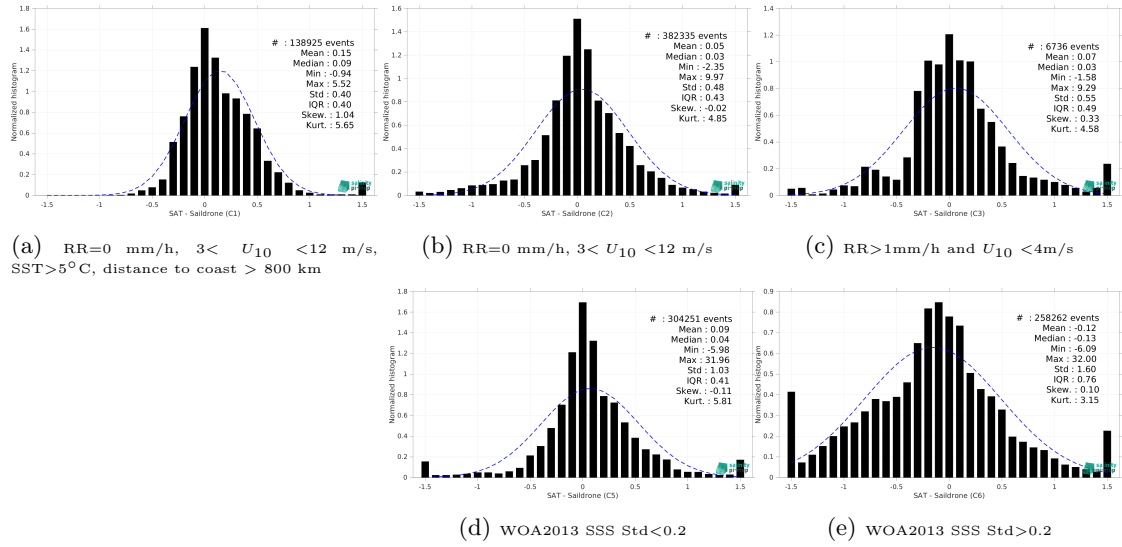
Figure 13: Normalized histogram of \Delta SSS (SMAP SSS L4 OI v2 - Monthly (IPRC) - Sairdron) for 5 different subdatasets corresponding to: RR=0 mm/h, 3 < U_{10} < 12 m/s, SST > 5°C, distance to coast > 800 km (a), RR=0 mm/h, 3 < U_{10} < 12 m/s (b), RR > 1mm/h and U_{10} < 4 m/s (c), WOA2013 SSS Std < 0.2 (d), WOA2013 SSS Std > 0.2 (e).
