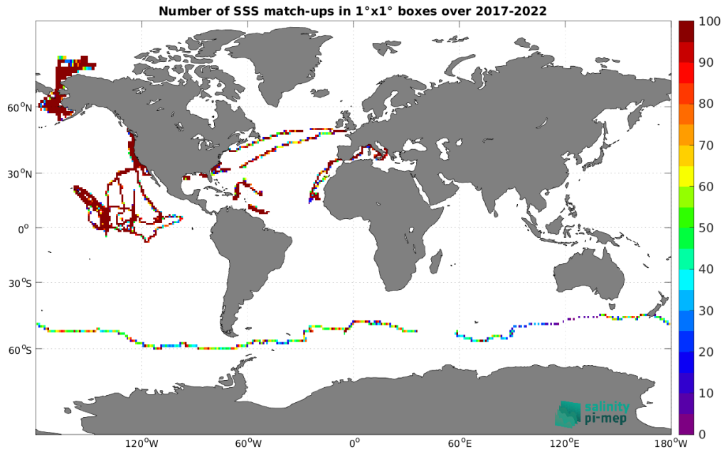
Figure 4: Number of SSS match-ups between Saildrone SSS and the SMAP SSS L4 OI v2 - Monthly (IPRC) SSS product for the Global Ocean Pi-MEP region over 1^\circ \times 1^\circ boxes and for the full satellite product period.
