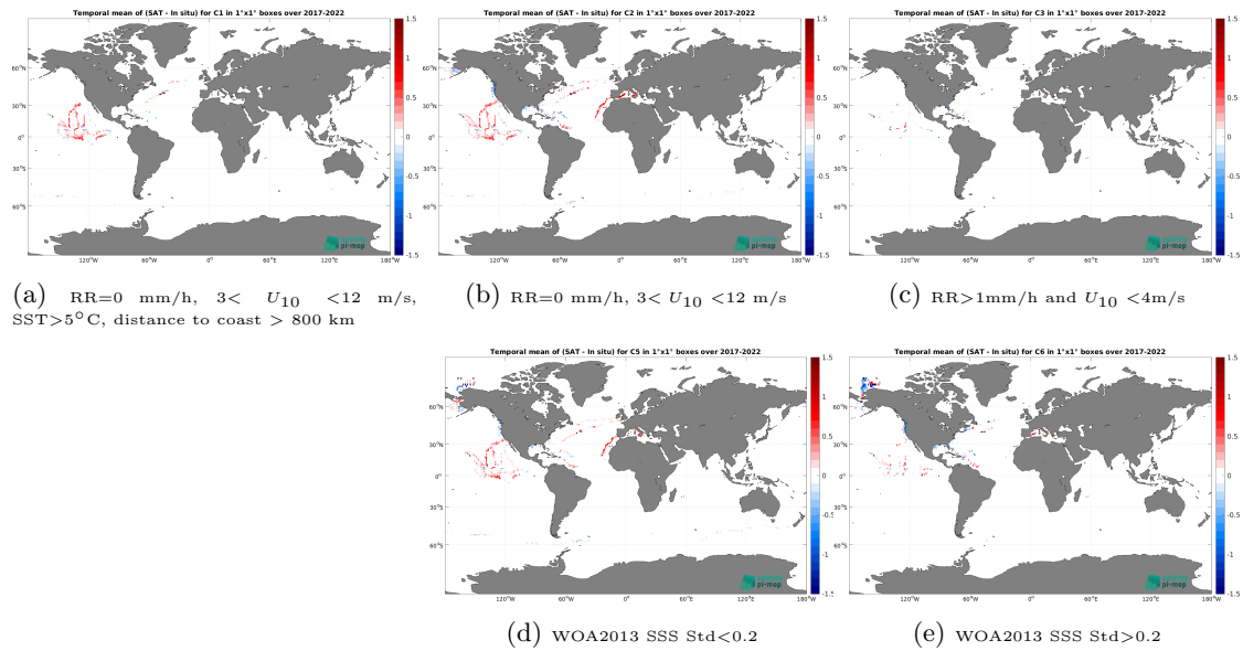
Figure 12: Temporal mean gridded over spatial boxes of size 1^\circ \times 1^\circ of \Delta SSS (SMAP SSS L4 OI v2 - Monthly (IPRC) - Saildrone) for 5 different subdatasets corresponding to:RR=0 mm/h, 3 < U_{10} < 12 m/s, SST >5^\circ\text{C} , distance to coast > 800 km (a), RR=0 mm/h, 3 < U_{10} < 12 m/s (b), RR >1 mm/h and U_{10} < 4 m/s (c), WOA2013 SSS Std <0.2 (d), WOA2013 SSS Std >0.2 (e).
