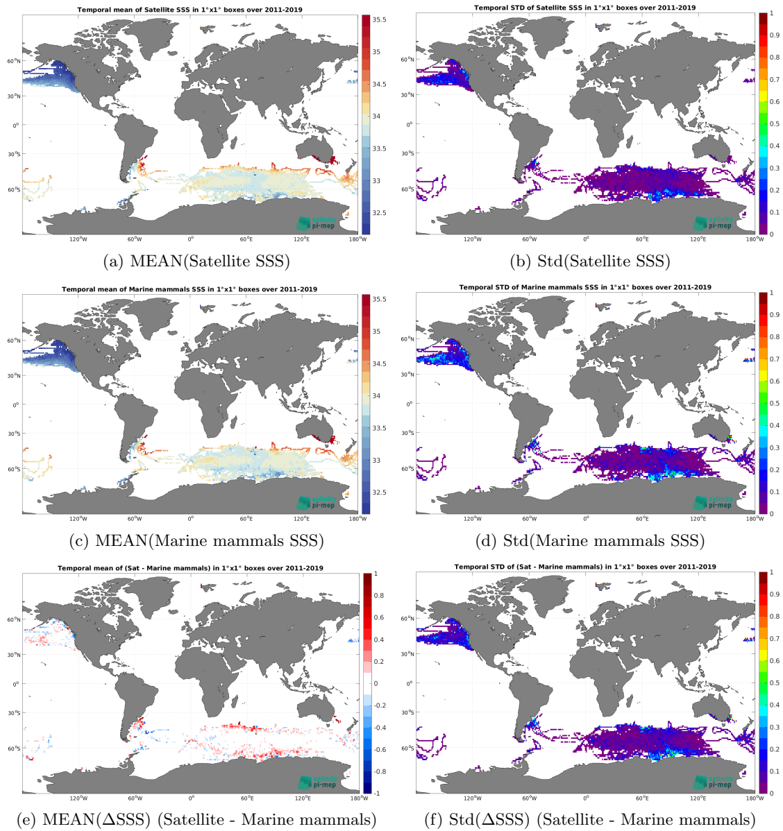
Figure 6: Temporal mean (left) and Std (right) of SSS from SMAP SSS L4 OI v2 - Monthly (IPRC) (top), Marine mammals (middle), and of \Delta SSS (Satellite - Marine mammals). Only match-up pairs are used to generate these maps.
