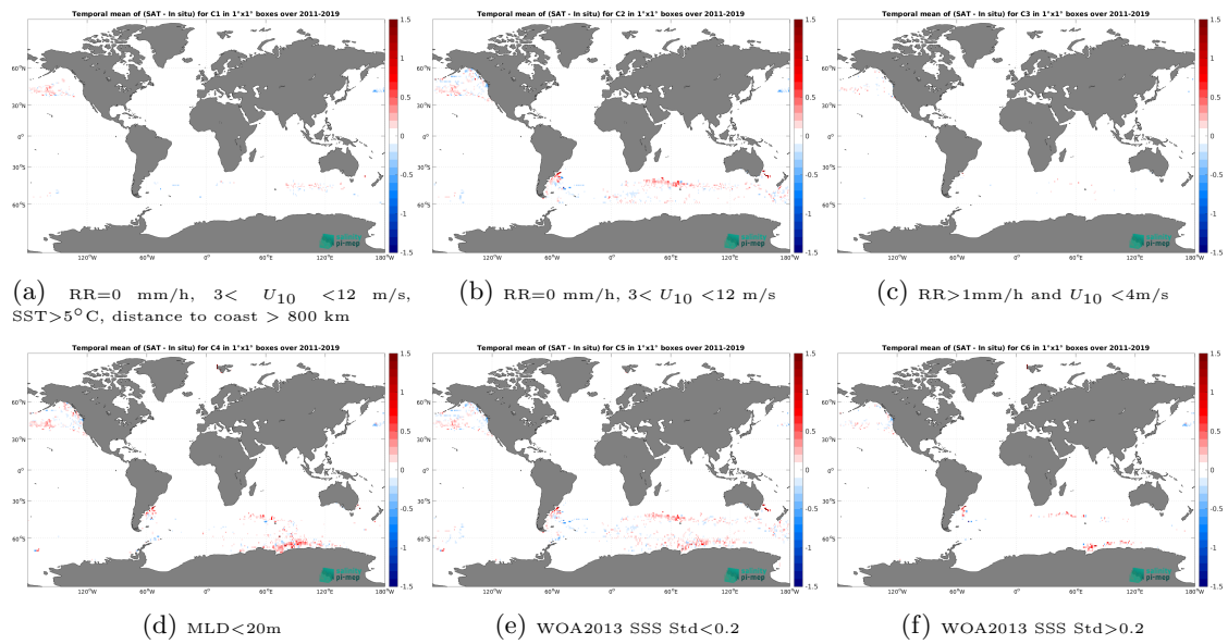
Figure 12: Temporal mean gridded over spatial boxes of size 1^\circ \times 1^\circ of \Delta SSS (SMAP SSS L4 OI v2 - Monthly (IPRC) - Marine mammals) for 6 different subdatasets corresponding to:RR=0 mm/h, 3 < U_{10} < 12 m/s, SST >5^\circ C, distance to coast > 800 km (a), RR=0 mm/h, 3 < U_{10} < 12 m/s (b), RR >1 mm/h and U_{10} < 4 m/s (c),MLD <20 m (d),WOA2013 SSS Std <0.2 (e),WOA2013 SSS Std >0.2 (f).
