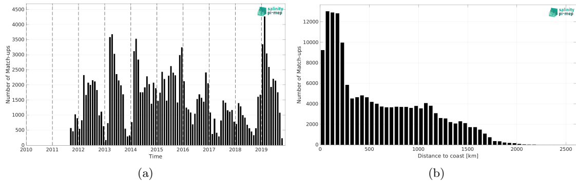
Figure 1: Number of match-ups between Marine mammals and SMAP SSS L4 OI v2 - Monthly (IPRC) SSS as a function of time (a) and as function of the distance to coast (b) over the Global Ocean Pi-MEP region and for the full satellite product period.
