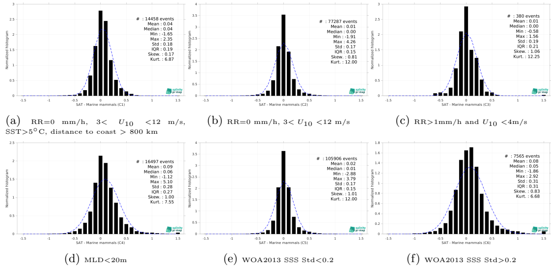
Figure 13: Normalized histogram of \Delta SSS (SMAP SSS L4 OI v2 - Monthly (IPRC) - Marine mammals) for 6 different subdatasets corresponding to: RR=0 mm/h, 3 < U_{10} < 12 m/s, SST > 5°C, distance to coast > 800 km (a), RR=0 mm/h, 3 < U_{10} < 12 m/s (b), RR > 1mm/h and U_{10} < 4 m/s (c), MLD < 20m (d), WOA2013 SSS Std < 0.2 (e), WOA2013 SSS Std > 0.2 (f).
