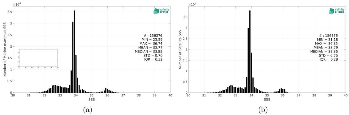
Figure 2: Histograms of SSS from Marine mammals (a) and SMAP SSS L4 OI v2 - Monthly (IPRC) (b) considering all match-up pairs per bins of 0.1 over the Global Ocean Pi-MEP region and for the full satellite product period.
