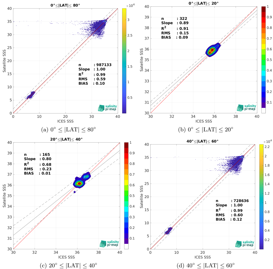
Figure 9: Contour maps of the concentration of SMAP SSS L4 OI v2 - Monthly (IPRC) SSS (y-axis) versus ICES SSS (x-axis) at match-up pairs for different latitude bands. For each plot, the red line shows x=y . The black thin and dashed lines indicate a linear fit through the data cloud and the \pm 95\% confidence levels, respectively. The number match-up pairs n , the slope and R^2 coefficient of the linear fit, the root mean square (RMS) and the mean bias between satellite and in situ data are indicated for each latitude band in each plots.
