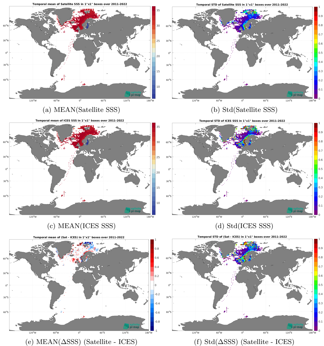
Figure 6: Temporal mean (left) and Std (right) of SSS from SMAP SSS L4 OI v2 - Monthly (IPRC) (top), ICES (middle), and of \Delta SSS (Satellite - ICES). Only match-up pairs are used to generate these maps.
