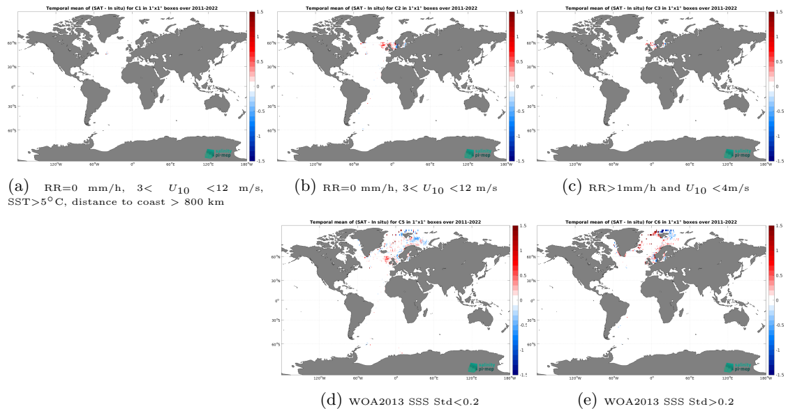
Figure 12: Temporal mean gridded over spatial boxes of size 1^\circ \times 1^\circ of \Delta SSS (SMAP SSS L4 OI v2 - Monthly (IPRC) - ICES) for 5 different subdatasets corresponding to:RR=0 mm/h, 3 < U_{10} < 12 m/s, SST > 5^\circ\text{C} , distance to coast > 800 km (a), RR=0 mm/h, 3 < U_{10} < 12 m/s (b), RR > 1 mm/h and U_{10} < 4 m/s (c), WOA2013 SSS Std < 0.2 (d), WOA2013 SSS Std > 0.2 (e).
