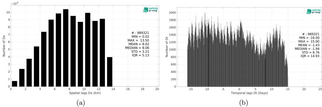
Figure 5: Histograms of the spatial (a) and temporal (b) lags between the location/time of the ICES measurement and the date of the corresponding SMAP SSS L4 OI v2 - Monthly (IPRC) SSS pixel.
