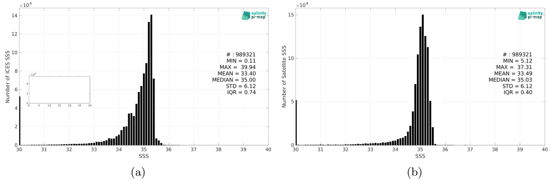
Figure 2: Histograms of SSS from ICES (a) and SMAP SSS L4 OI v2 - Monthly (IPRC) (b) considering all match-up pairs per bins of 0.1 over the Global Ocean Pi-MEP region and for the full satellite product period.
