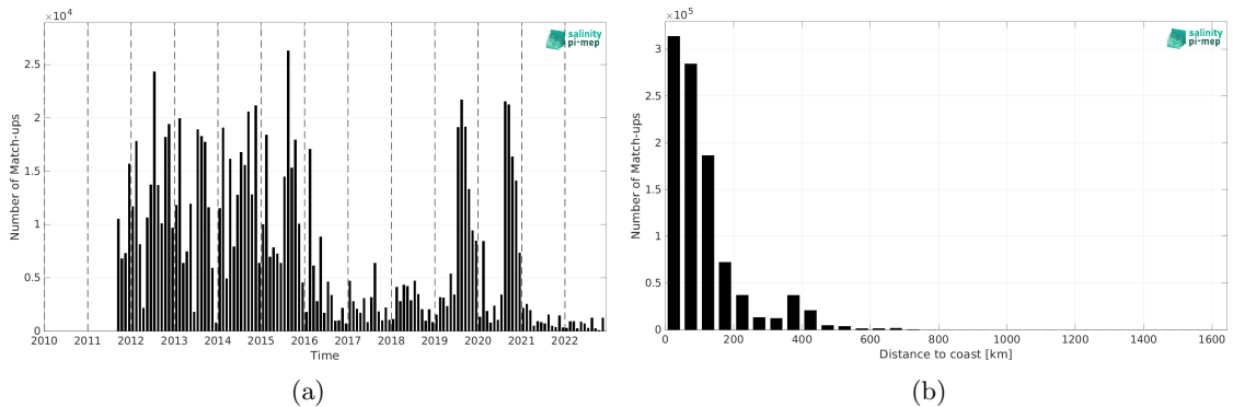
Figure 1: Number of match-ups between ICES and SMAP SSS L4 OI v2 - Monthly (IPRC) SSS as a function of time (a) and as function of the distance to coast (b) over the Global Ocean Pi-MEP region and for the full satellite product period.
