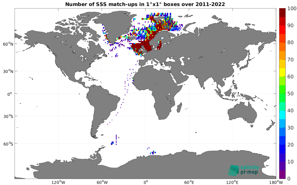
Figure 4: Number of SSS match-ups between ICES SSS and the SMAP SSS L4 OI v2 - Monthly (IPRC) SSS product for the Global Ocean Pi-MEP region over 1^\circ \times 1^\circ boxes and for the full satellite product period.
